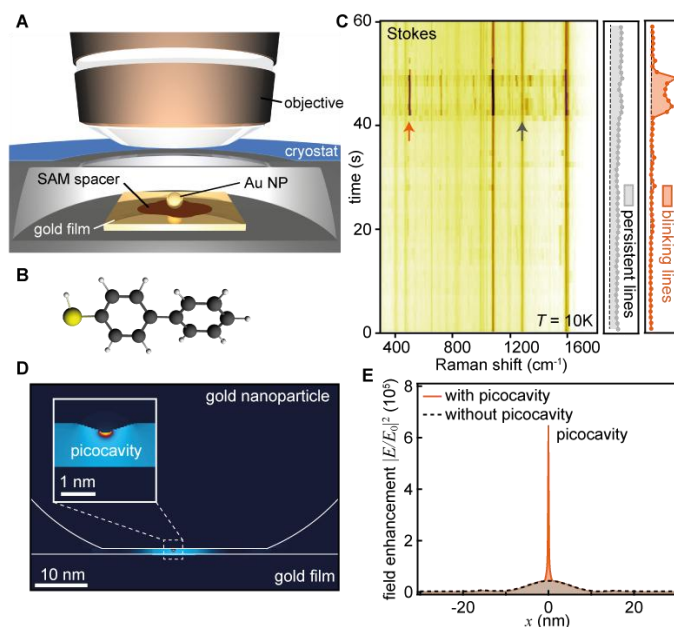
Figure 1 | Raman spectra from molecules in picocavity and near-field light distribution. (A) Schematic cooled nanoparticle-on-mirror (NPoM) geometry. (B) Biphenyl-4-thiol molecular monolayer. (C) SERS time series from a single 90nm NPoM with 60\mu\text{W}/\mu\text{m}^2 pump. (D-E) Simulations of faceted gold nanoparticle with(out) atomic protrusion at x=0 nm. (D) Near-field map, inset: enlarged view of picocavity, showing sub-nanometre localisation of optical field. (E) Near-field intensity across the gap.
