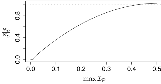
FIG. 2. Ratio of the pilot-based minimum N , N_{\mathcal{P}} , over the blind version, N_{\mathcal{B}} as a function of the rightmost point \max \mathcal{I}_{\mathcal{P}} of the pilot sample interval, with \Delta = 0.01 , \varepsilon = 0.0001 , \gamma = 0.01 , \gamma_{\mathcal{P}} = \gamma/10 . Here, N_{\mathcal{B}} = 68,311 .
