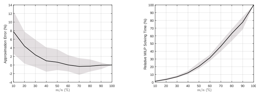
Fig. 5: Approximation errors (left panel) and runtimes (right panel) of the reduced capital budgeting problem for different reduction factors m/n . The solid lines represent the averages, while the shaded areas capture the intervals between the 10% and 90% quantiles across 100 independent simulation runs.
