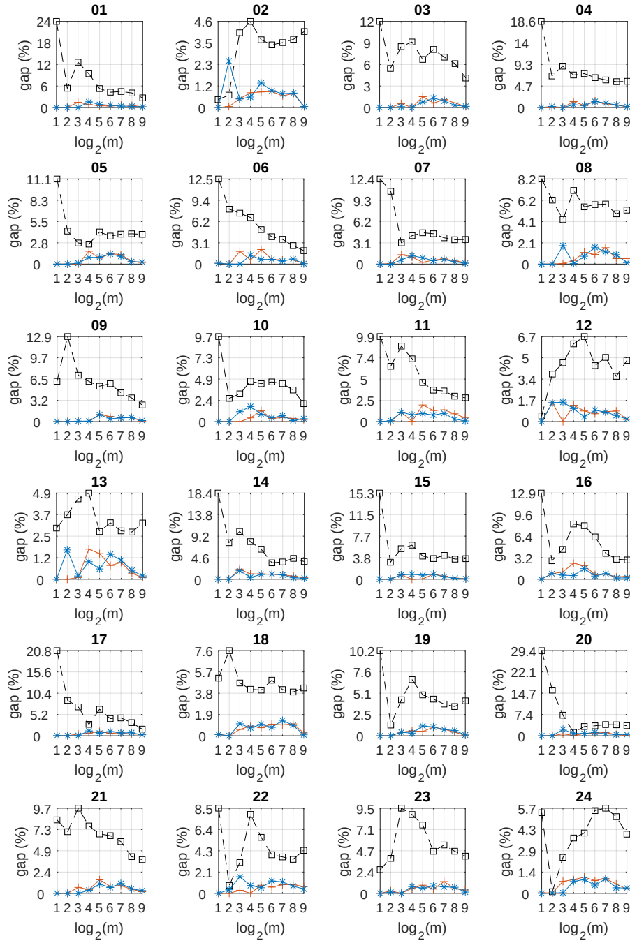
Fig. 4: Optimality gaps of DPCV (dashed lines with boxes), LOC-1 (solid lines with pluses) and LOC-2 (solid lines with stars) relative to MILP.
