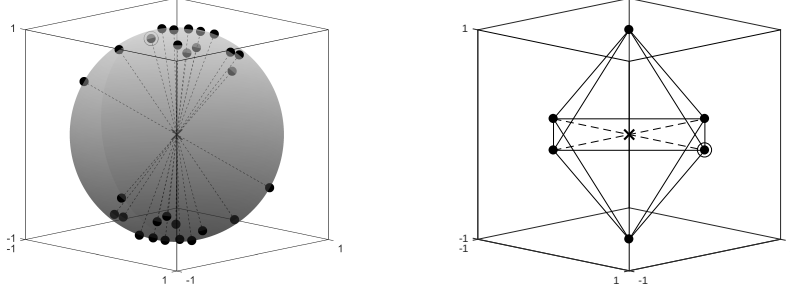
Fig. 2: Empirical distributions in \mathbb{R}^3 that maximize the ratio between D_l(\hat{\mathbb{P}}_n, 1) and C_l(\hat{\mathbb{P}}_n, 1) for l = 2 and \|\cdot\| = \|\cdot\|_2 (left panel) as well as l = 1 and \|\cdot\| = \|\cdot\|_1 (right panel). In both cases, the continuous scenario reduction problem is optimized by the Dirac distribution at \mathbf{0} (marked as \times ), whereas the discrete scenario reduction problem is optimized by any of the atoms (such as \circ ).
