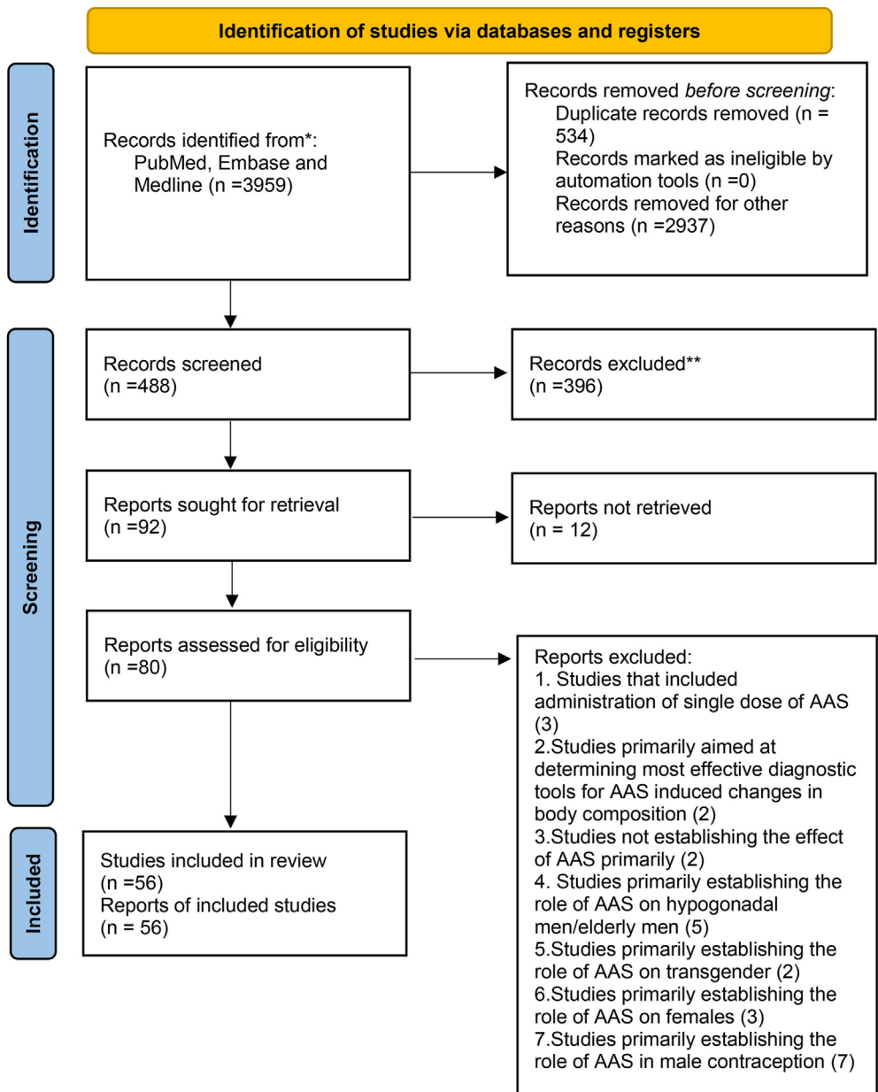
Fig. 1. PRISMA chart.
