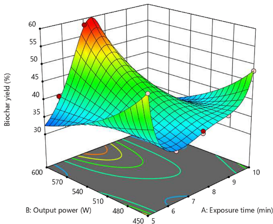
Figure 3. 3D-Surface plots of biochar yield as a function of microwave output power and exposure time.
