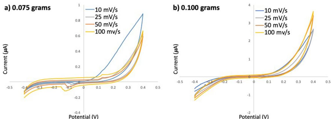
Figure 5. Cyclic voltammograms of the a) 0.075 g and b) 0.100 g biochar-electrolyte dispersion at scanning rates of 10, 25, 50, and 100 mV/s.
