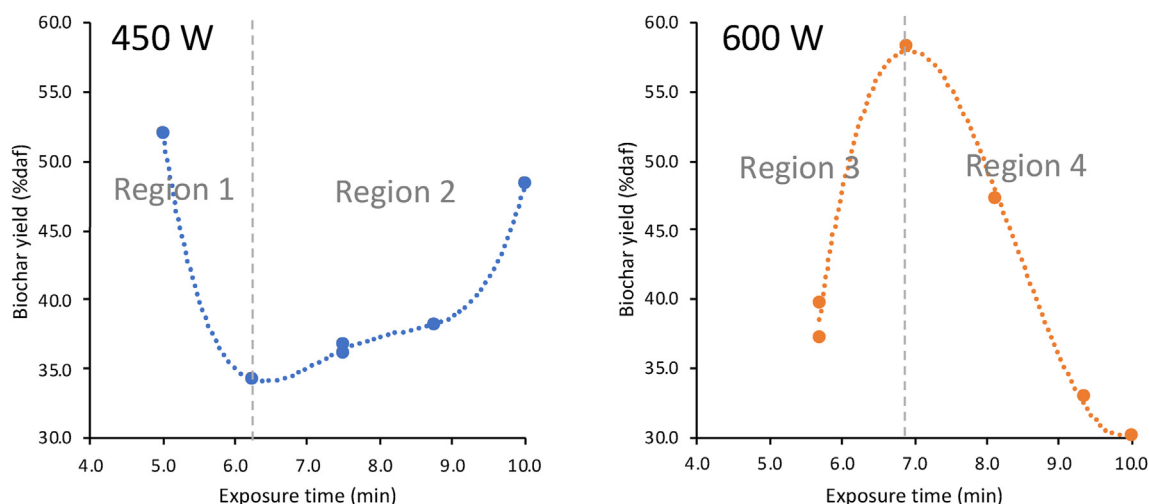
Figure 2. Effect of increasing exposure time on the biochar yield at 450 W and 600 W output power.
