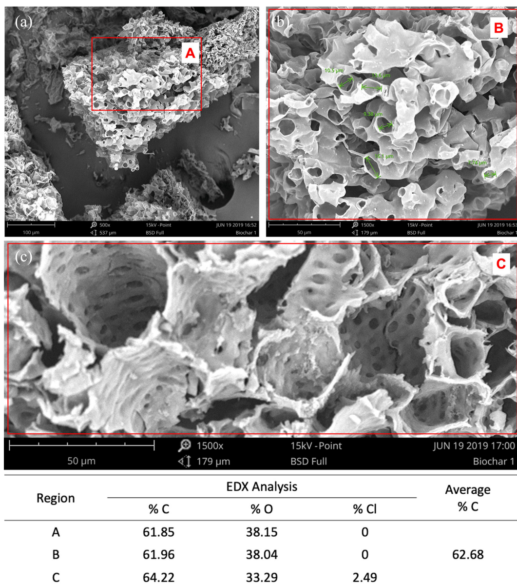
Figure 4. SEM images with EDX analysis of the optimized biochar product at different magnifications: 500x (a), 1500x (b and c). The red box enclosures (A, B, C) are the regions selected for EDX analysis.
