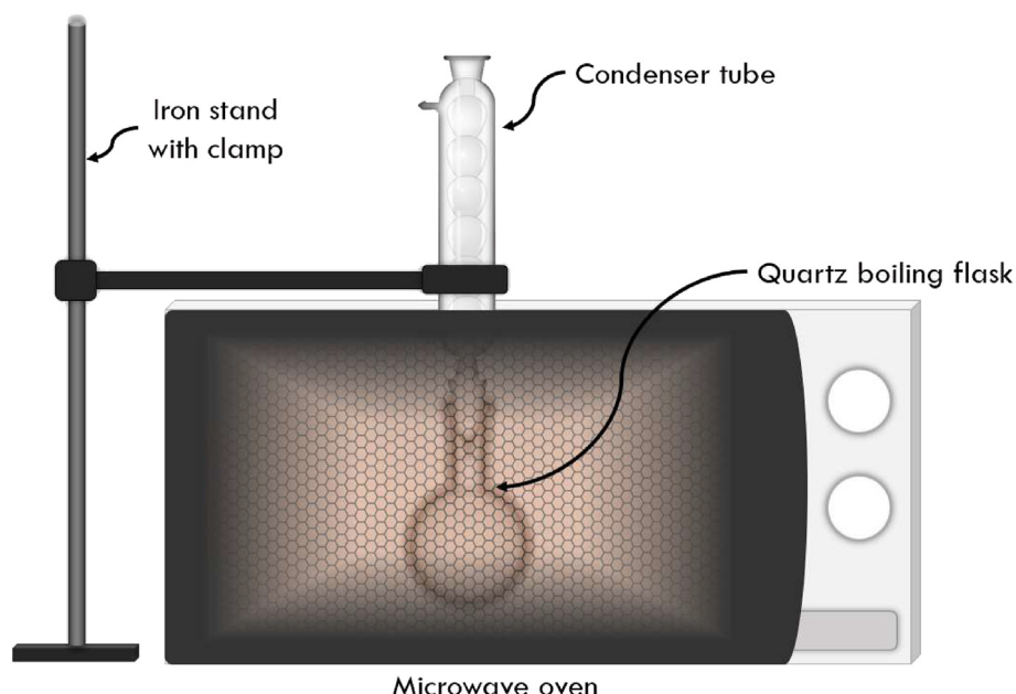
Figure 1. Experimental setup for pyrolysis experiment.
