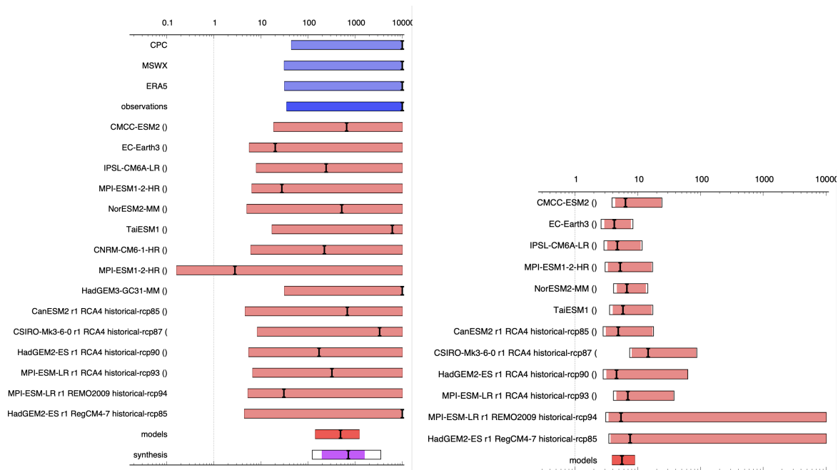
Figure 9. Synthesis of probability ratios when comparing the magnitudes of the 10-day averaged maximum temperatures over the study region between (a) the current climate and a 1.2°C cooler climate and (b) a 0.8°C warmer (2°C since pre-industrial) climate and the current climate. Note that many large values are cut off at 10000 in (a).
