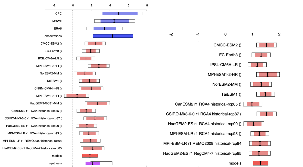
Figure 8: Synthesis of intensity changes when comparing the magnitudes of the 10-day averaged maximum temperatures over the study region between (a) the current climate and a 1.2°C cooler climate and (b) a 0.8°C warmer (2°C since pre-industrial) climate and the current climate.
