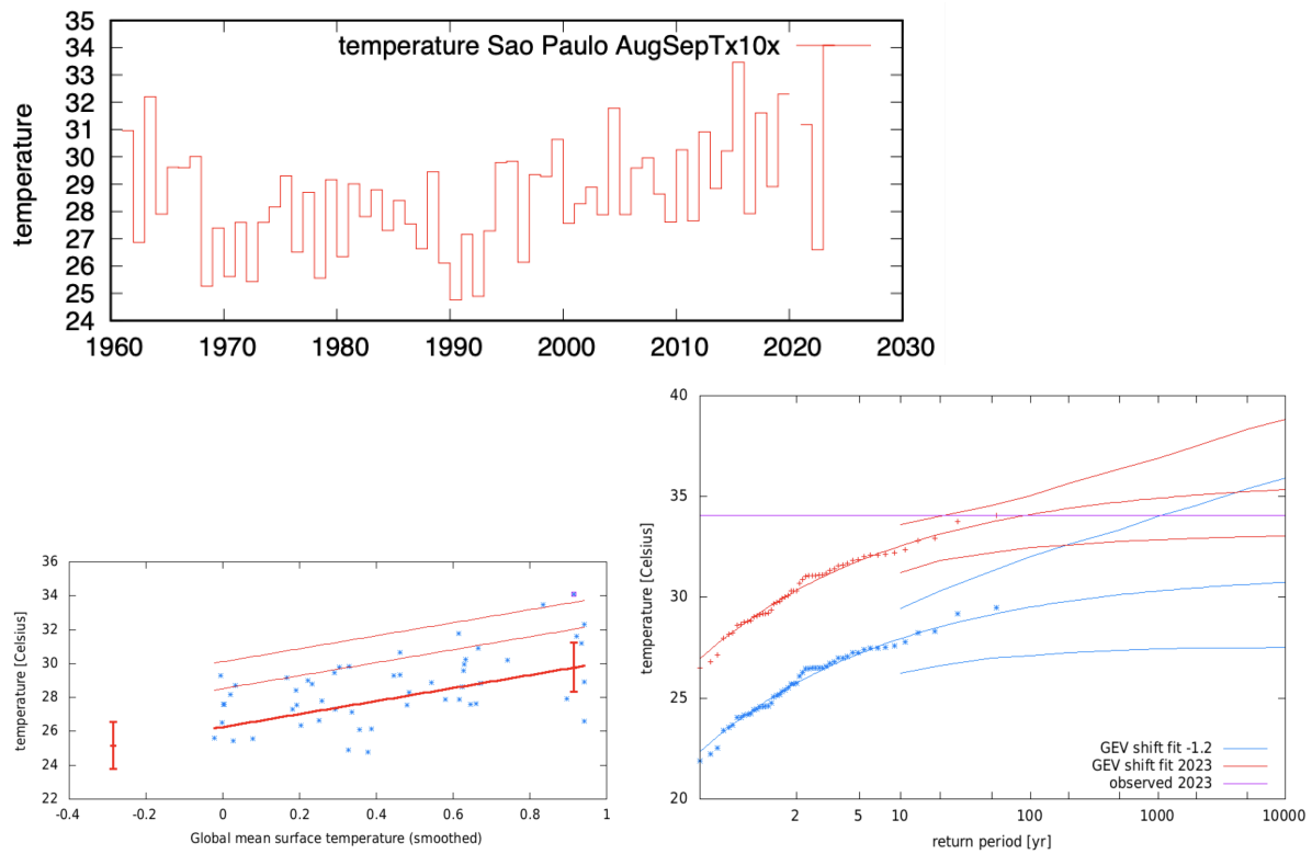
Figure 5. Time series of AugSepTX10x for the São Paulo station (top), and fitted trends and return level plots for a nonstationary GEV fitted to AugSepTX10x (bottom), similar to Figure 4.
