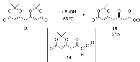
Scheme 3. Kiegiel's Reaction of t -Butanol with Double-Dioxinone 15
