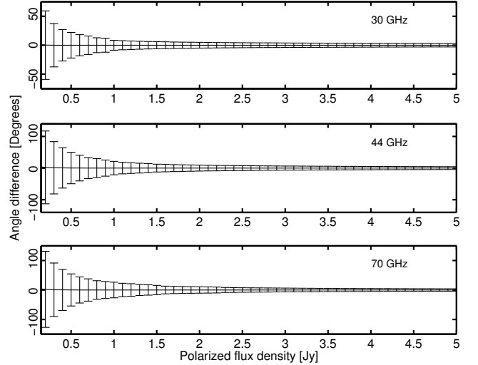
Fig. 21. Internal validation using Monte Carlo simulations to assess the recovery of the polarization angle of the 30, 44, and 70 GHz channels. In these simulations, point sources spanning the full range of polarization angles were injected into the Q and U maps with 50 different polarized flux density values, starting at 0.2 Jy and increasing with a step size of 0.1 Jy. The difference between the recovered and true angles is plotted against the true polarized flux density. Here we see there are no biases in the recovery of the polarization angle.
