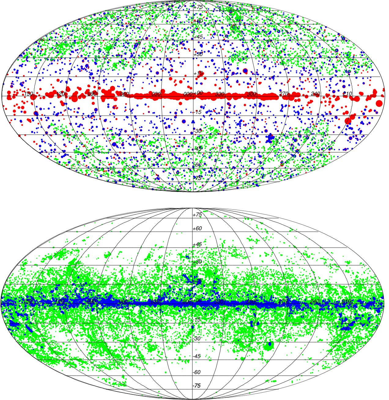
Fig. 2. Top: Distribution of the validated sources from the PCCS2. Red, blue, and green circles show sources from the 30, 143, and 857 GHz catalogues, respectively. Bottom: Location of the sources in the 143 and 857 PCCS2E. The figure is a full-sky Mollweide projection with the Galactic equator horizontal; longitude increases to the left with the Galactic centre in the centre of the map. The size of the filled circles gives an idea of the relative flux densities of the sources per frequency, with larger circles corresponding to larger flux densities. Note that a different size range for each channel was necessary for visualization purposes.
