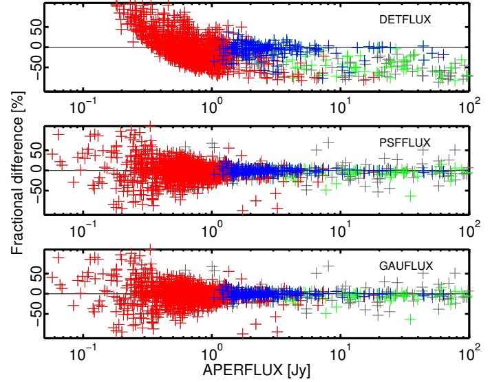
Fig. 10. Comparison of the DETFLUX, PSFFLUX, and GAUFLUX flux-density estimates with APERFLUX for the PCCS2 30 GHz catalogue. The fractional difference is defined as (S - S_{\text{APERFLUX}})/S_{\text{APERFLUX}} . The green and blue points correspond to sources where S_{\text{APERFLUX}}/S_{\text{APERFLUX\_ERR}} > 5 . Grey and green points correspond to sources with |b| < 5^\circ while the red and blue have |b| > 5^\circ .
