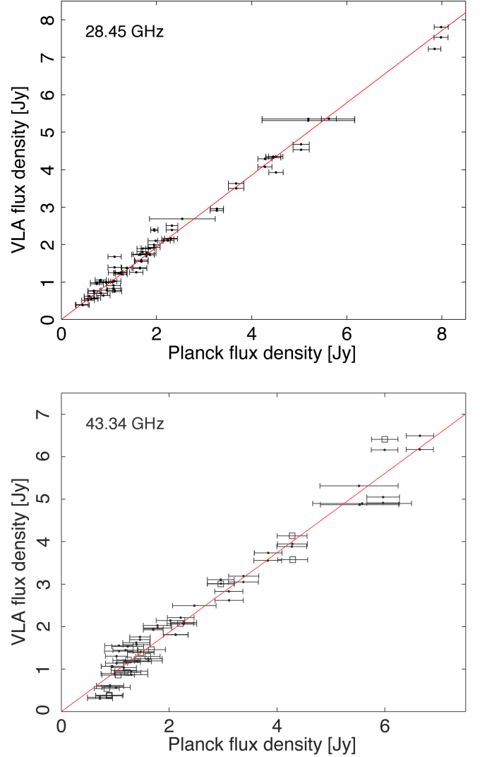
Fig. 15. Comparison of simultaneous colour-corrected flux density measurements by Planck and the VLA at 28.45 GHz (top) and Planck and the VLA (dots)/ATCA (open squares) 43.34 GHz (bottom). The best fit line is shown in red. The Planck 44 GHz channel is noisier than the 30 GHz channel and shows Eddington bias at low flux densities. Some sources have larger error bars than others because they lie close to the Galactic plane where the uncertainties in the measured flux densities can be large. The tiny VLA error bars have not been plotted for clarity.
