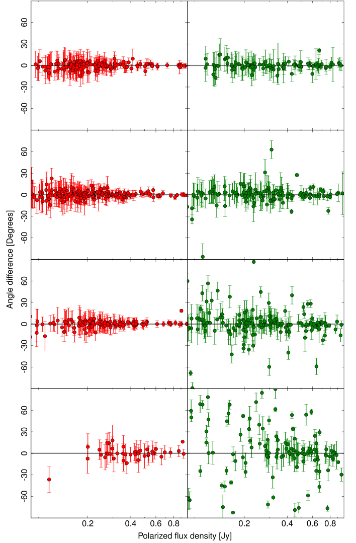
Fig. 23. Difference between the recovered and true polarization angles, from top to bottom, for the 100–353 GHz FFP8 simulations. Left (red): PCCS2. Right (green): PCCS2E. These are the significantly polarized sources, as found by the common method, and the uncertainties associated with the best-fit estimates are \pm 3\sigma error bars.
