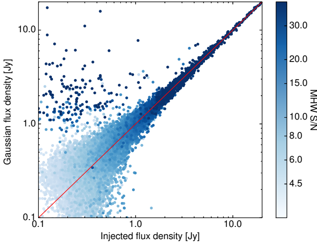
Fig. B.2. Comparison of injected and recovered Gaussian flux densities for point sources at 100 GHz. The saturation of points is proportional to the S/N of the MHW2 detection. Gaussian fitting improves the outlier flux densities slightly, but the flux-density estimates are still biased.
