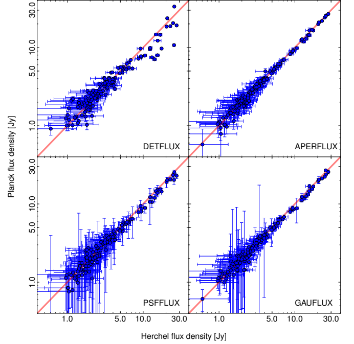
Fig. 17. Comparison of flux densities from Planck and Herschel at 350\,\mu\text{m} (857 GHz) using the Herschel Reference Survey. The one-to-one lines are shown in red.
