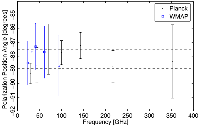
Fig. 24. Polarization position angles for Tau A from WMAP (blue squares, Weiland et al. 2011) and Planck (black dots). The IRAM measurement from Aumont et al. (2010) is also shown (solid line).
