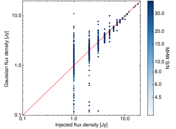
Fig. B.4. Comparison of injected and recovered Gaussian flux densities for cold cores at 100 GHz. The saturation of points is proportional to the S/N of the MHW2 detection. The visible digitization is because only integer values were used for the flux densities of injected sources.
