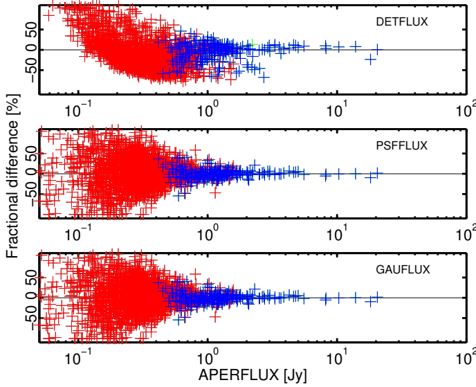
Fig. 12. Comparison of the DETFLUX, PSFFLUX, and GAUFLUX flux-density estimates with APERFLUX for the PCCS2 143 GHz catalogue. The fractional difference is defined as (S - S_{\text{APERFLUX}})/S_{\text{APERFLUX}} . The blue points correspond to sources where S_{\text{APERFLUX}}/S_{\text{APERFLUX\_ERR}} > 5 .
