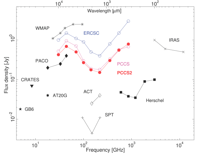
Fig. 1. Sensitivity (the flux density at 90 % completeness) of the PCCS2, compared with PCCS, ERCSC, WMAP and others. The sensitivities displayed for the LFI channels are for the full sky. For the HFI channels, the 90 % completeness limits plotted for the PCCS were evaluated in the extragalactic zone as defined in Planck Collaboration XXVIII (2014) . The regions of sky to which the 90 % completeness limits apply are therefore similar but not identical to those of the PCCS2. These comparisons are discussed further in Sect. 4.
