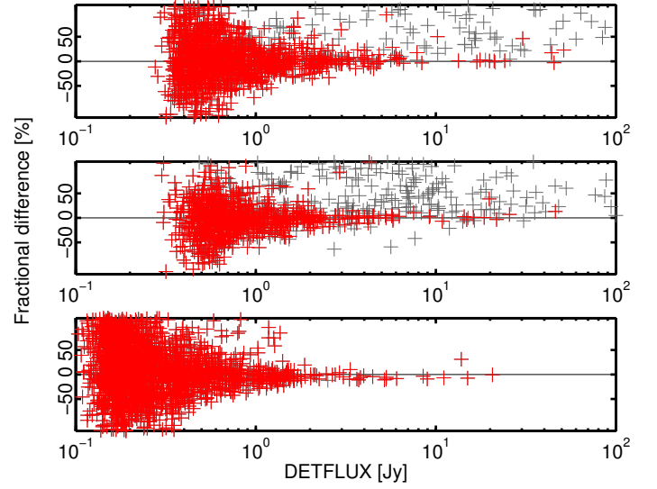
Fig. 14. Comparison of the APERFLUX flux-density estimates with DETFLUX for the PCCS2 30 GHz ( top panel ), 70 GHz ( middle panel ) and 143 GHz ( bottom panel ) catalogues. The fractional difference is defined as (S_{\text{APERFLUX}} - S_{\text{DETFLUX}})/S_{\text{DETFLUX}} . Grey points: |b| < 5^\circ ; red points: |b| > 5^\circ . The greater depth of the 143 GHz catalogue is clear.
