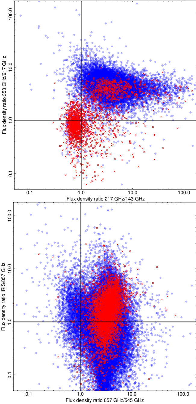
Fig. 26. Colour-colour plots. Red crosses represent sources from the PCCS2 and blue diamonds sources from the PCCS2E. Top panel: common frequency 217 GHz: we can see the non-thermal and thermal source populations of the PCCS2; the PCCS2E contains significantly more thermal sources than the PCCS2, as expected given that PCCS2E contains the Galactic plane region. Bottom panel: common frequency 857 GHz: the PCCS2 is consistent with a population of cold sources spanning a narrow range in temperature, whereas the PCCS2E shows a wider distribution of source properties.
