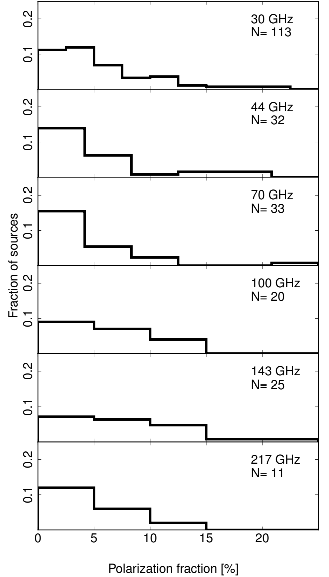
Fig. 5. Normalized histograms of the recovered polarization fraction from the PCCS2 catalogue from 30 to 217 GHz (the 353 GHz channel is not shown because the catalogue contains only one source). The number of sources in each histogram is indicated.
