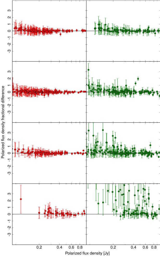
Fig. 22. Fractional difference between the true and recovered polarized flux densities, from top to bottom, for the 100–353 GHz FFP8 simulations. Left (red): PCCS2. Right (green): PCCS2E. Fractional difference is defined as recovered minus true divided by the true value. These are the significantly polarized sources, as found by the common method, and the uncertainties associated with the best-fit estimates are \pm 3\sigma error bars. Eddington bias is seen at lower polarized flux densities.
