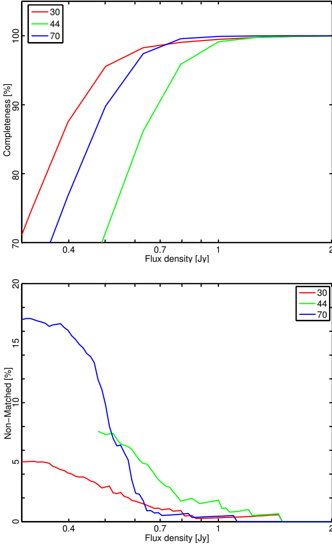
Fig. 6. External validation summary of the 30, 44, and 70 GHz channels. The top panel shows the cumulative completeness per flux-density bin of the PCCS2 catalogue. The lower panel shows the number of unidentified sources per flux-density bin. These sources have no clear counterpart in any of the external catalogues, but have been matched in a neighbouring Planck channel in this release.
