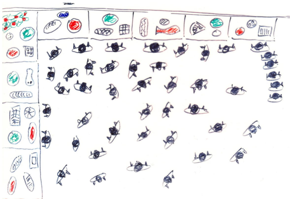
Figure 2. Daan's splendid "dinner party" cartoon on entropy driven phase transitions in mixtures of different sized/shaped particles: a) a low-density mixed state where the diners and tables are distributed evenly in space; b) high density demixed state where the diners and tables are separated to allow more free space and movement for the dinner guests.
