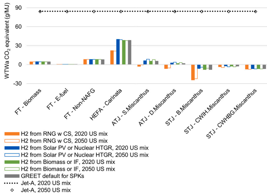
Fig. 7. WTWa CO 2 equivalent emission comparison of low-carbon 100 % SPK feedstocks and pathways for 2020 and 2050 US energy mix scenarios using hydrogen produced from less carbon intense scheme (with only CO 2 emissions in PTWa phase) [FT: Fischer Tropsch; NAFG: North American flared gas; D: distributed; S: standalone; ATJ: alcohol to jet; STJ: sugar to jet; CWIH: catalytic with in-situ H 2 plant type; catalytic with H 2 from biomass gasification plant type; RNG: renewable natural gas; CS: carbon sequestration; PV: photovoltaics; HTGR: high temperature gas reactor; IF: integrated fermentation; SPK: synthetic paraffin kerosene].
