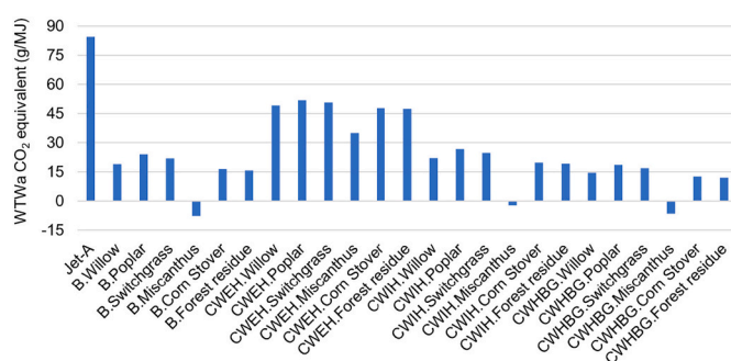
Fig. 6. WTWa CO 2 equivalent emission comparison of different STJ feedstocks for 2020 (with only CO 2 emissions in PTWa phase) [B: biological; CWEH: catalytic with external H 2 plant type; CWHI: catalytic with in-situ H 2 plant type; CWHBG: catalytic with H 2 from biomass gasification plant type].
