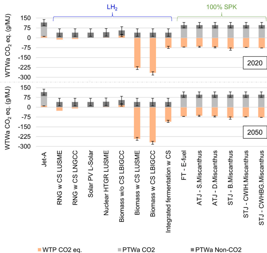
Fig. 8. WTWa CO 2 equivalent emission comparison for different LH 2 and 100 % SPK feedstock and pathways for 2020 and 2050 US energy mix scenarios including non-CO 2 effects [w: with; w/o: without; CS: carbon sequestration; RNG: renewable natural gas; LUSME: liquefaction using US mix of electricity; PV: photovoltaics; HTGR: high temperature gas reactor; LNGCC: liquefaction using power from natural gas combined cycle; LBIGCC: liquefied using electricity from biomass integrated gasification combined cycle; FT: Fischer Tropsch; D: distributed; S: standalone; ATJ: alcohol to jet; STJ: sugar to jet; B: biological; CWIH: catalytic with in-situ H 2 plant type; CWHBG: catalytic with H 2 from biomass gasification plant type].
