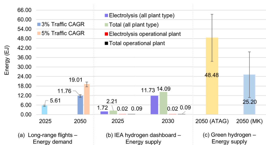
Fig. 10. Energy demand forecast for long-haul aviation and supply of green hydrogen [ATAG: Air Transport Action Group report; MK: McKinsey report; CAGR: compound annual growth rate].
