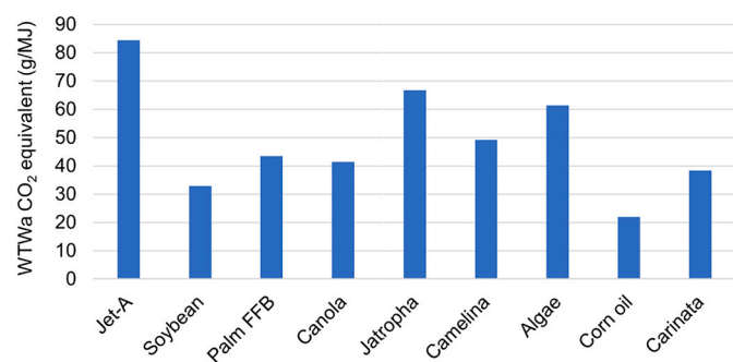
Fig. 4. WTWa CO 2 equivalent emission comparison of different HEFA feedstocks for 2020 (with only CO 2 emissions in PTWa phase).
