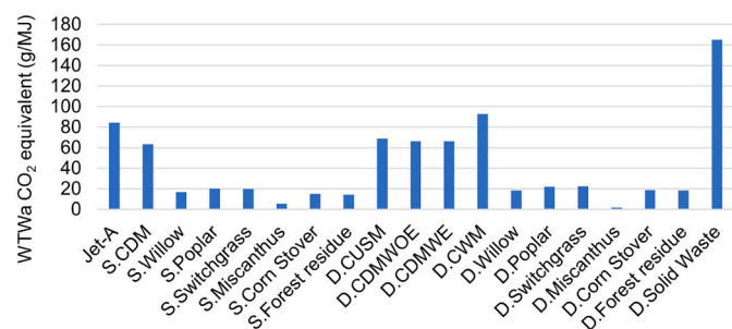
Fig. 5. WTWa CO 2 equivalent emission comparison of different ATJ feedstocks for 2020 (with only CO 2 emissions in PTWa phase) [S; standalone; CDM: corn with dry mill; D: distributed; CUSM: corn US mix; CDMWOE: corn dry mill without extraction; CDMWE: corn dry mill with extraction; CWM: corn wet mill].
