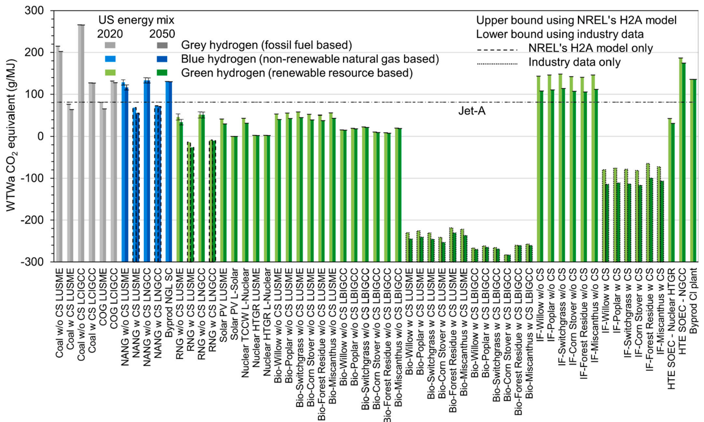
Fig. 2. WTWa comparison of different LH 2 feedstocks and pathways for 2020 and 2050 (with only CO 2 emissions in PTWa phase) [w/o: without; w: with; CS: carbon sequestration; LUSME: liquification using US mix of electricity; COG: coke oven gas; LCIGCC: liquification using electricity from coal integrated gasification combined cycle; NANG: North American natural gas; LNGCC: liquification using power from natural gas combined cycle; NGL: natural gas liquid; SC: steam cracking; RNG: renewable natural gas; L-liquification; PV: photovoltaic; TCCW: thermochemical cracking of water; HTGR: high temperature gas reactor; LBIGCC: liquified using electricity from biomass integrated gasification combined cycle; IF: integrated fermentation; HTE: high temperature electrolysis; SOEC: Solid oxide electrolysis cell; NGCC: natural gas combined cycle].
