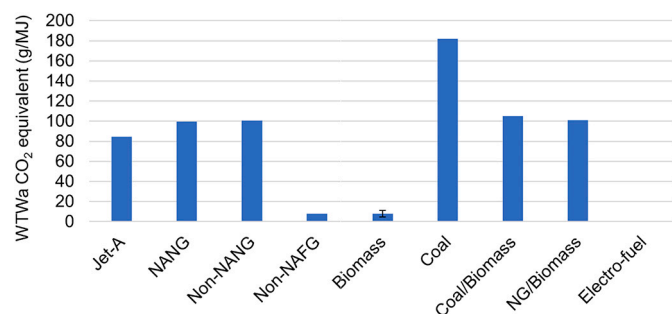
Fig. 3. WTWa CO 2 equivalent emission comparison of different FT feedstocks for 2020 (with only CO 2 emissions in PTWa phase) [NANG: North American natural gas; NAFG: North American flared gas].
