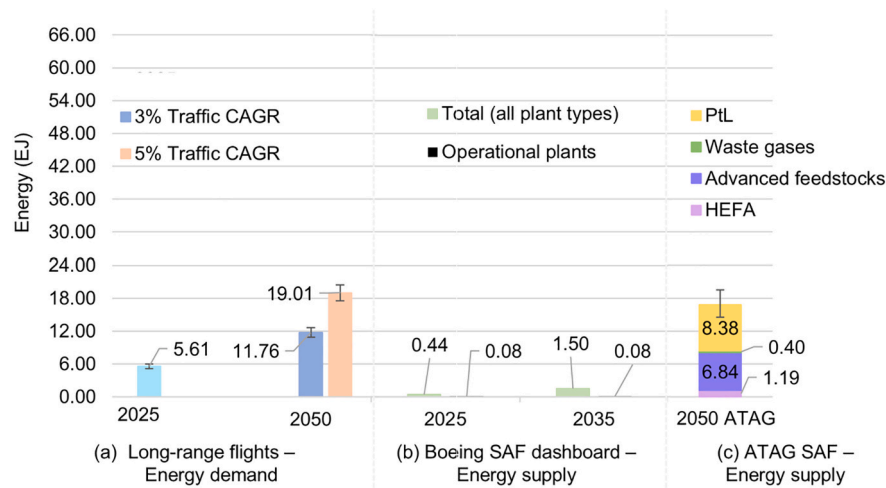
Fig. 9. Energy demand forecast for long-haul aviation and supply of SAF [HEFA: hydro-processed esters and fatty acids; PtL: power to liquid fuel; CAGR: compound annual growth rate].
