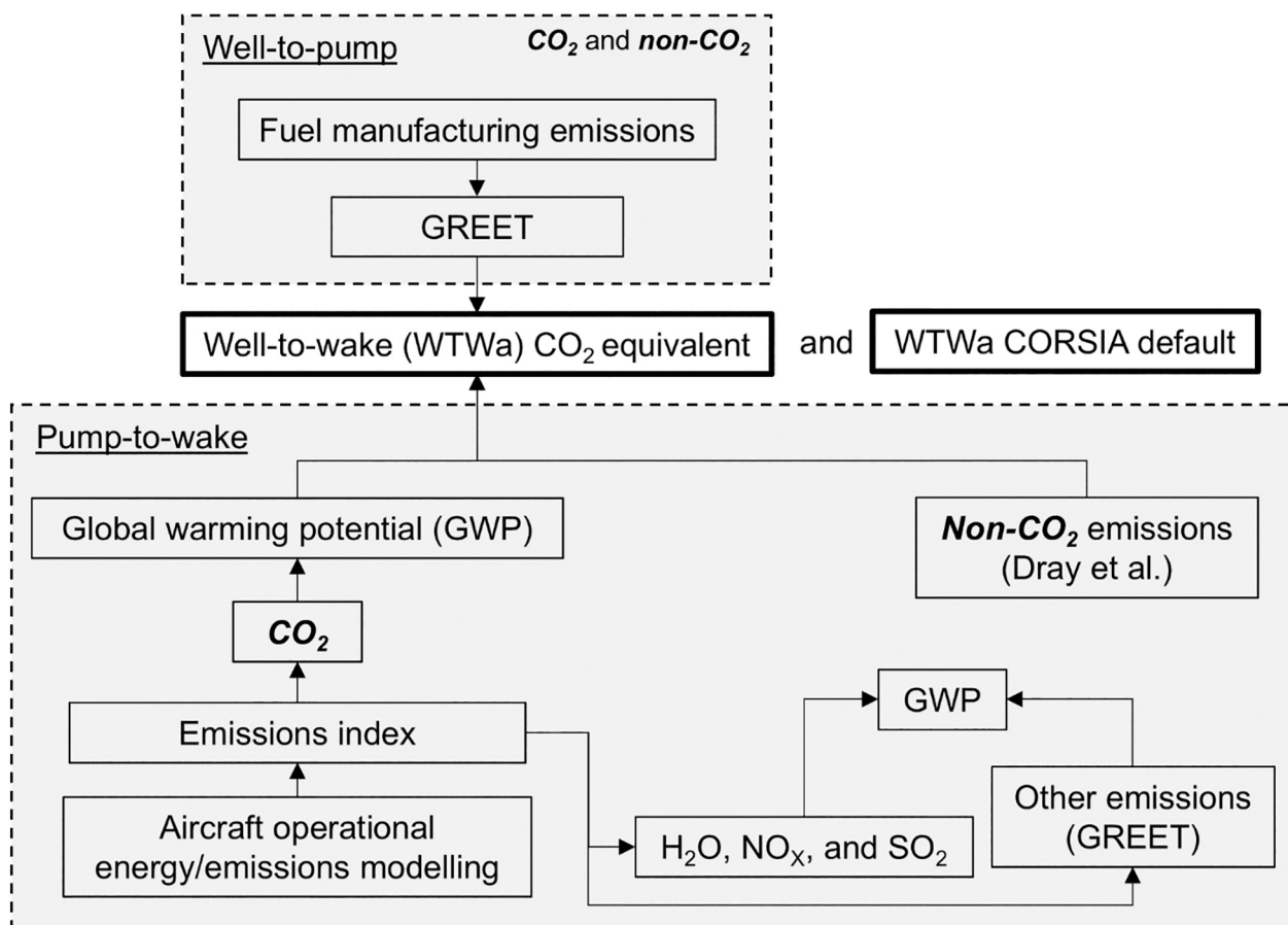
Fig. 1. Schematic of WTWa emissions calculation process from WTP and PTWa emissions.
