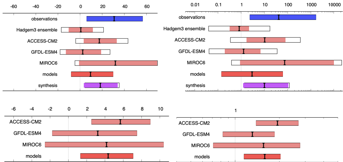
Fig 6.4: Synthesised changes for mean precipitation on stormy days in the UKIre domain. Changes in intensity (left) and PR (right) are shown for a historical period comparing the past 1.2°C cooler climate with the present (top row) and for a future period, based on model projections only, comparing the present and a 2°C warmed climate (bottom row).
