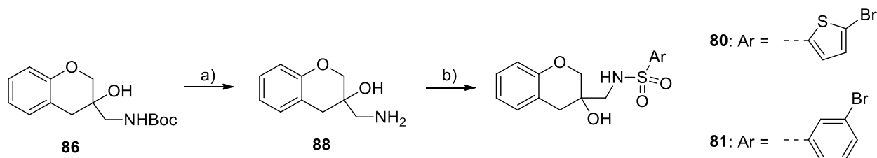
Scheme 13. Preparation of final compounds 80 and 81 . Reagents and conditions: a) TFA, DCM, 0 °C, 30 min, 33%; b) ArSO 2 Cl, Et 3 N, DCM, rt, 16 h, 15-70%.
