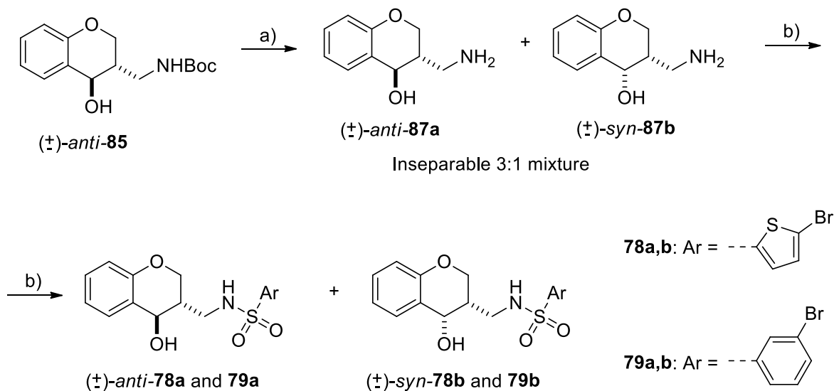
Scheme 12. Preparation of final compounds 78a,b and 79a,b . Reagents and conditions: a) TFA, DCM, 0 °C, 30 min, 57%; b) ArSO 2 Cl, Et 3 N, DCM, rt, 16 h, 77-93%.
