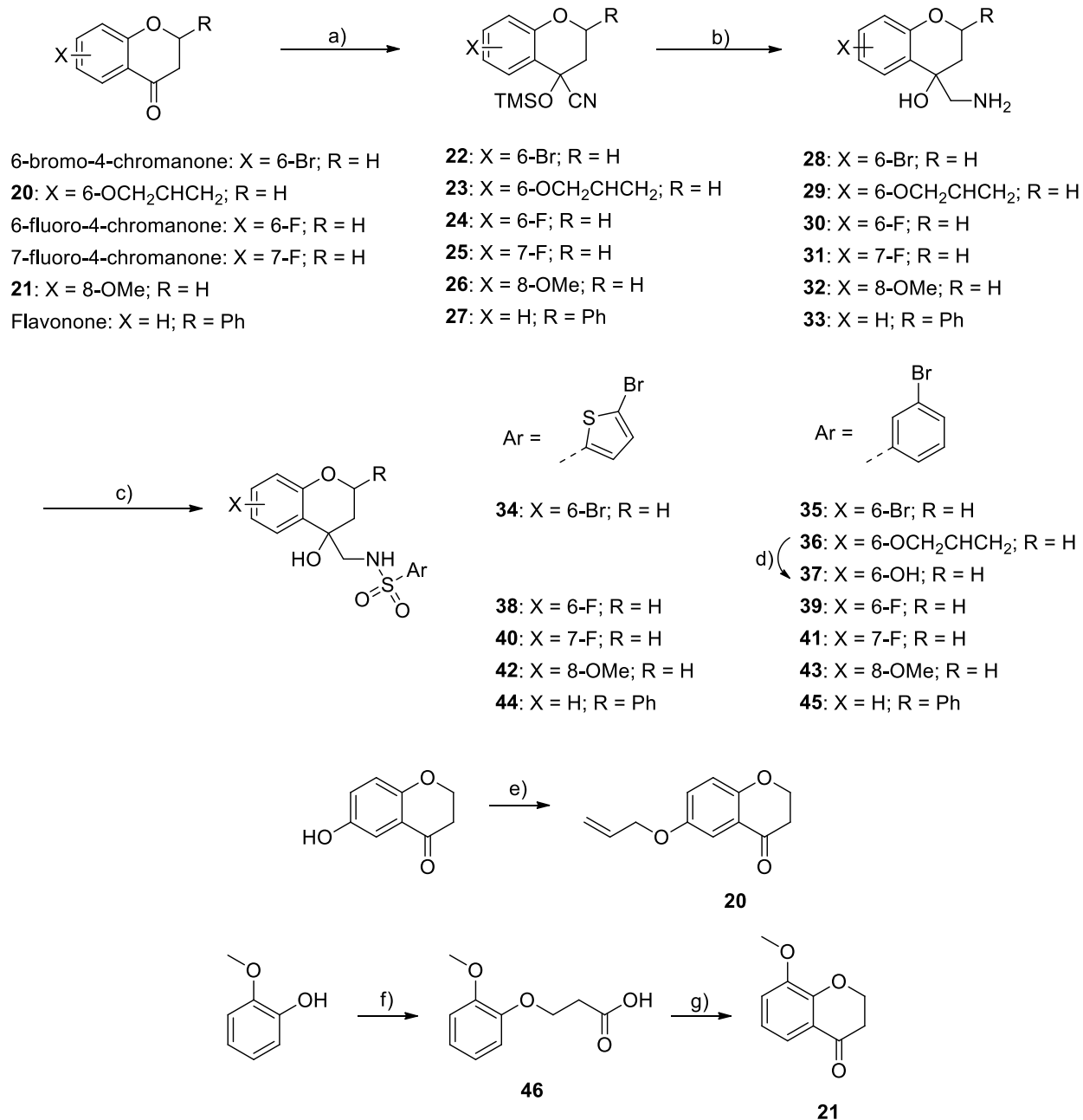
Scheme 3. Study of substitution in the core chromane scaffold. Reagents and conditions: a) TMSCN, ZnI 2 , DCM, rt, 16 h, 65-91%; b) LAH, THF, rt, 16 h, 23-70%; c) ArSO 2 Cl, Et 3 N, DCM, rt, 16 h, 28-90%; d) Pd(PPh 3 ) 4 , K 2 CO 3 , MeOH, reflux, 16 h, 75%; e) allyl bromide, K 2 CO 3 , acetone, reflux, 16 h, 85%; f) 3-bromopropionic acid, NaH, DMF, rt, 16 h, 17%; g) Eaton's reagent, rt, 16 h, 88%.
