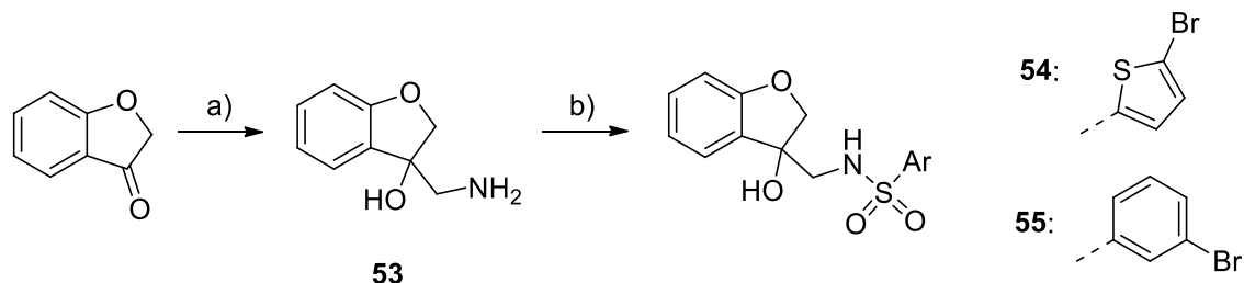
Scheme 5. Synthesis of the reduced core scaffold analogues. Reactants and reagents: a) i) TMSCN, potassium phthalimide, rt, 16 h; ii) LAH, THF, rt, 16 h, 35% (over two steps); b) ArSO 2 Cl, Et 3 N, DCM, 0 °C to rt, 16 h, 51-53%.
