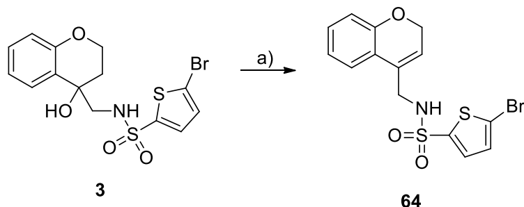
Scheme 7. Removal of the hydroxyl group in compound 3 . Reagents and conditions: a) \text{BF}_3 \cdot \text{Et}_2\text{O} , DCM, 0 °C, 1 h, 11%.
