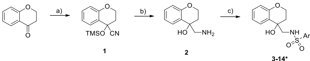
Scheme 1. Study of different aromatic substituents for the sulfonamide. Reagents and conditions: a) TMSCN, ZnI 2 , DCM, rt, 16 h, quant.; b) LAH, THF, rt, 16 h, quant.; c) ArSO 2 Cl, Et 3 N, DCM, rt, 16 h, 4-74%. *Ar groups can be reviewed in Table 1.
