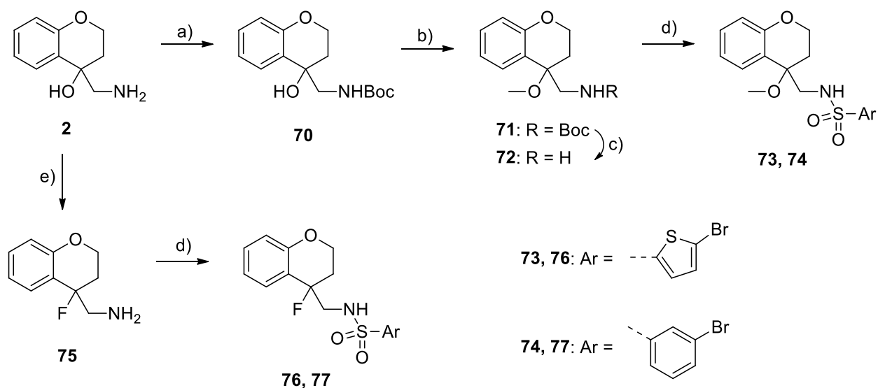
Scheme 9. Synthesis of alkylated and fluorinated analogues. Reagents and conditions: a) \text{Boc}_2\text{O} , \text{Et}_3\text{N} , DCM, 0 °C to rt, 5 h, quant.; b) MeI, \text{K}^t\text{OBu} , THF, 0 °C to rt, 2 h, 70%; c) 1M TBAF in THF, reflux, 16 h, 39%; d) \text{ArSO}_2\text{Cl} , \text{Et}_3\text{N} , DCM, rt, 16 h, 44-84%; e) DAST, DCM, -78 °C to rt, 3 h, 31%.
