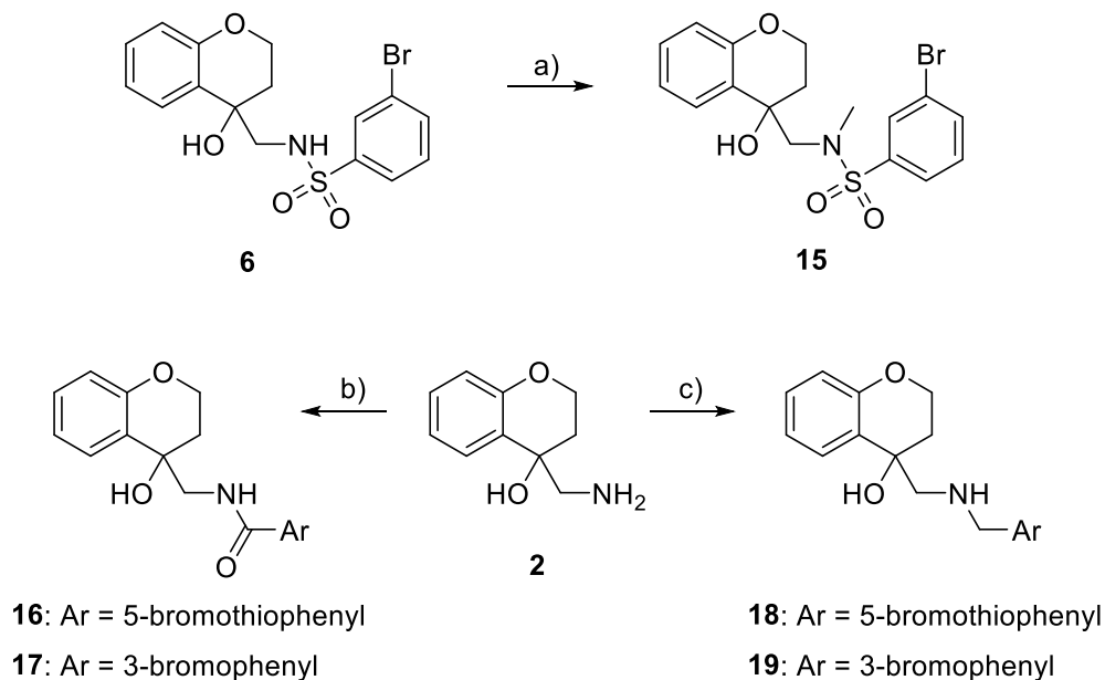
Scheme 2. Study of the sulfonamide linker. Reagents and conditions: a) MeI, K 2 CO 3 , DMF, 50 °C, 4 h, 80%; b) ArCOOH, EDC, HOBT, Et 3 N, DCM/DMF, rt, 16 h, 55-68%; c) ArCHO, 2-picoline borane, MeOH, rt, 24 h, 10-50%.
