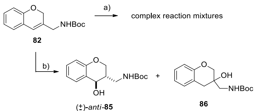
Scheme 11. Hydroboration-oxidation of 82 . Reagents and conditions: a) i) 1M \text{BH}_3 \cdot \text{THF} , 0 °C to rt, 2 h; ii) \text{H}_2\text{O}_2 , NaOH, \text{H}_2\text{O} , 0 °C to rt, 16 h; b) i) 1M \text{BH}_3 \cdot \text{THF} , 0 °C to rt, 2 h; ii) \text{NaBO}_3 \cdot 4\text{H}_2\text{O} , \text{H}_2\text{O} , rt, 2 h, 27-49%.
