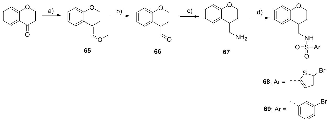
Scheme 8. Preparation of the dehydroxylated derivatives. Reagents and conditions: a) (methoxymethyl)triphenylphosphonium chloride, BuLi, THF, -78 °C to rt, 16 h, 86%; b) 70% HClO 4 , Et 2 O, 0 °C to rt, 45 min, quant.; c) i) NH 2 OH·HCl, EtOH, rt, 45 min ii) Zn, HCl, rt, 15 min, 33%; d) ArSO 2 Cl, Et 3 N, DCM, rt, 16 h, 43-68%.
