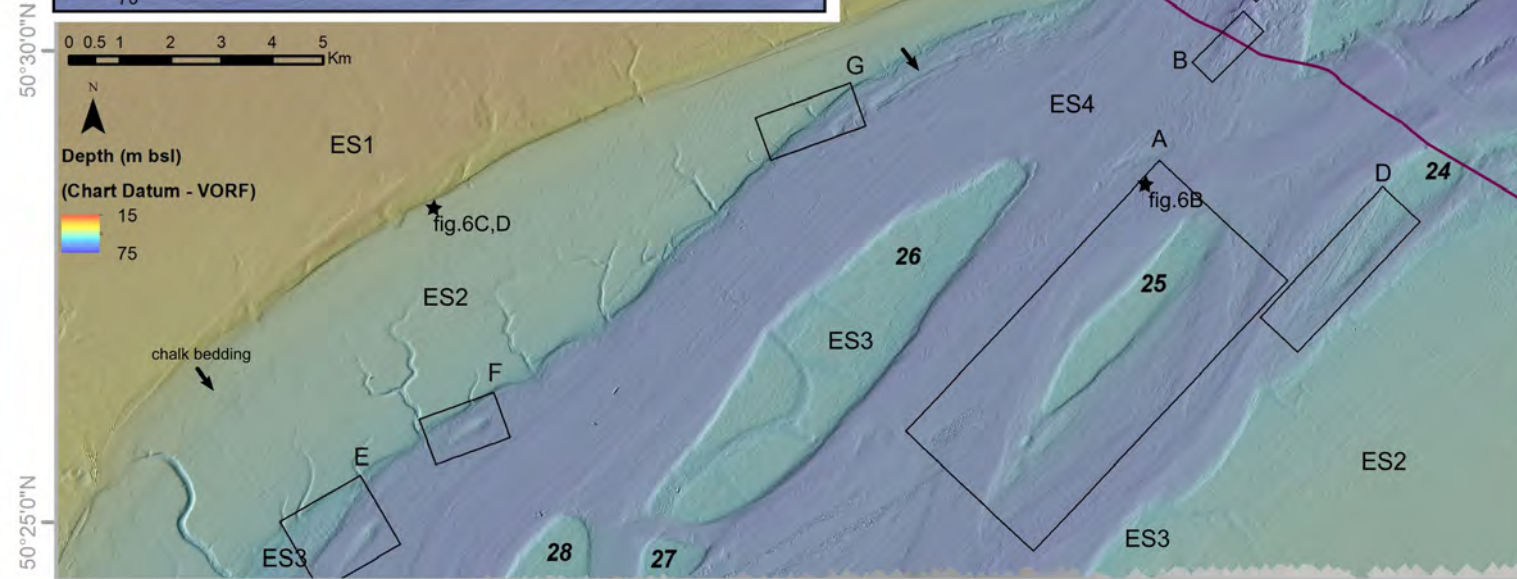
A modern megaripples original island 25 island erosional remnants 1.5 km m bsl 30 70
