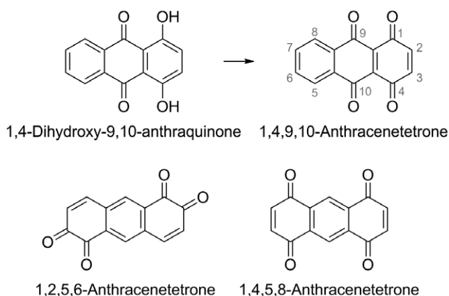
Scheme 1. Facile synthesis of 1,4,9,10-anthracenetetrone starting from 1,4-dihydroxy-9,10-anthraquinone (top), molecular structure of 1,2,5,6- and 1,4,5,8-anthracenetetrone (bottom).
