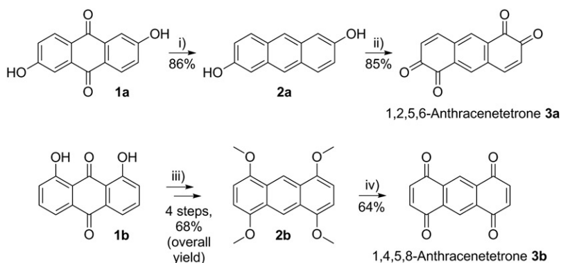
Scheme 2. (i) Reduction of 2,6-dihydroxy-9,10-anthraquinone ( 1a ) to 2,6-dihydroxyanthracene ( 2a ). Conditions: \text{NaBH}_4 , 1 M \text{Na}_2\text{CO}_3 solution, under argon, RT, overnight. (ii) Oxidation to 1,2,5,6-anthracenetetrone ( 3a ). Conditions: benzeneseleninic acid anhydride, dry THF, under argon, 50^\circ\text{C} , 3 h. (iii) Conversion of 1,8-dihydroxy-9,10-anthraquinone ( 1b ) into 1,4,5,8-tetramethoxyanthracene ( 2b ). Conditions: see Ref. [28], and (iv) Oxidation to 1,4,5,8-anthracenetetrone 3b . Conditions: silica-supported ceric ammonium nitrate (CAN), \text{CH}_2\text{Cl}_2 , RT, 1 h.
