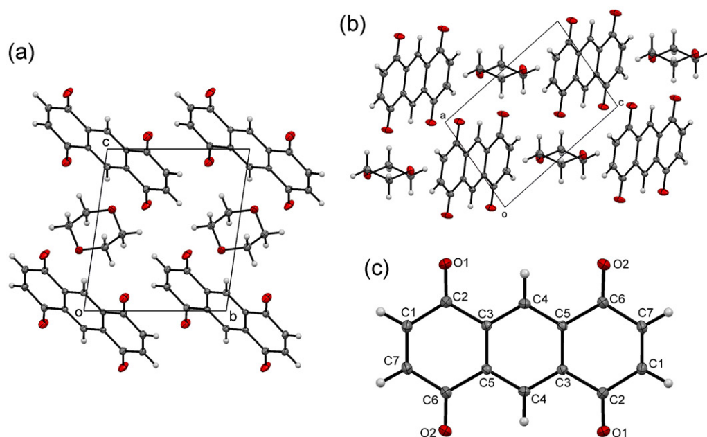
Figure 1. Crystal structure of 3b ·1,4-dioxane viewed down (a) [100] and (b) [010]. (c) The molecular structure of 3b . C (grey) and O (red) atoms are represented by ellipsoids drawn at the 50% probability levels; H atoms by white spheres of arbitrary radius.
