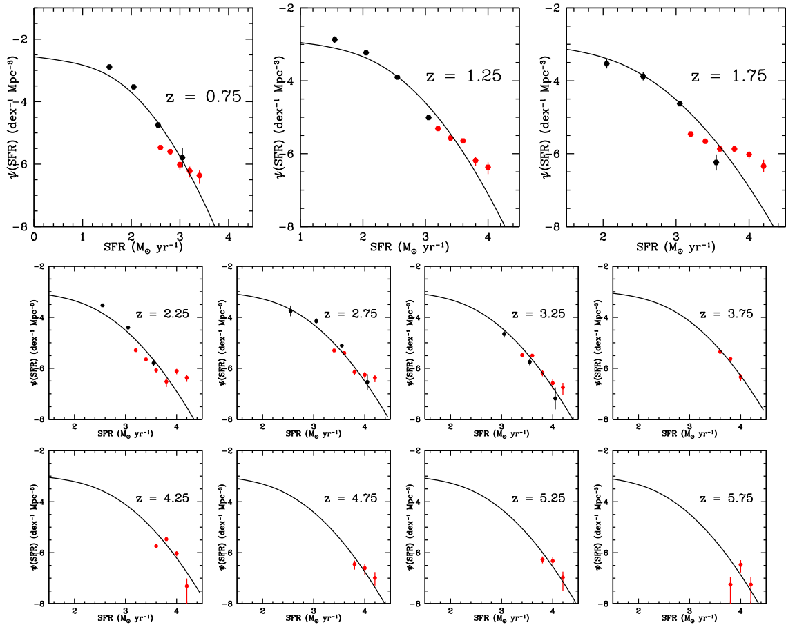
Figure 9. Star formation rate functions for starburst galaxies for z = 0.5 – 6.0 , in bins of 0.5 in redshift. Red points are from present HerMES-SWIRE study, black points are from Gruppioni et al. 2013.
