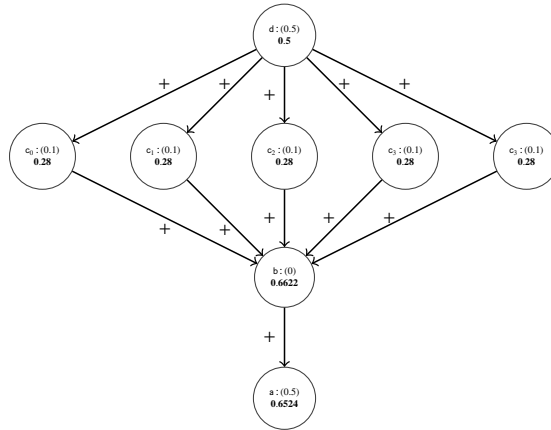
Fig. 39. \text{Ctrb}^{\partial} violates the proximity principle w.r.t. QE semantics.
