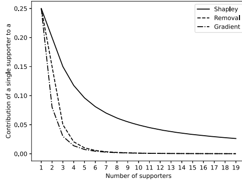
5.2: Contribution of b_i , 1 \leq i \leq n to a , given n .
