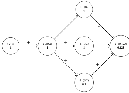
Fig. 35. \text{Ctrb}^{\mathcal{S}} violates the proximity principle w.r.t. DFQuAD semantics.
