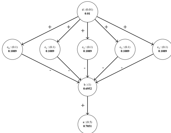
Fig. 40. \text{Ctrb}^{\partial} violates the proximity principle w.r.t. SD-DFQuAD semantics.
