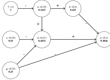
Fig. 38. \text{Ctrb}^{\mathcal{L}} violates the proximity principle w.r.t. EBT semantics.
