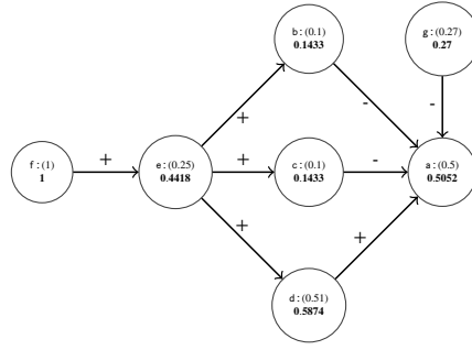
Fig. 37. \text{Ctrb}^{\mathcal{L}} violates the proximity principle w.r.t. EB semantics.
