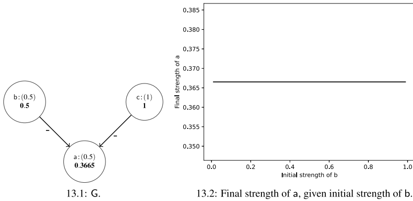
Fig. 13. \text{Ctrb}^{\mathcal{S}} violates local faithfulness w.r.t. EBT semantics.
