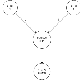
Fig. 28. \text{Ctrb}^{\mathcal{R}} violates the proximity principle w.r.t. SD-DFQuAD semantics.
