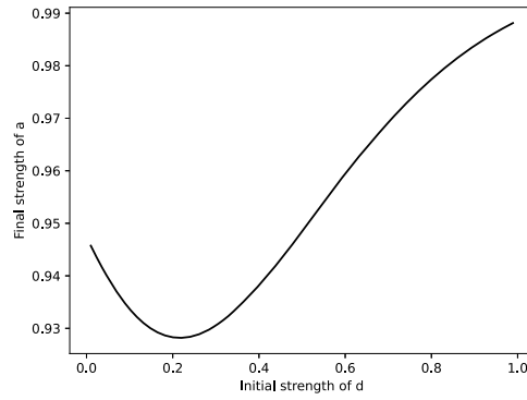
11.2: Final strength of a, given initial strength of d.
