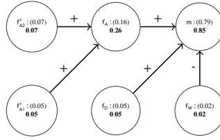
Fig. 26. QBAG for movie rating with initial strengths in normal font and DFQuAD final strength in bold font (taken from [5]).
