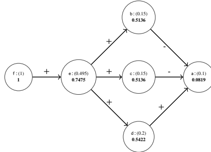
Fig. 19. \text{Ctrb}^{\mathcal{S}} violates the counterfactuality and quantitative counterfactuality principles w.r.t. SD-DFQuAD semantics.
