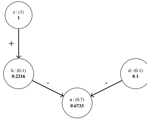
Fig. 16. \text{Ctrb}^{\mathcal{R}'} violates the counterfactuality and quantitative counterfactuality principles w.r.t. EBT semantics.
