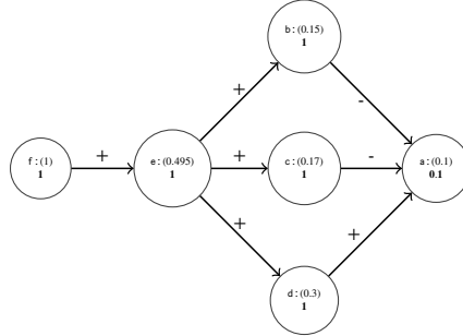
Fig. 18. \text{Ctrb}^{\mathcal{S}} violates the counterfactuality and quantitative counterfactuality principles w.r.t. DFQuAD semantics.
