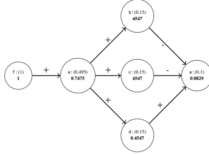
Fig. 34. \text{Ctrb}^{\mathcal{S}} violates the proximity principle w.r.t. QE semantics.
