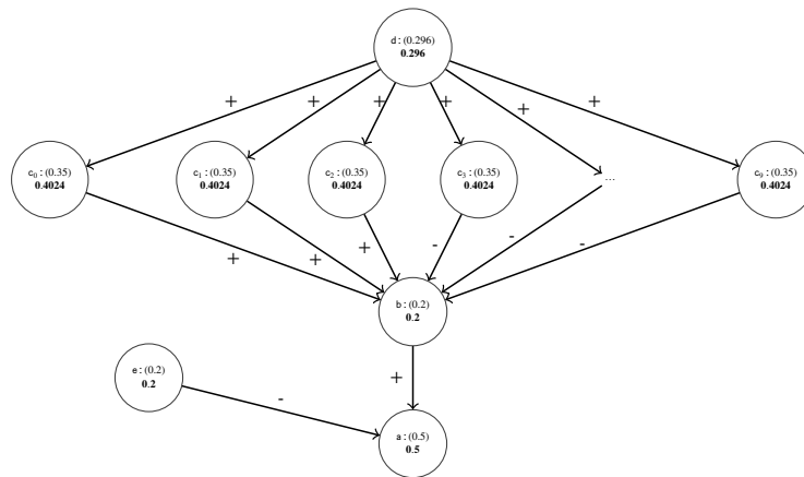
Fig. 22. \text{Ctrl}^b violates the counterfactuality and quantitative counterfactuality principles w.r.t. QE semantics. Note that “...” (with incoming support and outgoing attack) represents arguments c_4 - c_8 with same initial strength and incoming support and outgoing attack as c_3 and c_9 .
