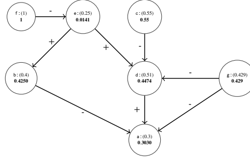
Fig. 21. \text{Ctrb}^{\mathcal{S}} violates the counterfactuality and quantitative counterfactuality principles w.r.t. EBT semantics.
