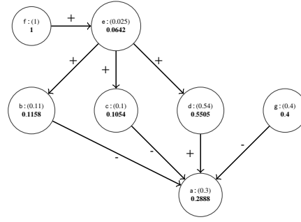
Fig. 20. \text{Ctrb}^{\mathcal{S}} violates the counterfactuality and quantitative counterfactuality principles w.r.t. EB semantics.
