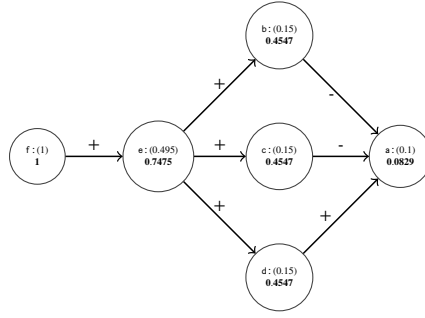
Fig. 17. \text{Ctrb}^{\mathcal{S}} violates the counterfactuality and quantitative counterfactuality principles w.r.t. QE semantics.
