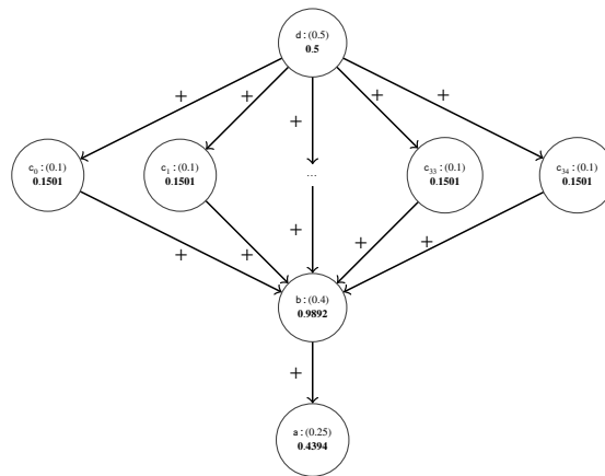
Fig. 41. \text{Ctrb}^d violates the proximity principle w.r.t. EB semantics.
