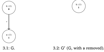
Fig. 3. While our contribution functions can be intuitively expected to satisfy directionality with respect to modular semantics, this may not be the case with respect to other semantics: consider \text{Ctrb}^{\mathcal{R}} and \sigma(x) = \tau(x) - \sum_{\{y|x \in \text{Att}(y)\}} \tau(y) .
