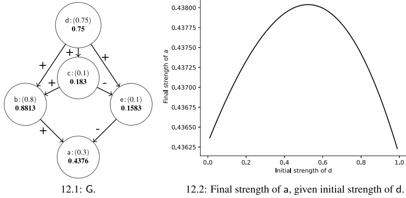
Fig. 12. \text{Ctrb}^{\mathcal{S}} violates local faithfulness w.r.t. EB semantics.
