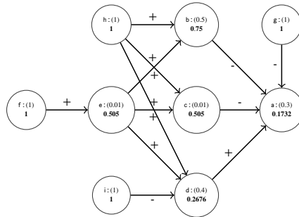
Fig. 36. \text{Ctrb}^{\mathcal{S}} violates the proximity principle w.r.t. SD-DFQuAD semantics.
