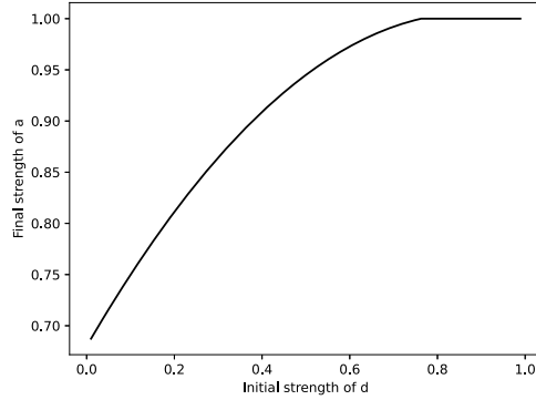
7.2: Final strength of a, given initial strength of d.
