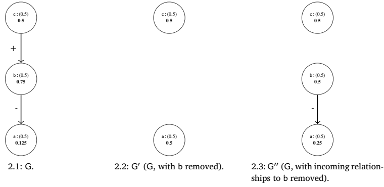
Fig. 2. A QBAG G and its updates, with b (G') and incoming relationships to b removed (G'').
