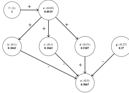
Fig. 15. \text{Ctrb}^{\mathcal{R}'} violates the counterfactuality and quantitative counterfactuality principles w.r.t. EB semantics.
