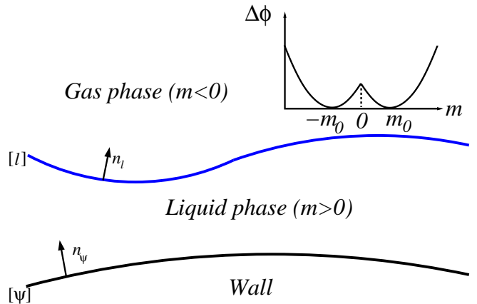
FIG. 1: Schematic illustration of a nonplanar interfacial configuration (blue line) for a constrained wetting film of liquid at a nonplanar wall (black line). Conventions for the surface normals are shown. The inset shows the double-parabola approximation for \Delta\phi(m) .
