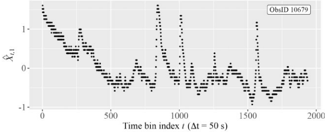
Figure 8. Predicted soft-band states \hat{X}_1, \dots, \hat{X}_{2027} for ObsID 10679.
