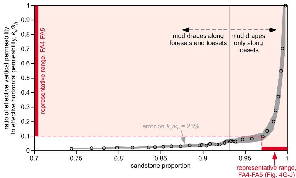
Fig. 6. Plot of k_v/k_h ratio versus sandstone content, for heterolithic trough cross-bedded sandstones that contain mudstone drapes along their foresets and toesets (after Massart et al., 2016, their Fig. 7). Data are derived from small models (3 m x 3 m x 1 m) constructed using outcrop data, and the proportion of foreset-toeset surfaces that are draped by mudstone patches ranges from 100% (at a sandstone proportion of 0.74) to 0% (for a sandstone proportion of 1.00).
