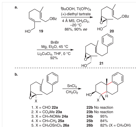
Scheme 5 Synthesis of an epoxy alcohol and derivatization into different substrates for polyene cyclization reactions
