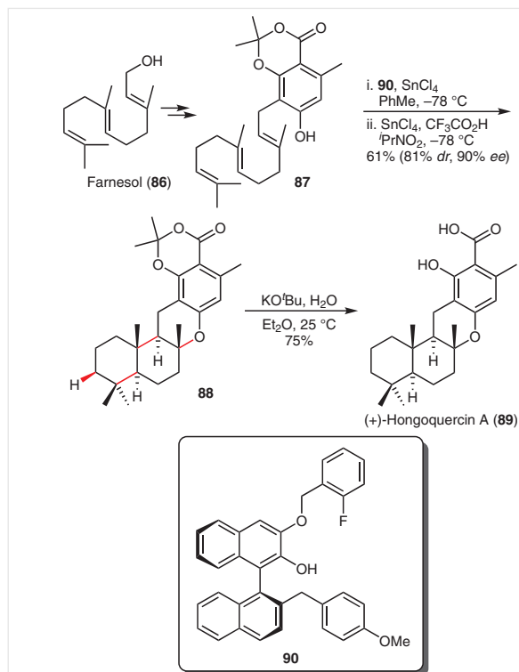
Scheme 19 Synthesis of (+)-hongoquercin A
