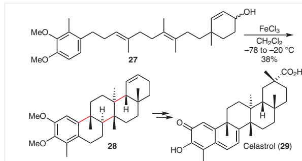
Scheme 6 Synthesis of celastrol
