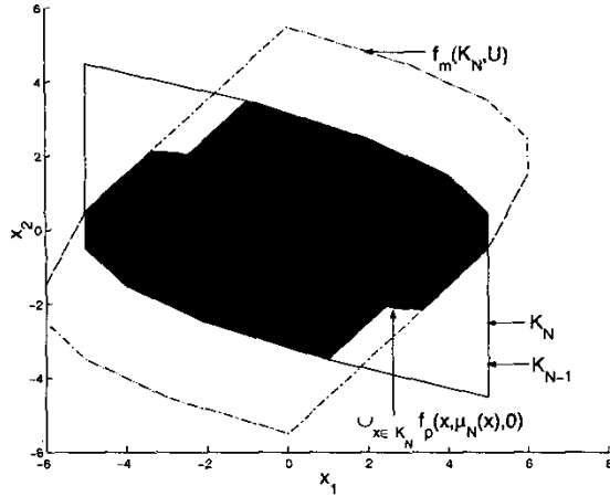
Figure 3: Plot of sets used in Example 21.
