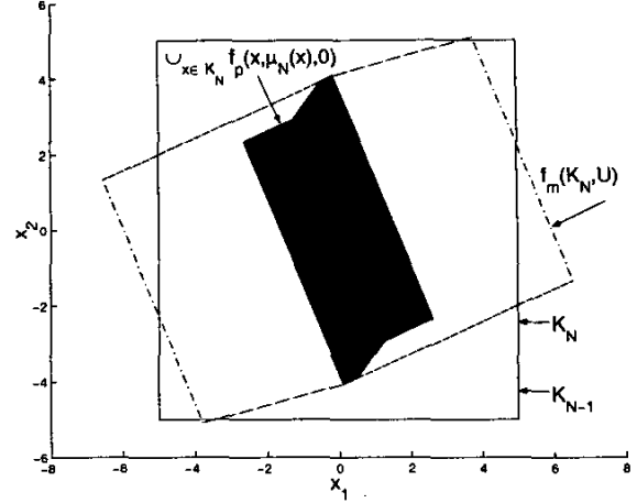
Figure 2: Plots of sets used in Example 19.
