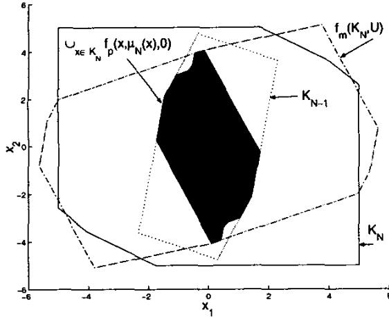
Figure 1: Plots of sets used in Example 18.
