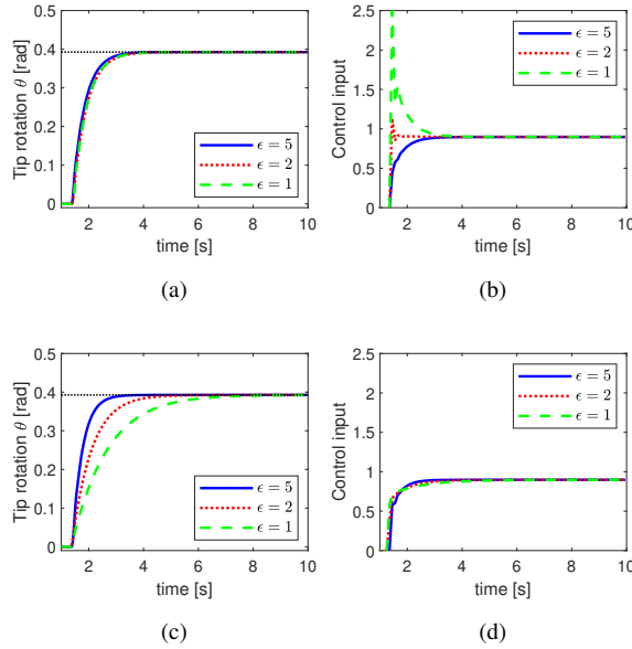
Fig. 2. Simulation results for system (2-3) comparing controller (13) with controller (22) for different parameters \epsilon : (a) tip rotation \theta with (13); (b) control input u with (13); (c) \theta with (22); (d) u with (22).
