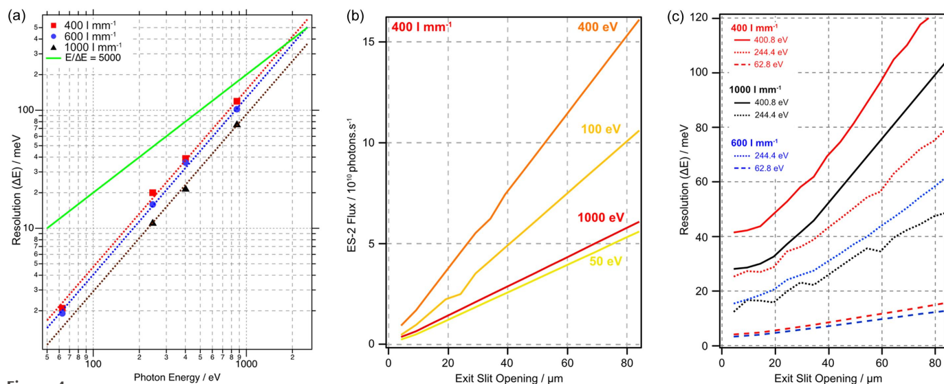
Figure 4 (a) Photon energy resolution ( \Delta E ) as a function of photon energy for the three gratings, measured with a vertical exit slit opening of 4 \mu\text{m} ( 400 \text{ l mm}^{-1} : red squares; 600 \text{ l mm}^{-1} : blue circles; 1000 \text{ l mm}^{-1} : black triangles). (b) Photon flux at ES-2 from the 400 \text{ l mm}^{-1} grating as a function of vertical exit slit opening for four photon energies. (c) Photon energy resolution ( \Delta E ) as a function of vertical exit slit opening for the three gratings at 62.8 \text{ eV} (He, dashed line), 244.4 \text{ eV} (Ar, dotted line) and 400.8 \text{ eV} ( \text{N}_2 , solid line).
