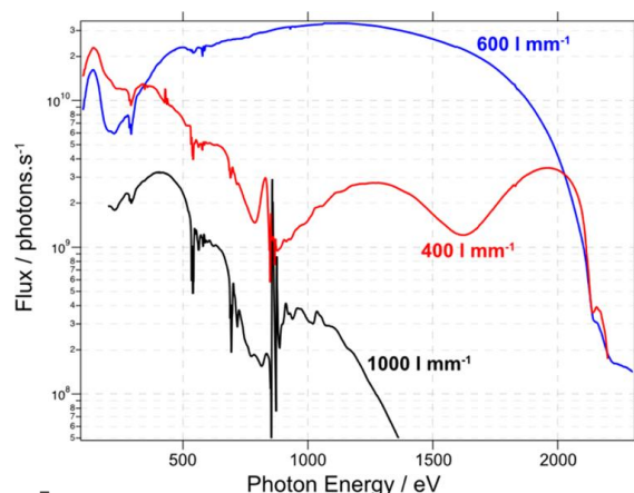
Figure 5 Beamline transmission for the three gratings as measured from a photodiode in ES-2, vertical exit slit opening 9 \mu\text{m} , c_{\text{ff}} 1.4.
