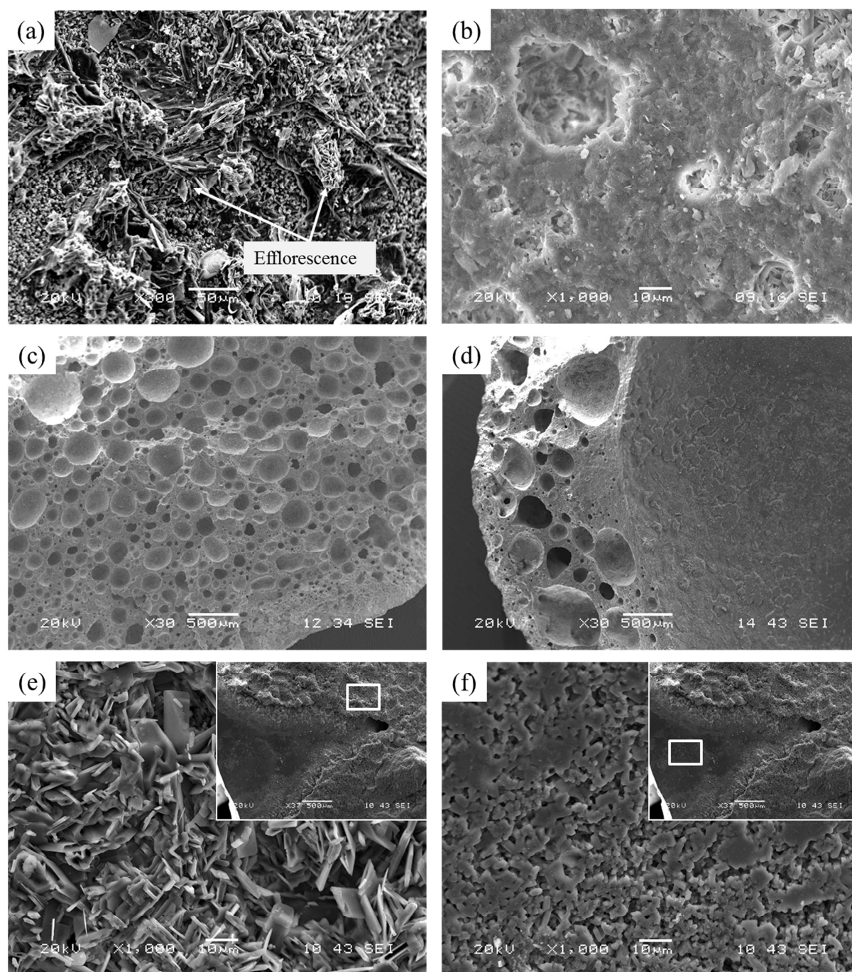
Fig. 5. SEM micrographs of (a) outer surface of DCLWA fired at 1180°C, (b) fracture surface of DCLWA fired at 1180°C (c) fracture surface of W-DCLWA fired at 1160°C (d) fracture surface of W-DCLWA fired at 1190°C (e) – (f) outer surface of W-DCLWA fired at 1170°C (the attached image shows the locations of magnified areas on the outer surface).
