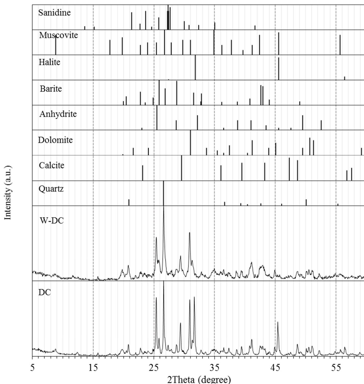
Fig. 1. XRD traces for the as-received drill cuttings (DC) showing the major crystalline phases are quartz ( \text{SiO}_2 ), calcite ( \text{CaCO}_3 ), dolomite ( \text{CaMg}(\text{CO}_3)_2 ), anhydrite ( \text{CaSO}_4 ), barite ( \text{BaSO}_4 ), halite ( \text{NaCl} ), muscovite ( \text{KAl}_2(\text{Si}_3\text{AlO}_{10})(\text{OH})_2 ) and sanidine ( \text{KAlSi}_3\text{O}_8 ). XRD traces for washed drill cuttings (W-DC) shows the absence of NaCl peaks. The representative XRD patterns of the major phases are included with the same intensity scale.
