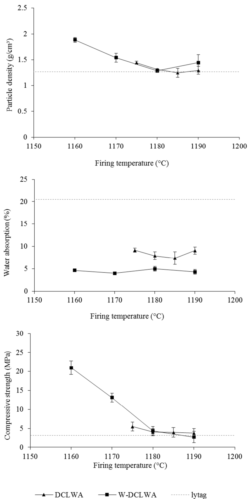
Fig. 4. Particle density, water absorption and compressive strength measured at various firing temperatures for DCLWA and W-DCLWA. Properties of Lytag are marked (dashed line). Error bars are \pm one standard deviation.
