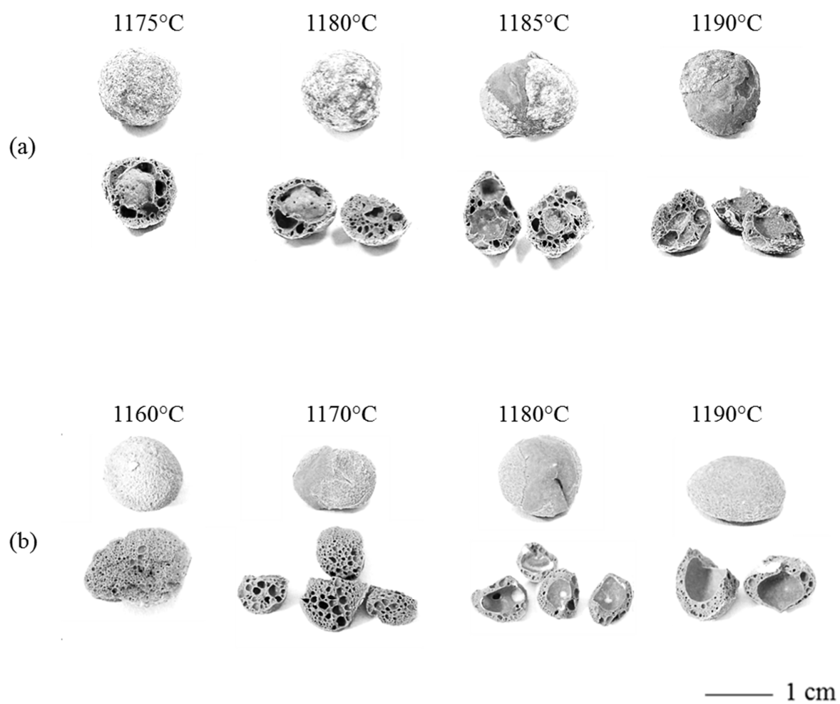
Fig. 3. Appearance and internal structure of (a) DCLWA and (b) W-DCLWA.
