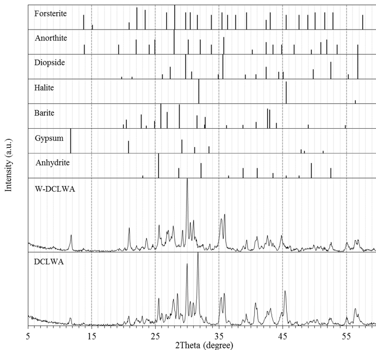
Fig. 6. XRD traces for DCLWA and W-DCLWA manufactured at 1180°C showing that diopside ( \text{CaMgSi}_2\text{O}_6 ) is the major neo-formed crystalline phase present after firing. The representative XRD patterns of the major phases are included with the same intensity scale.
