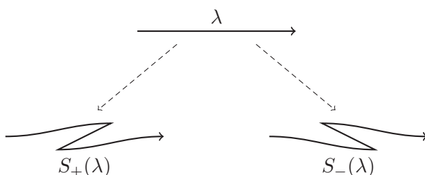
FIGURE 2 Stabilization of an oriented Legendrian knot \lambda . Here, we work locally, in the standard contact (\mathbb{R}^3, \xi = \ker(dz - ydx)) , with each knot shown in the front (xz) -projection.
