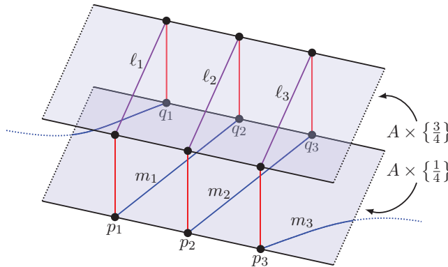
FIGURE 4 The curve \partial D is identified with the union of \ell_i \times \{\frac{3}{4}\} (purple), m_i \times \{\frac{1}{4}\} (blue), p_i \times [\frac{1}{4}, \frac{3}{4}] (red), and q_i \times [\frac{1}{4}, \frac{3}{4}] (red) on the boundary of M_f - U^\circ . For readability, we label \ell_i \times \{\frac{3}{4}\} and m_i \times \{\frac{1}{4}\} with \ell_i and m_i , respectively.
