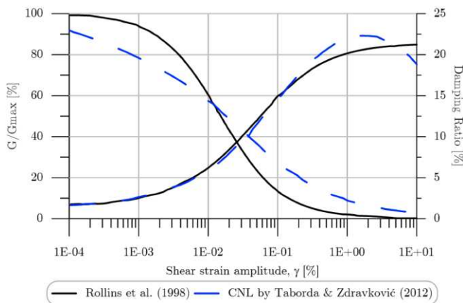
Figure 5. CNL model compared with empirical curves proposed by Rollins et al. (1998). Modified from Taborda & Zdravković (2012).
