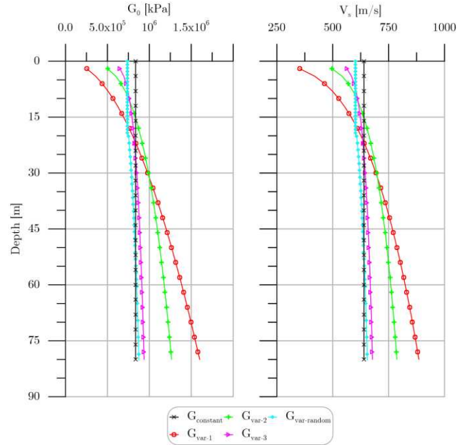
Figure 4. G_0 and V_s for the profiles studied
