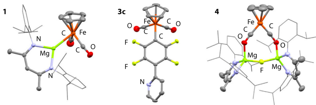
Figure 2. Structures of 1 , 3c and 4 . Selected bond lengths (Å) 1 : 2.5190(7), Fe–CO 1.727(3), 1.744(3), 3c : Fe–CO 1.771(4), 1.772(4), C–O 1.136(4), 1.138(5), Fe–CAr 2.001(3). 4 : Fe–CO 1.679(2), 1.692(2), Mg–O 2.0160(15), 1.9885(17), Mg–F 1.8719(13), 1.8710(13), C–O 1.206(3), 1.200(3).
