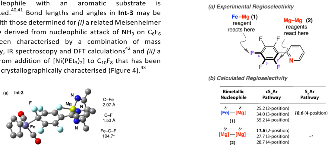
Figure 5. (a) Experimental regioselectivity. (b) Calculated barriers (Gibbs energies in kcal\ mol^{-1} ) for reactions of (2-pentafluorophenyl)pyridine with 1 and 2 by cS_NAr and S_NAr mechanisms. a pathway could not be identified.
