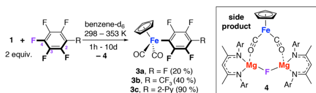
Scheme 1. Reaction of 1 with a series of fluoroarenes.
