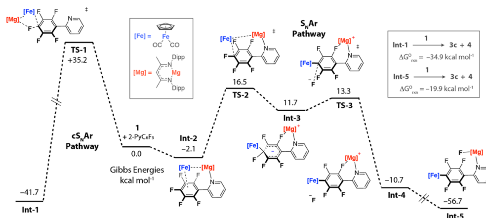
Figure 3. Calculated S_NAr and cS_NAr reaction pathways for the reaction of 1 with the 4-position of 2-(pentafluorophenyl). Insets: Key for abbreviation of the [Fe] and [Mg] fragments and thermodynamics of product generation.
