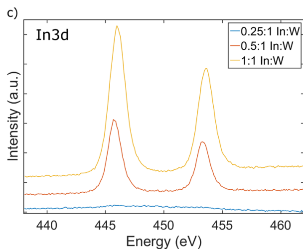
(c) In 3d
