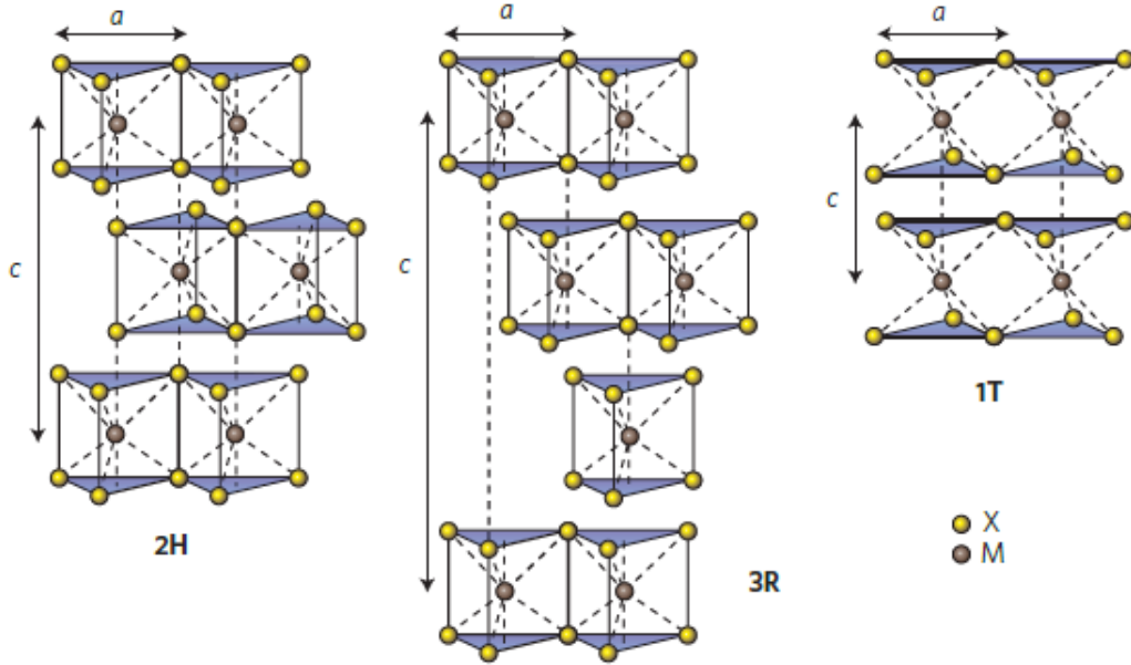
Figure 2.1: Schematics of the structural polytypes: 2H (hexagonal symmetry, two layers per repeat unit, trigonal prismatic coordination), 3R (rhombohedral symmetry, three layers per repeat unit, trigonal prismatic coordination) and 1T (tetragonal symmetry, one layer per repeat unit, octahedral coordination). The chalcogen atoms (X) are yellow and the metal atoms (M) are grey. The lattice constants a are in the range 3.1 to 3.7 Å for different materials. Adopted from [3]
