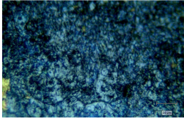
Figure 10.12: Optical micrograph of the WS_2/MoS_2 on Au substrate
