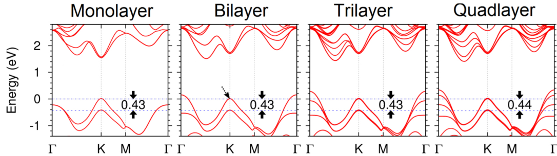
Figure 2.2: Band structures of 1,2,3 and 4 layer WS_2 , from ab initio calculations. Adopted from [4]
