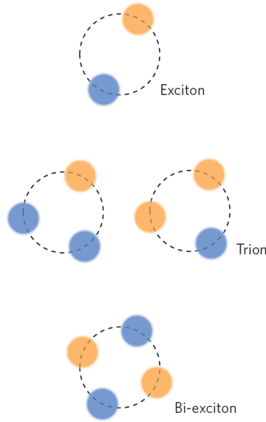
Figure 2.5: An exciton and other excitonic complexes: a neutral exciton, a trion and a bi-exciton. Reproduced from [26]
