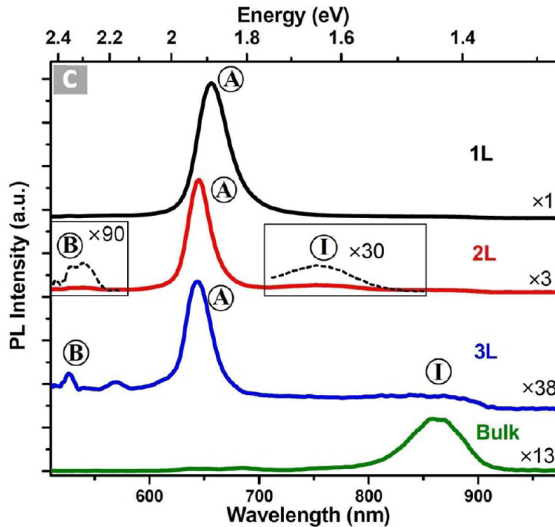
Figure 2.3: Typical PL spectrum of WS_2 showing the influence of the number of layers. Adopted from [8].
