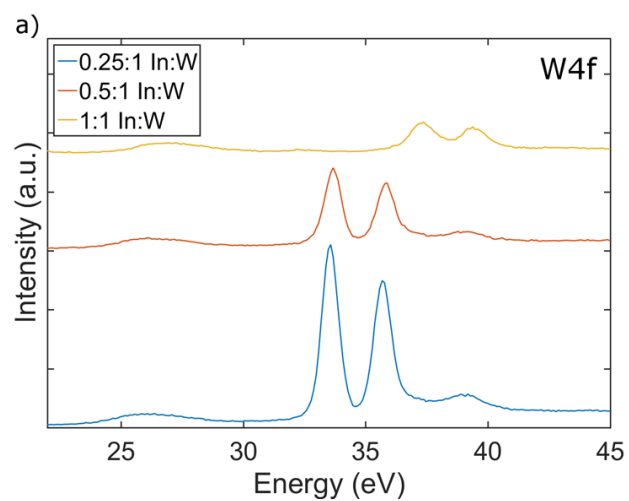
(a) W 4f
