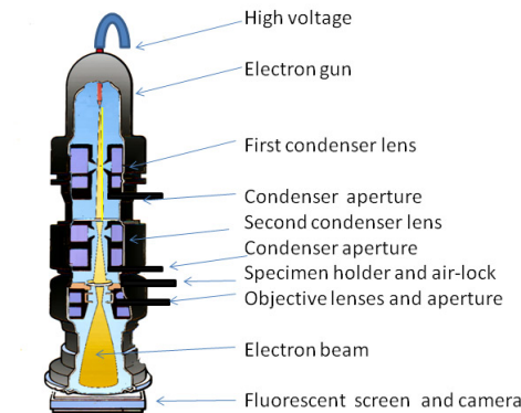
Figure 3.7: Crossection of a TEM column. Reproduced from ccber.ucsb.edu
