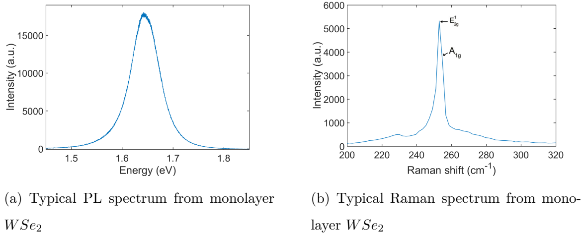
Figure 9.2: PL and Raman spectra from monolayer WSe_2
