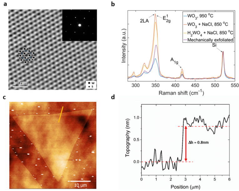
Figure 7.5: a) HRTEM image of WS_2 grown with H_2WO_4 + NaCl , inset shows a hexagonal diffraction pattern. b) Raman spectra taken from WS_2 grown various precursors with characteristic peaks indicated. c) AFM image and d) height profile of single layer WS_2 . Adopted from [147].
