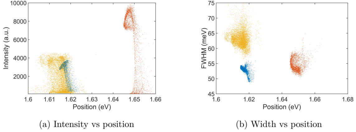
Figure 9.5: PL peak parameters distribution
