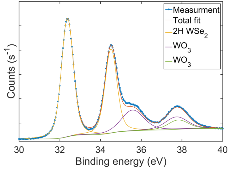
(a) W 4f
