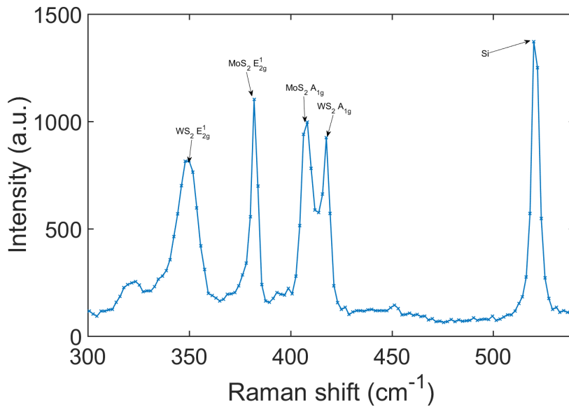
Figure 10.4: Raman spectrum of WS_2/MoS_2 heterobilayer
