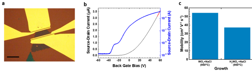
Figure 7.16: a) OM image of FET from bilayer \text{WS}_2 (scale bar is 30 \mu\text{m} ); (b) FET transfer curve taken from \text{WS}_2 made with \text{WO}_3 + \text{NaCl}/950^\circ\text{C} c) electron mobility of double layer sample made with different precursors. Adopted from [147].
