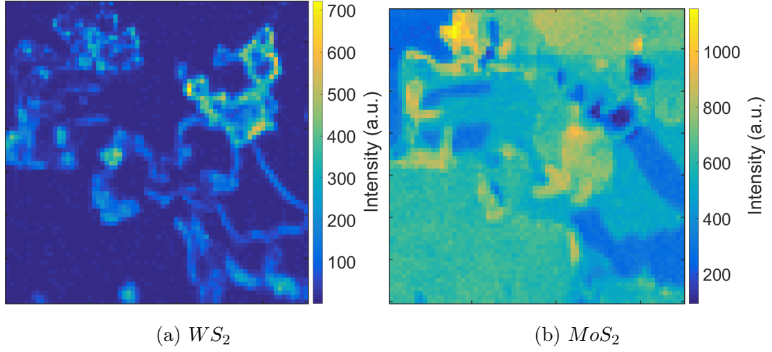
Figure 10.6: Map of Raman E_{2g}^1 peak intensity
