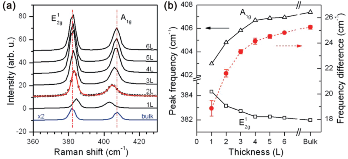
Figure 2.11: a) Raman spectra with of mono and few layers and bulk WS_2 with indicated characteristic peaks b) Characteristic Raman peak position and difference between them as a function of number of layers. Adopted from [51].
