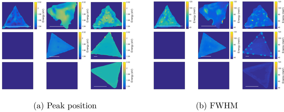
Figure 7.10: PL peak positions and FWHM maps. Adopted from [147].
