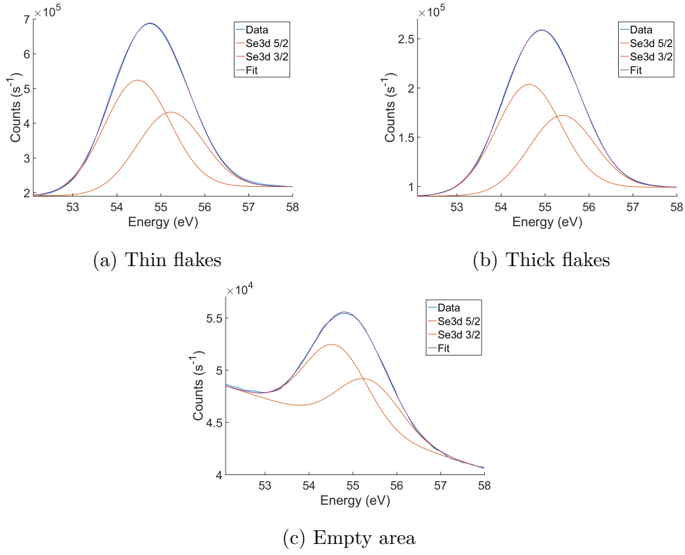
Figure 9.8: XPS spectra of Se3d peaks in different areas of the sample
