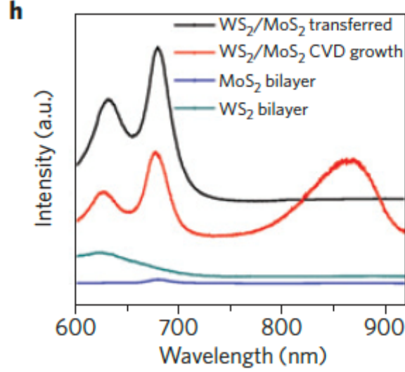
Figure 5.7: Comparison of PL spectra from hetero and homo bilayers of WS_2 and MoS_2 . Adopted from [92].
