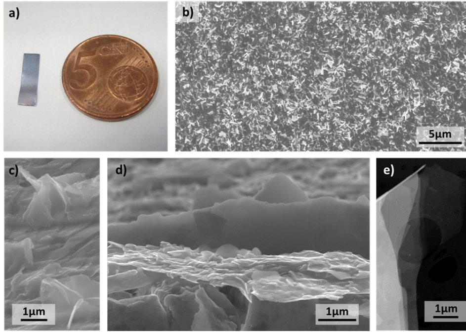
Figure 10.2: a) MoS_2/WS_2 heterobilayer on Au substrate b) SEM image of MoS_2/WS_2 heterobilayer on Au substrate c) side; d) cross-sectional SEM image e) STEM image of the flake edge. Adopted from [192].
