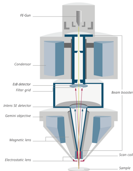
Figure 3.5: Cross section of the SEM optical column. Reproduced from zeiss.com
