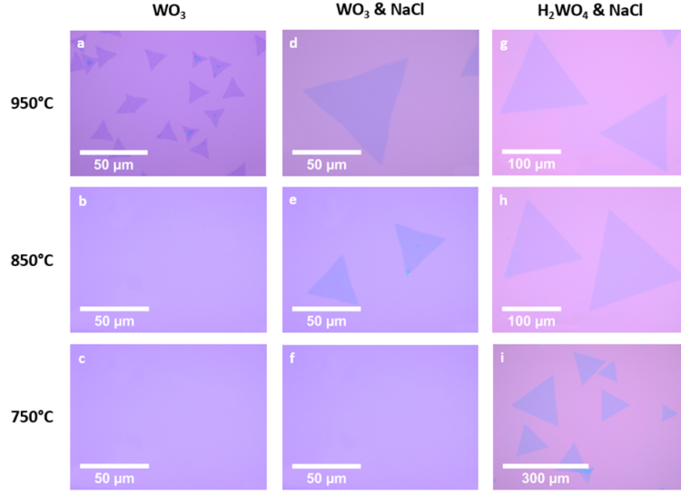
Figure 7.2: OM image of WS_2 . Adopted from [147].
