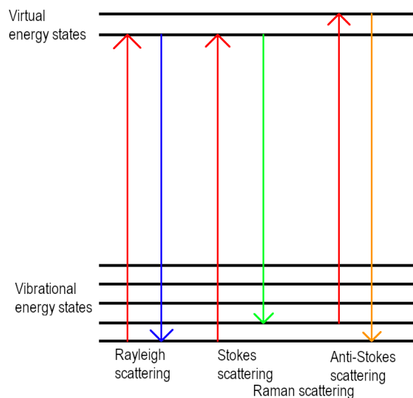
Figure 3.1: An energy diagram comparing elastic and inelastic scattering.
