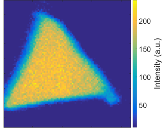
(a) Raman E_{2g}^1 intensity map of as-grown sample
