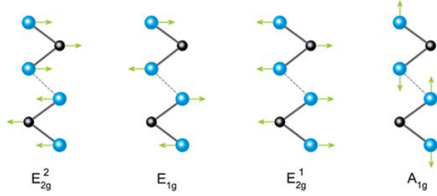
Figure 2.8: 4 active Raman modes in TMDCs. Metal atoms and chalcogen atoms are black and blue respectively. Adopted from [49]
