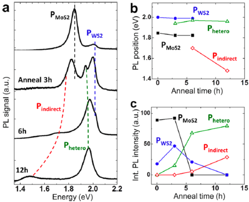
Figure 5.6: PL Spectrum of heterostructure after annealing. Adopted from [91].
