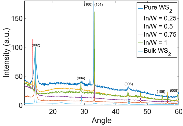
(a) XRD patterns for CVD-grown pure WS_2 and In-doped WS_2 .
