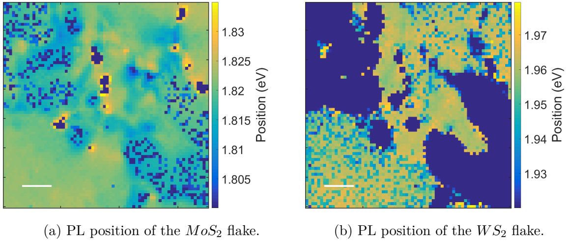
Figure 10.11: Map of PL peak positions. Scalebar is 10\mu m .
