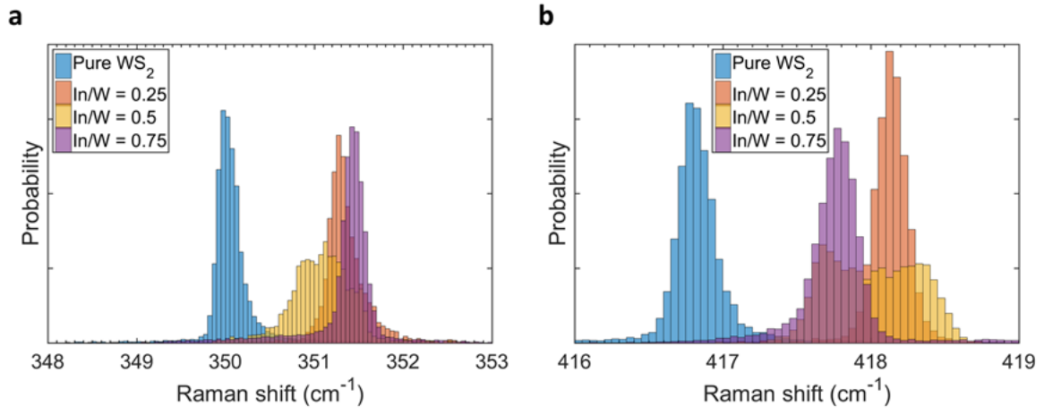
Figure 8.7: a) E_{2g}^1 and b) A_{1g} peak positions for pure WS_2 and Raman active In-doped WS_2 samples.
