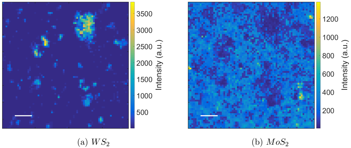
Figure 10.14: Raman E_{2g}^1 intensity maps. Scalebar is 10\mu m .
