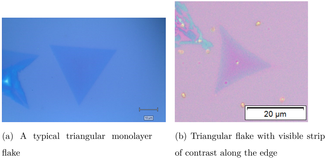
Figure 9.1: Optical micrographs of WSe_2 monolayer flakes
