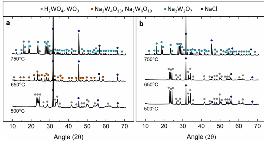
Figure 7.4: XRD spectra of residuals after annealing, a) H_2WO_4 + NaCl b) WO_3 + NaCl . Adopted from [147].
