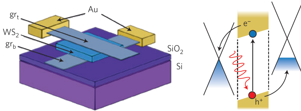
Figure 2.7: Left: \text{WS}_2 vertical photoconductor with graphene deposited on top ( \text{gr}_t ) and back ( \text{gr}_b ) electrodes. Right: Band diagram of a graphene/ \text{WS}_2 /graphene heterostructure with a built-in electric field. Reproduced from [26]
