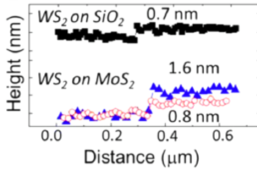
Figure 5.5: Comparison of AFM profiles of WS_2 on Si/SiO_2 and MoS_2 . Adopted from [91].
