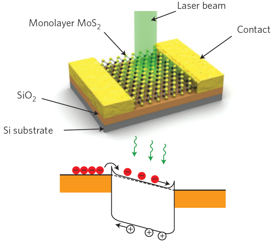
Figure 2.6: Top: Monolayer \text{MoS}_2 lateral photoconductor. Bottom: Band diagram of the monolayer \text{MoS}_2 photodetector. Reproduced from [26]
