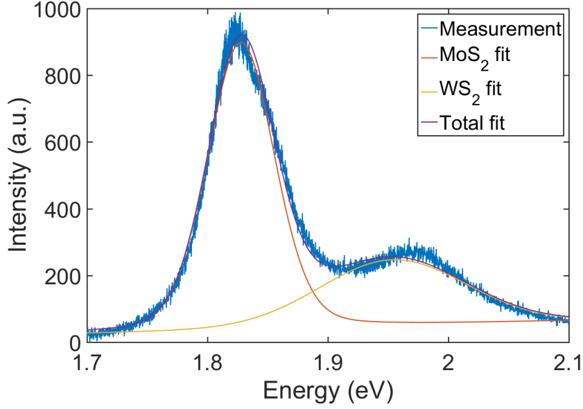
Figure 10.8: PL spectrum of MoS_2/WS_2 heterobilayer
