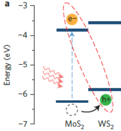
Figure 5.1: Charge separation across heterojunction following photoabsorption. Adopted from [89]
