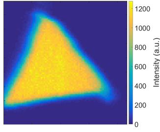
(a) Raman E_{2g}^1 intensity map of as-grown sample
