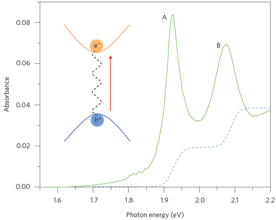
Figure 2.4: Absorption spectrum of monolayer MoS_2 at 10 K in green. A and B peaks correspond to two spin-split valence to the conduction bands transition. Blue dashed line - absorbance in absence of excitonic effects. Inset - Coulomb attraction between an optically generated electron-hole pair which forms a bound exciton. Reproduced from [26]
