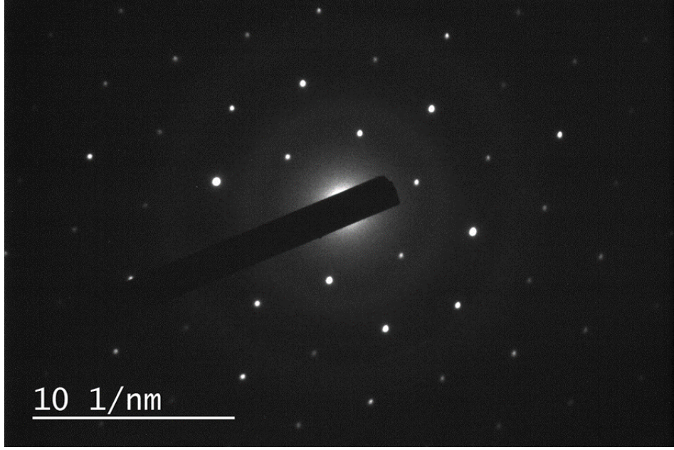
Figure 8.10: Electron diffraction pattern of WS_2 flake with In : W = 1 : 2
