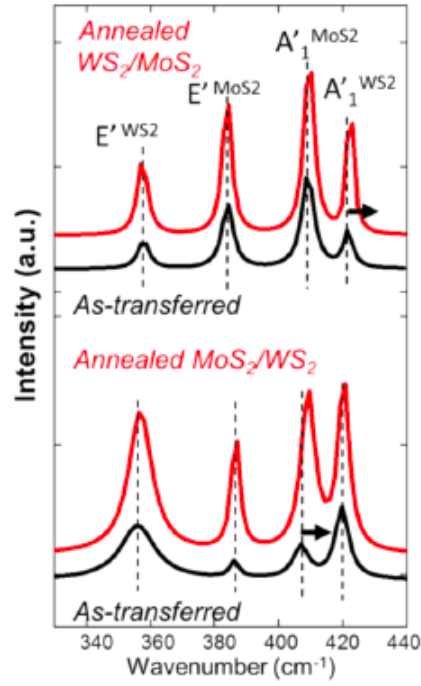
Figure 5.4: Heterostructure Raman spectrum. Adopted from [91].
