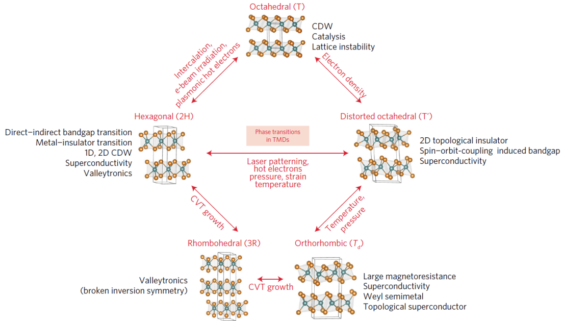
Figure 6.1: Transition and correlation between phase and physics in TMDCs. Reproduced from [110]
