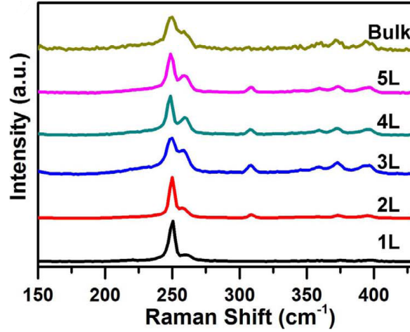
Figure 2.12: Raman spectra of mono and few-layer WSe_2 . Adopted from [53].
