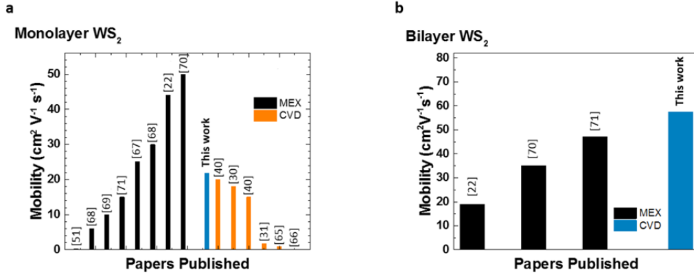
Figure 7.15: Comparison of electron mobility with literature for a) monolayer b) bilayer. Adopted from [147].
