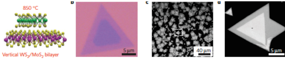
Figure 5.3: Heterostructure imaging. Adopted from [92].
