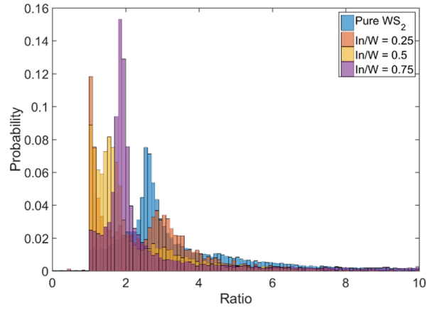
(a) Excitons-to-trions ratio for pure WS_2 and PL active In-doped WS_2 samples XPS
