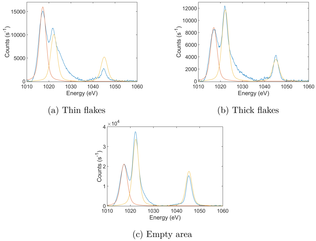
Figure 9.9: XPS spectra of Zn2p peaks in different areas of the sample
