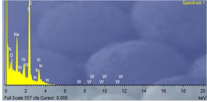
(a) Before transfer
