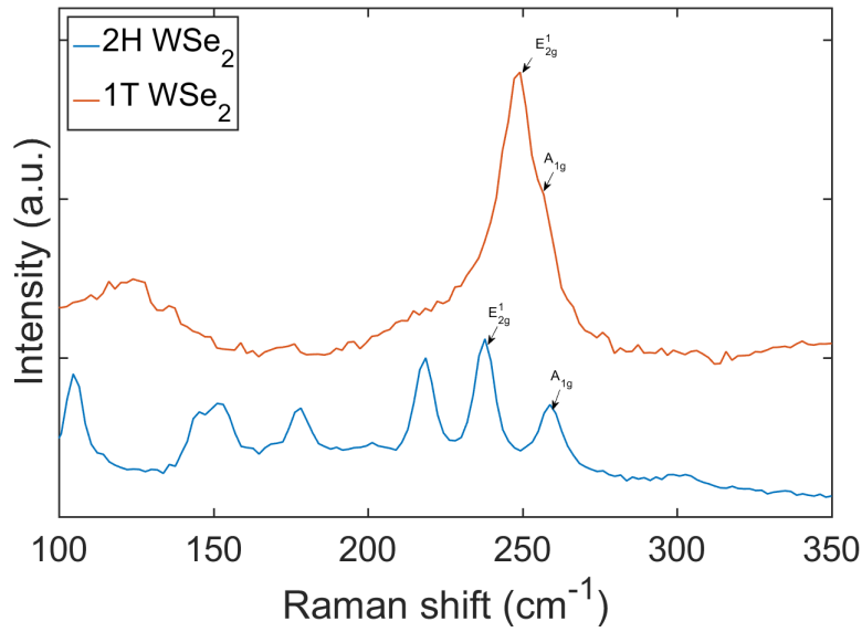
Figure 9.11: Raman spectra of 2H WSe_2 and 1T' WSe_2
