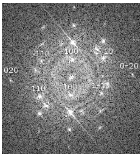
(c) FFT pattern constructed from the image in b).
