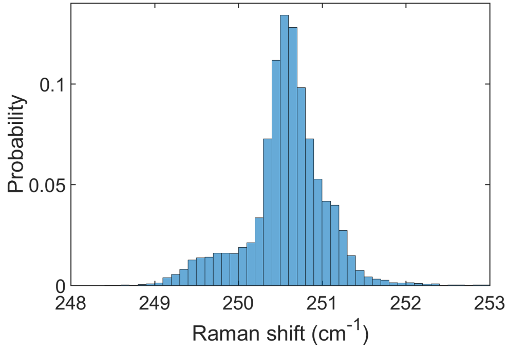
Figure 9.6: Histogram of Raman E_{2g}^1 peak position from monolayer WSe_2
