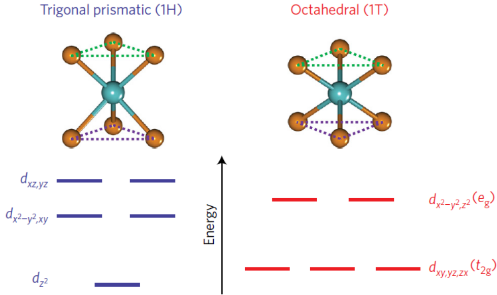
Figure 6.2: Diagrams of 1H and 1T lattices and energy levels of d-orbital electrons. Reproduced from [110].
