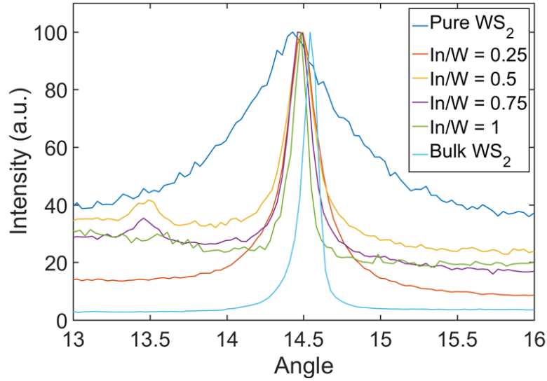
(b) (002) XRD peak for CVD-grown pure WS_2 and In-doped WS_2
