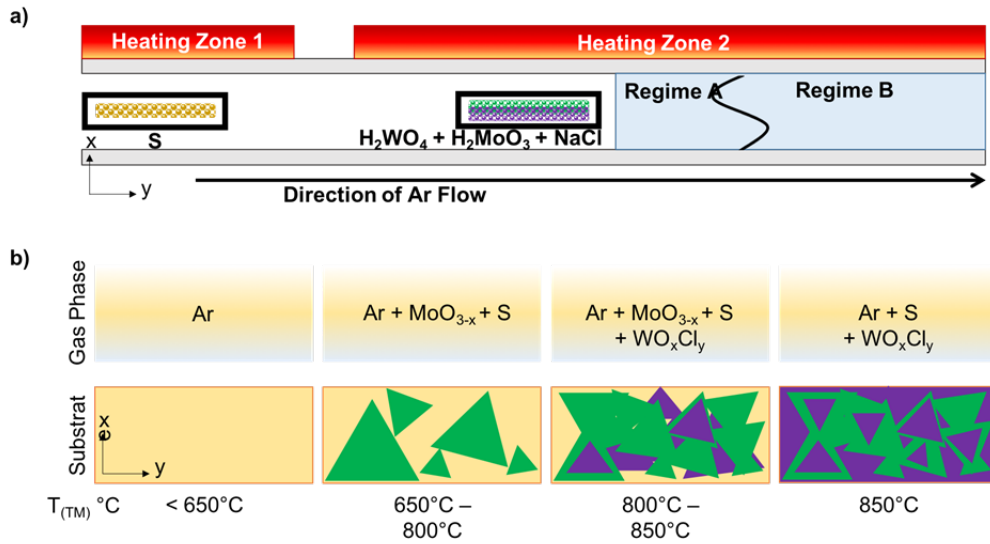
Figure 10.1: CVD furnace setup a) spatial distribution of precursors b) simplified representation of the growth result (green = Mo region; purple = W region).
