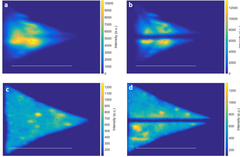
Figure 7.11: Maps of PL intensity a) before b) after performing the cut. Maps of 2LA + E_{2g}^1 Raman peak intensity c) before d) after performing the cut. Scale bar is 10 \mu\text{m} . Adopted from [147].
