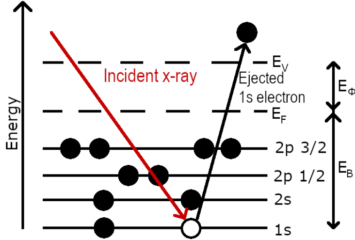
Figure 3.4: Photoelectron effect energy diagram present during XPS.
