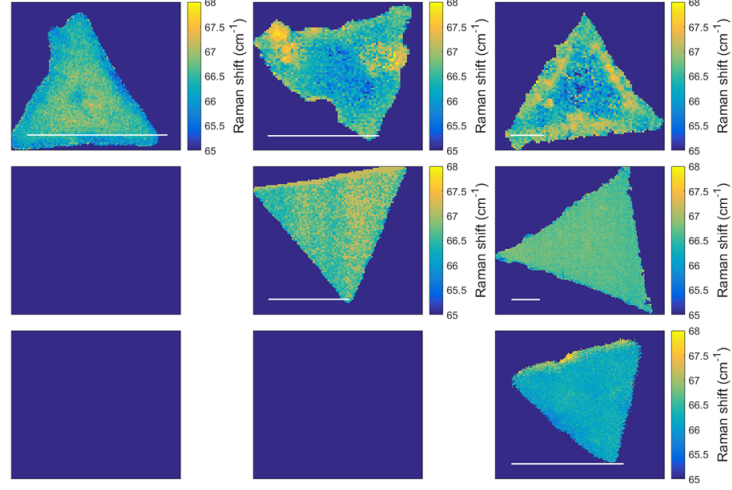
Figure 7.9: Raman peaks 2LA , A_{1g} positions difference. Scale bar is 10\ \mu\text{m} . Adopted from [147].
