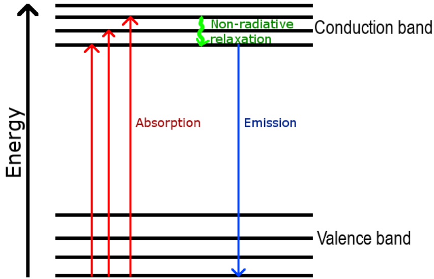
Figure 3.3: The photoluminescence process.
