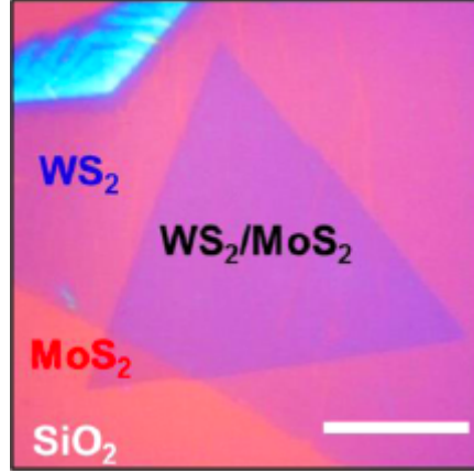
Figure 5.2: Optical micrograph of the heterostructure of WS_2/MoS_2 . Adopted from [91].
