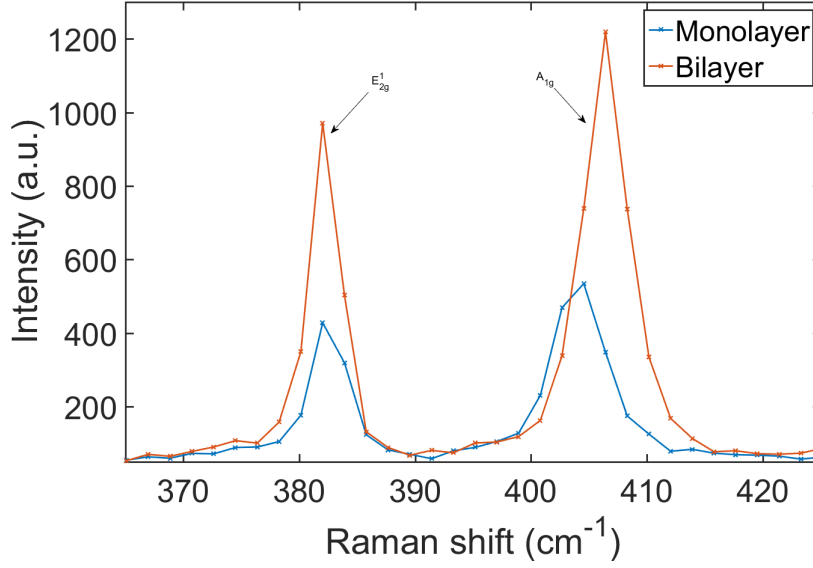
Figure 10.5: Raman spectra of mono and bilayer MoS_2
