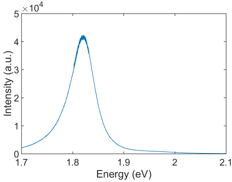
Figure 10.9: PL spectrum of MoS_2 monolayer
