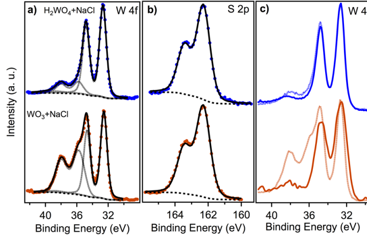
Figure 7.13: XPS spectra of the WS_2 samples. a) W 4f 5/2 , W 4f 7/2 , W 5p core levels of sample grown with H_2WO_4 + NaCl/950 °C (top), sample grown with WO_3 + NaCl/950 °C (bottom). Black dashed line - deconvolution of the peaks, black continuous line - total fit. (b) S 2p 1/2 , 2p 3/2 core levels for corresponding samples. (c) W 4f 5/2 , W 4f 7/2 , W 5p core levels taken from samples before (dashed line) and after (solid line) transfer. Adopted from [147].
