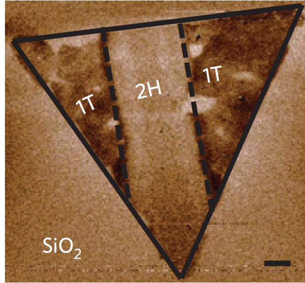
Figure 6.3: Electrostatic force microscopy phase image of a monolayered MoS_2 homo-junction. Reproduced from [106]
