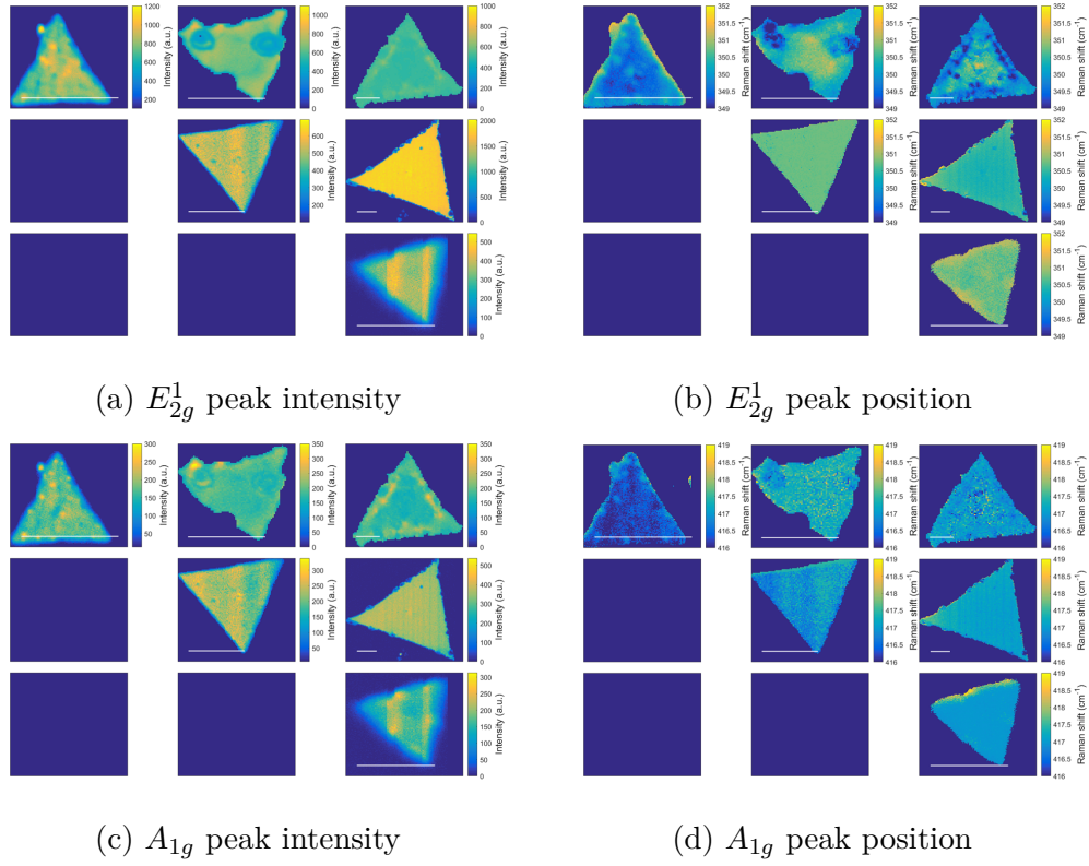
Figure 7.8: Raman peaks maps. Adopted from [147].
