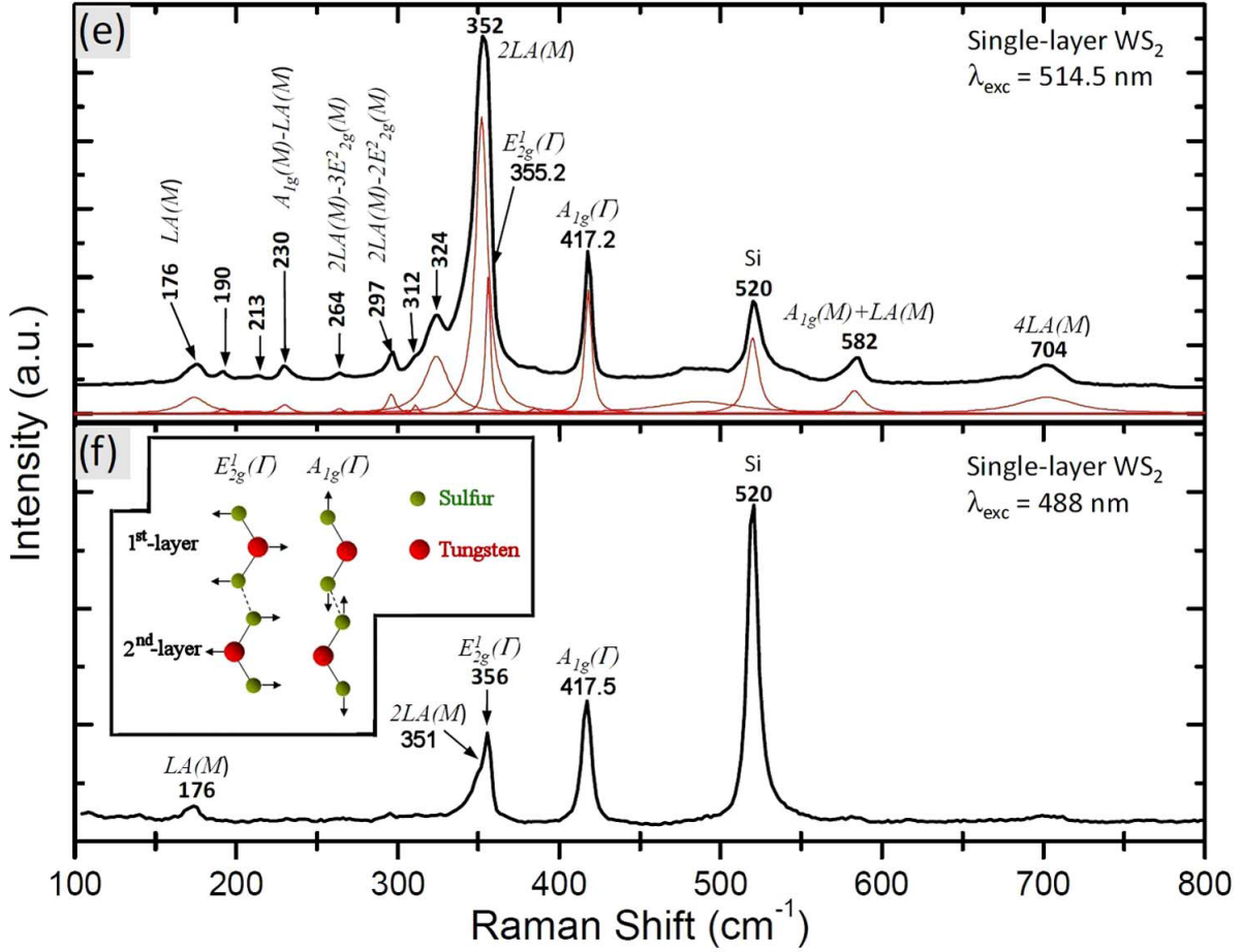
Figure 2.9: Raman spectrum of WS_2 with characteristic peaks indicated. Adopted from [50].
