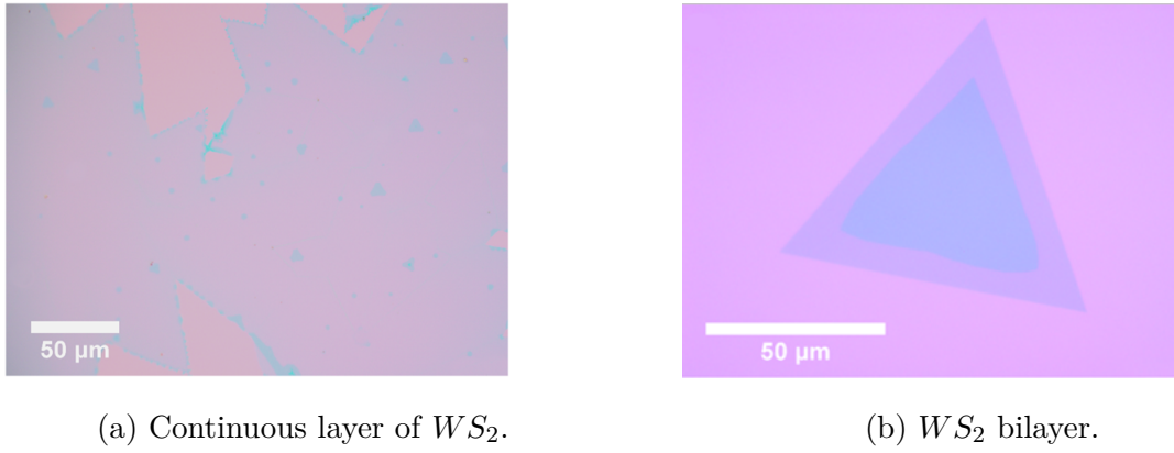
Figure 7.3: OM Images of WS_2 . Adopted from [147].
