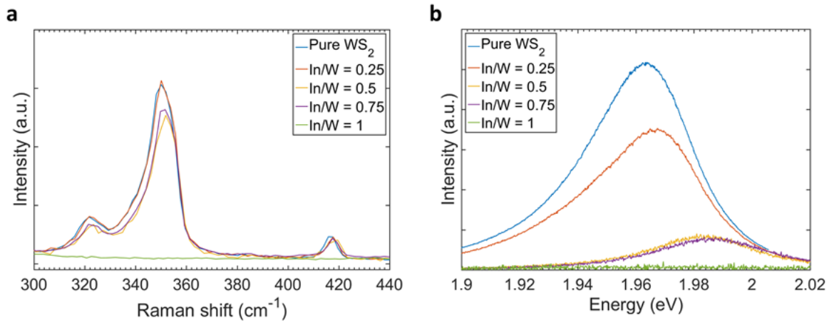
Figure 8.4: Representative a) Raman and b) PL spectra for pure WS_2 (grown by using H_2WO_4 as metal precursor) and In-doped WS_2
