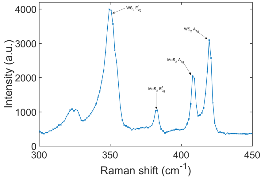
Figure 10.13: Raman spectrum of WS_2/MoS_2 on Au substrate
