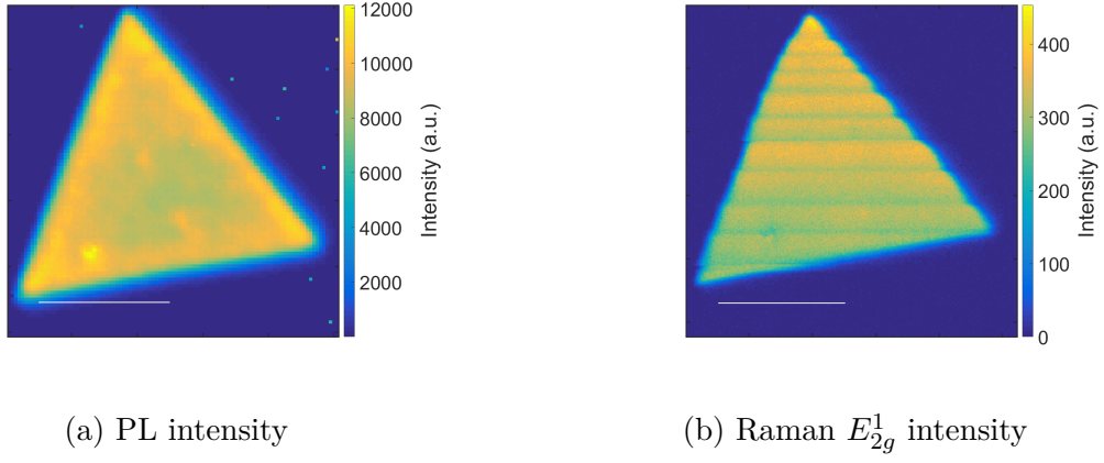
Figure 9.3: PL intensity and Raman E_{2g}^1 intensity maps
