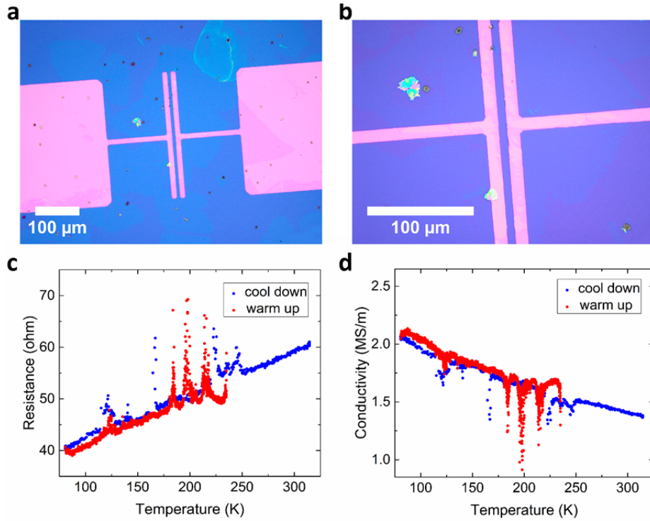
Figure 8.6: (a, b) Optical micrographs of Ti and Au contacts deposited on In/W=1 flakes. (c) Measured resistance as a function of temperature. (d) Calculated conductivity vs. temperature revealing a semi-metallic behaviour.
