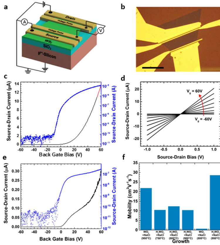
Figure 7.14: a) FET diagram; b) OM image of the FET (scale bar is 20 μm); c) FET transfer curve taken from the single layer sample made with H_2WO_4 + NaCl/950 °C; d) I-V curves taken at different gate biases for sample made with H_2WO_4 + NaCl ; e) FET transfer curve taken for single layer sample made with WO_3 + NaCl/800 °C; (f) comparison of electron mobilities of single layer WS_2 made with different precursors. Adopted from [147].
