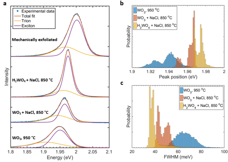
Figure 7.7: a) WS_2 PL spectra grown using various precursors b) histograms of PL peak positions c) histograms of PL peak widths. Adopted from [147].
