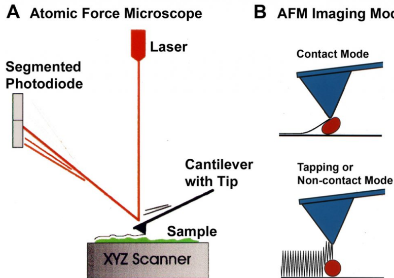
Figure 3.6: Diagram of AFM setup and operating basics. Reproduced from ccem.mcmaster.ca
