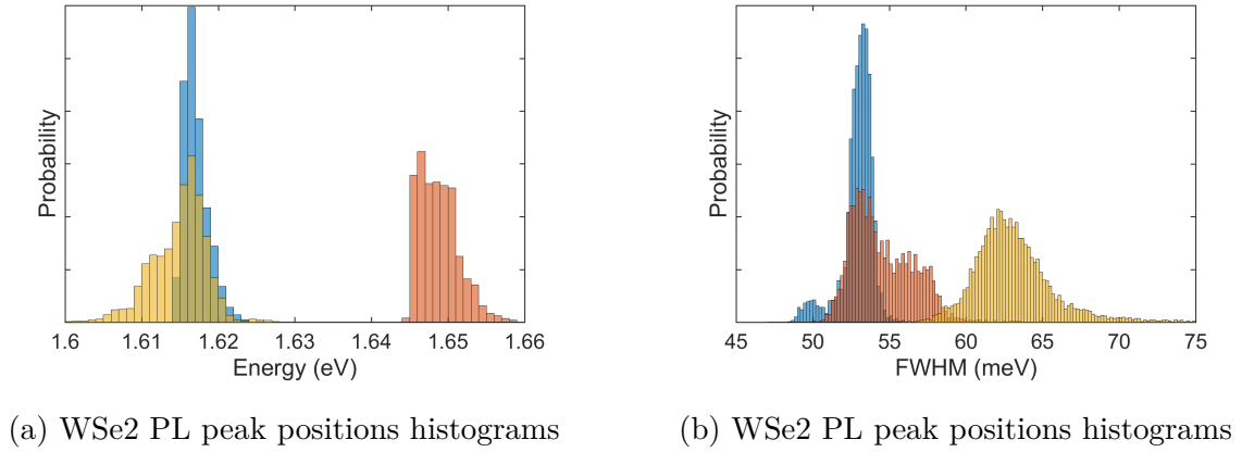
Figure 9.4: Comparison of PL peak positions and widths in different WSe_2 samples. Different colour correspond to separate growths.
