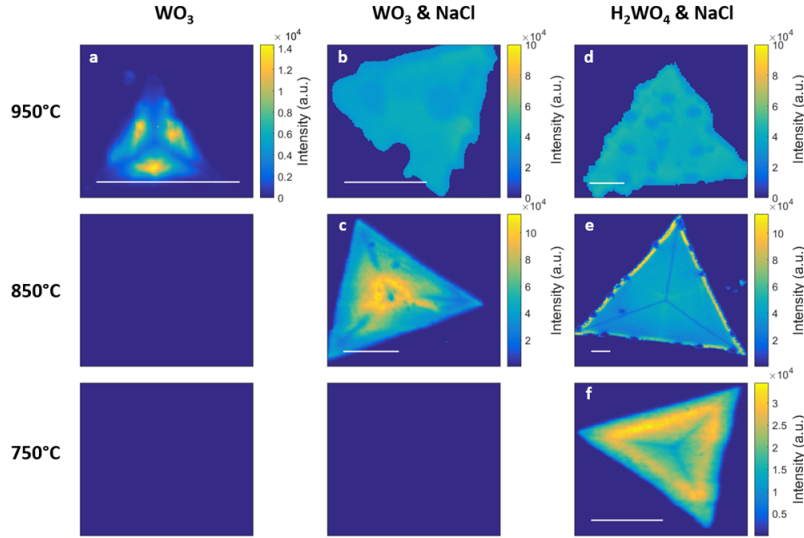
Figure 7.6: Maps of WS_2 PL intensity. The scale bar is 10\mu m . Adopted from [147].
