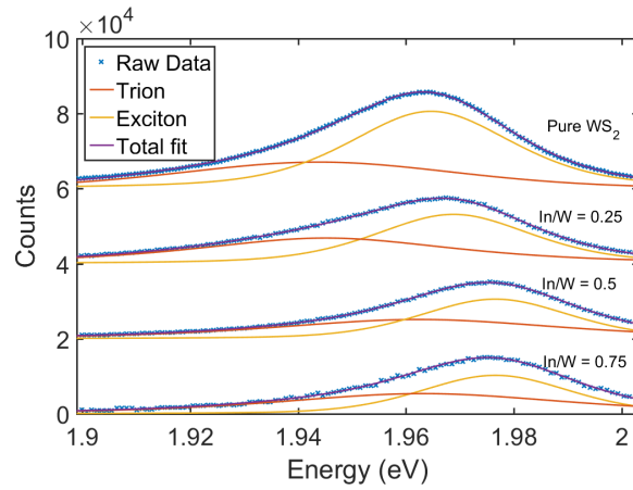
(b) PL spectra from samples of different In/W precursor ratio.
