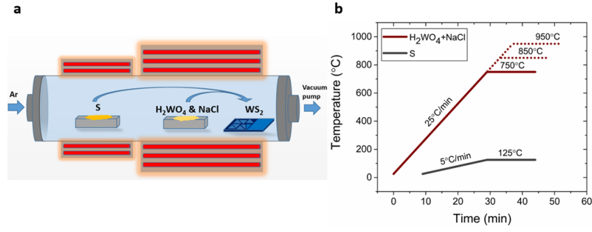
Figure 7.1: a) CVD furnace setup; b) Temperature profiles for the W and S precursors. Adopted from [147]
