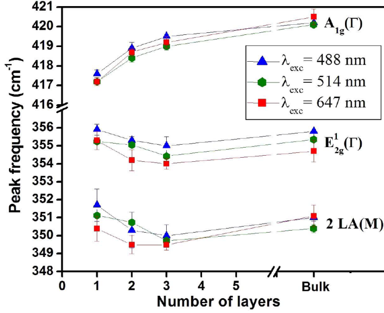
Figure 2.10: Identification of number of layers by the difference in position of A_{1g} and E_{2g}^1 peaks. Adopted from [50].
