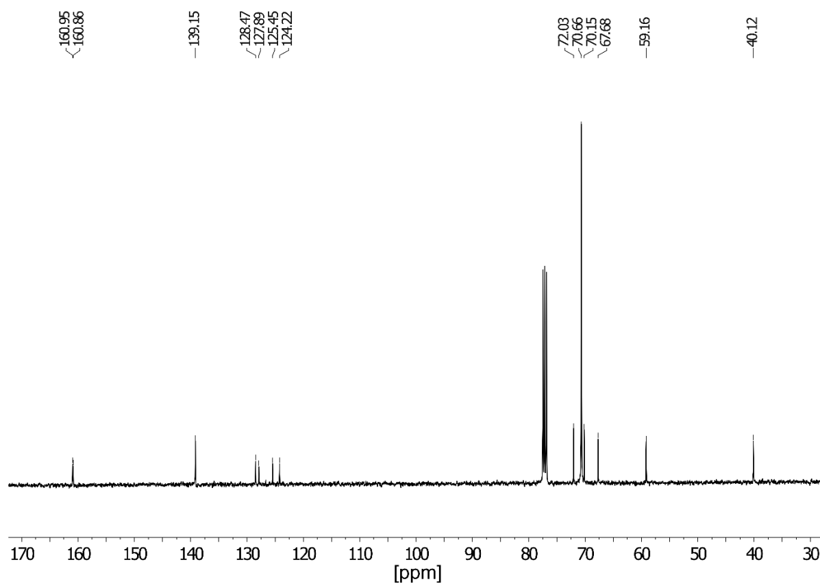
Figure S6: 1 H NMR and 13 C NMR spectra of g7-NDI-Br 2 measured in CDCl 3 .
