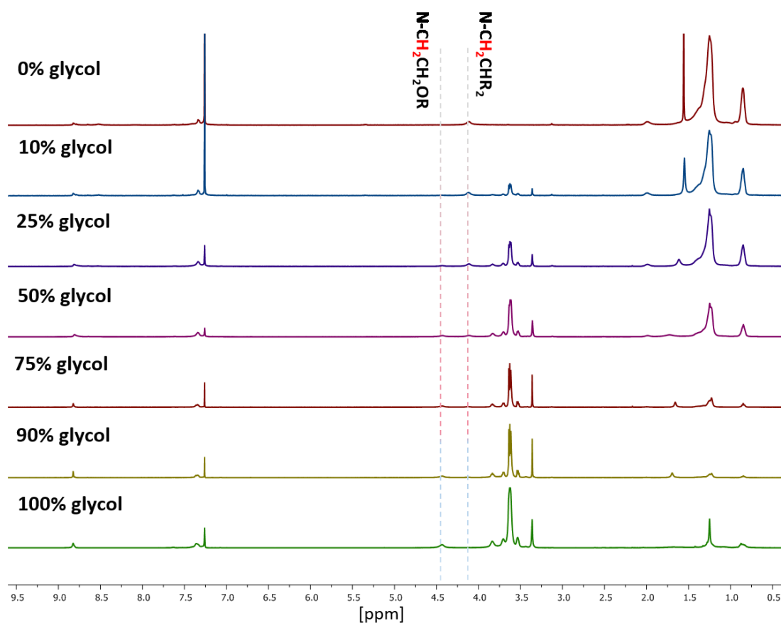
Figure S15: ^1\text{H} -NMR spectra of the copolymers measured in \text{CDCl}_3 .
