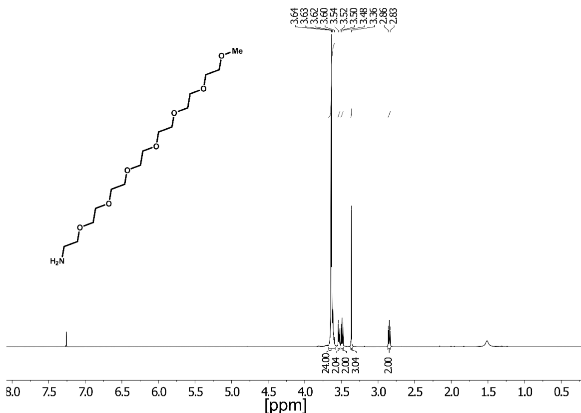
Figure S4: ^1\text{H} NMR of 2,5,8,11,14,17,20-heptaoxidocosan-22-amine measured in \text{CDCl}_3 .
