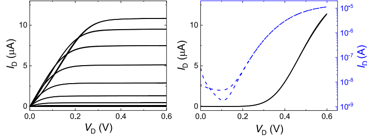
Figure S28: Thickness scaling for OECT performance. P-90 OECT with the same areal dimensions ( 100 \times 10 \mu\text{m} ), as spin cast devices above, with a thickness of 1015nm. This OECT yields a peak transconductance, g_m , of 47 \mu\text{S} .
