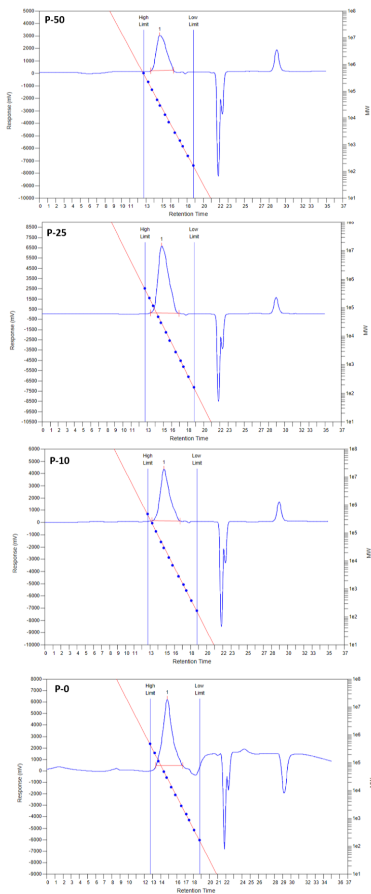
Figure S18: GPC measurements of the polymer P-50 to P-0 in chlorobenzene (no observation of a bimodale elution).
