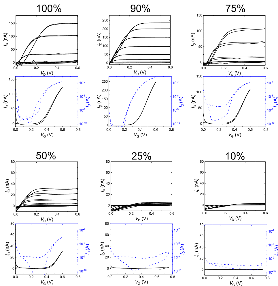
Figure S27: Organic electrochemical transistor measurements for P-10 , P-25 , P-50 , P-75 , P-90 and P-100 . For each polymer, the output ( I_D - V_D ) and transfer ( I_D - V_G ; linear, black solid line, log scale, blue dotted line) plots are shown. All OECTs measured were nominally 100 \times 10 \mu\text{m} ( W \times L ), with thicknesses of 28 nm ( P-100 ), 52 nm ( P-90 ), 39 nm ( P-75 ), 31 nm ( P-50 ), 32 nm ( P-25 ), and 41 nm ( P-10 ). P-0 did not show OECT operation, or any indications of turn on over the bias range probed. The non-idealities typically observed for NDI copolymers with polar side chains ( P-50 to P-100 as well as p(gNDI-gT2) 2 ) are often associated with voltages that lead to irreversible degradation, and are the topic of ongoing investigation. The typical operation voltages (peak g_m ), are at stable potentials.
