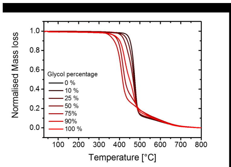
Figure S23: TGA of the copolymers.
