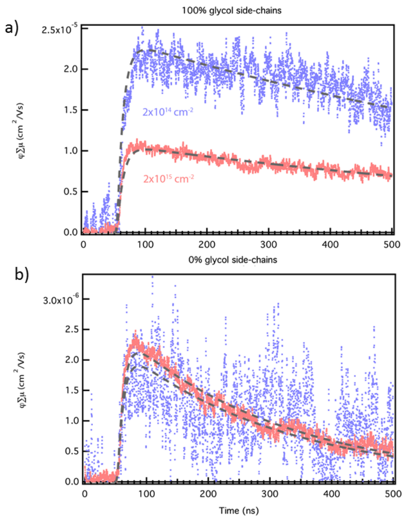
Figure S31: Example microwave photoconductance transients for thin films of P-100 : (a) and P-0 (b) glycol side-chain fraction. The red traces show the results for excitation with 2 × 10 15 cm -2 and the blue for 2 × 10 14 cm -2 . The gray dashed traces show the single-exponential fits used to calculate the data points in Figure S28.
