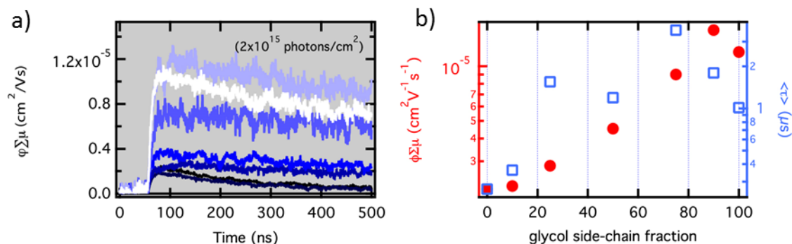
Figure S30: (a) Microwave photoconductance transients measured with 700 nm excitation at 2 \times 10^{15} photons/cm 2 . The left axis is an expression of the fluence-normalized photoconductance, the product of carrier yield and the sum of microwave-frequency mobility contributions. (b) The initial magnitude (red circles, left axis) and single-exponential lifetime (blue squares, right axis) as a function of glycol side-chain fraction (%). These values were extracted from single-exponential fits to each transient, and averaged across the measured intensity range ( 2 \times 10^{14} - 2 \times 10^{15} cm -2 ) as there was little variation in either property as a function of intensity.
