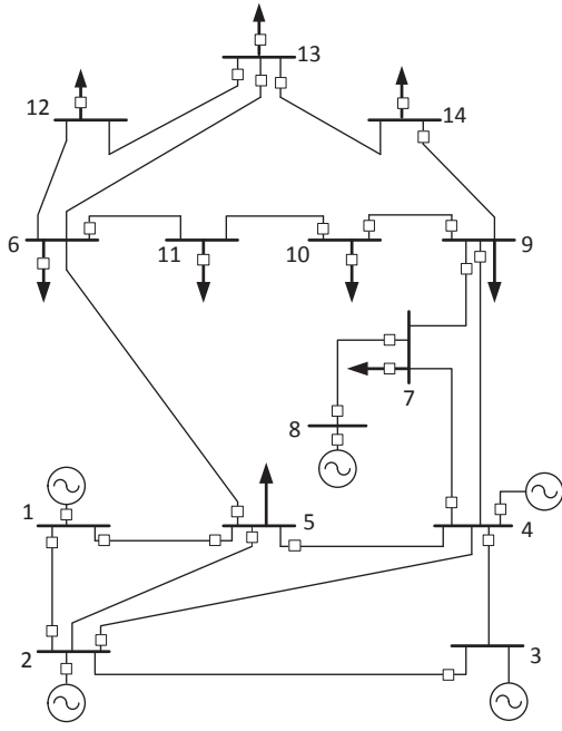
Fig. 6. IEEE-14 bus system
