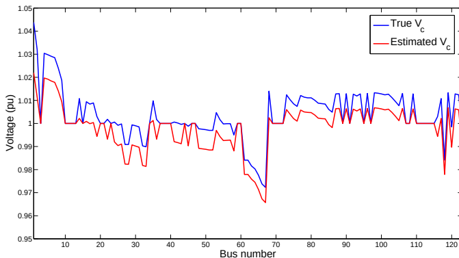
Fig. 15. True and estimated voltages of phase c for IEEE 123 bus system
