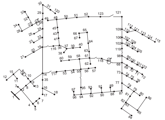
Fig. 7. IEEE 123-bus distribution system
