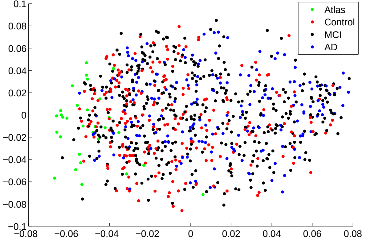
Figure 4.10: First two embedding coordinate for 796 ADNI images together with 30 manually labeled atlas images obtained from applying a spectral embedding step to pairwise similarities evaluated over the whole brain after an affine normalization to a template space.
