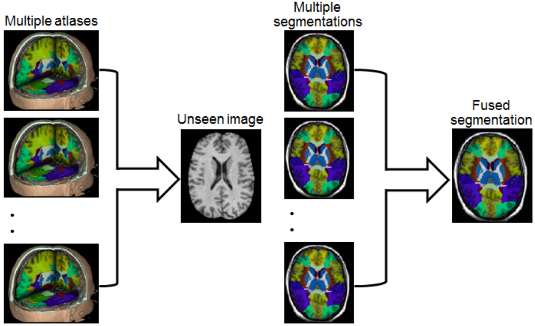
Figure 2.3: Multi-atlas brain segmentation. Multiple atlas images are registered with the unseen images and all atlas labels are propagated to the target. The final segmentation is obtained from fusing the individual segmentations.
