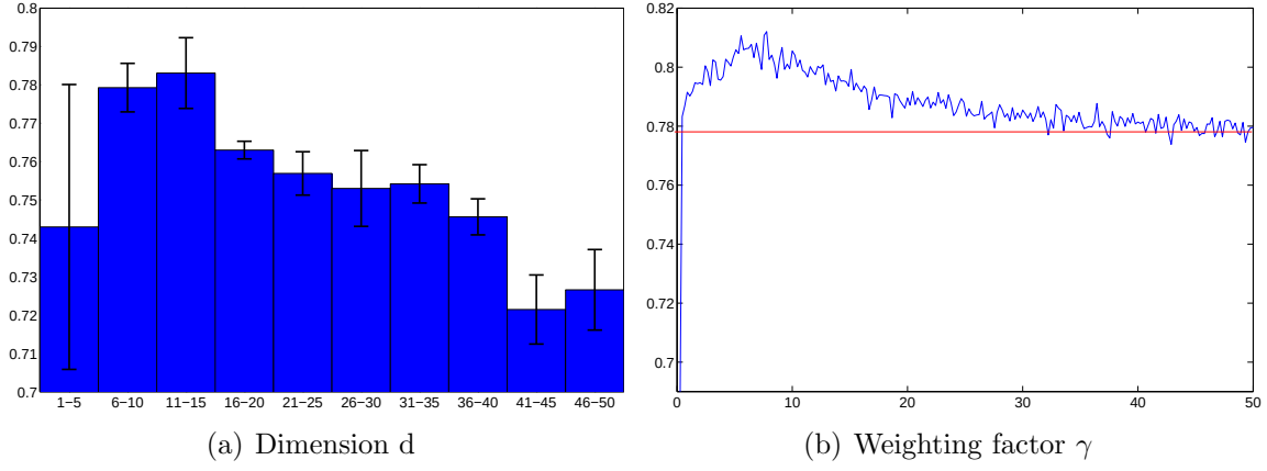
Figure 6.5: (a): Classification rate in the training data set when varying the dimension of the low-dimensional manifold between 1 and 50. Results are presented as mean rates over ten bins covering five dimensions each. The high standard deviation observed in the first bin results from a very low classification rate with d=1 . (b): Classification rate when varying \gamma between 1 and 50 evaluated for d \in [6, 15] .
