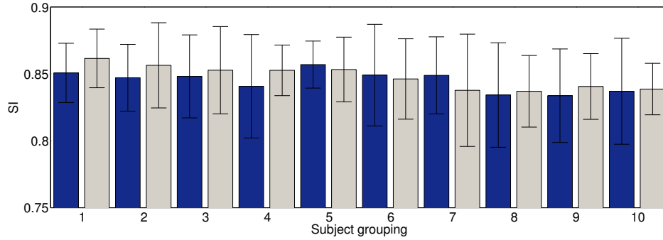
Figure 4.12: Label overlaps (SI) for automated hippocampus segmentation with semi-automated reference segmentations. Compared are segmentations obtained with LEAP when using a similarity measure over the whole brain (blue) to a similarity measure defined in a region around the hippocampus (grey). Results for both approaches are represented for 10 groups of subjects as described before for Figure 4.7.
