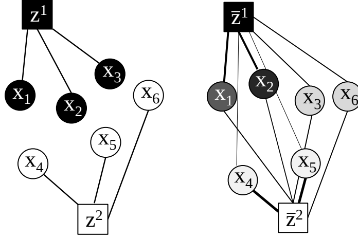
Figure 6.1: Weights defined between image nodes \mathbf{x}_i and support nodes representing metadata Z . In the discrete setting (left), equally weighted edges are defined according to Equation 6.5. In the continuous setting (right), weights to both additional nodes are defined according to Equations 6.6 and 6.7. A higher weight is illustrated by a thicker edge.
