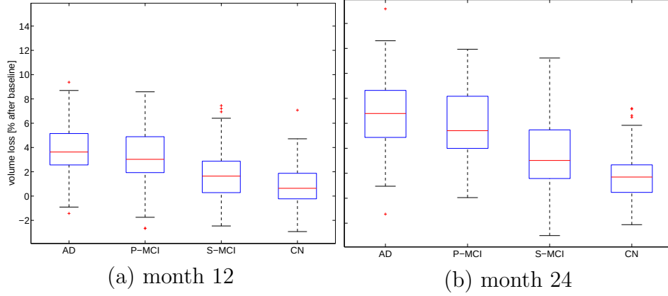
Figure 5.3: Hippocampal volume loss in % from baseline after 12 and 24 months. Box-and whisker plots for AD, P-MCI, S-MCI, CN.
