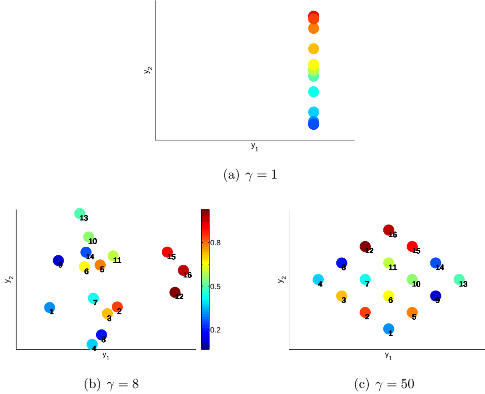
Figure 6.2: First two embedding coordinates with varying influence of \gamma . A high weight leads to an embedding similar to the one obtained with classic Laplacian eigenmaps (c). A very low weight embeds the images mainly based on metadata (a).
