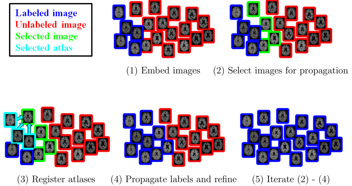
Figure 4.2: Process of atlas propagation with LEAP. All labeled (atlases) and unlabeled images are embedded into a low-dimensional manifold (1). The N closest unlabeled images to the labeled images are selected for segmentation (2). The M closest labeled images are registered to each of the selected images (an example for one image is shown in (3)). Intensity refinement is used to obtain label maps for each of the selected images (4). Steps (2) - (4) are iterated until all images are labeled.
