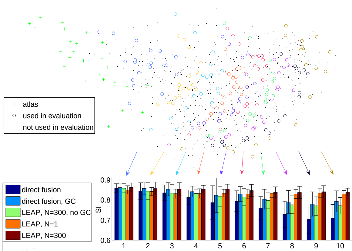
Figure 4.7: Development of segmentation accuracy with increasing distance from the original set of atlases. Each subset of images used for evaluation is represented by one bar plot.
