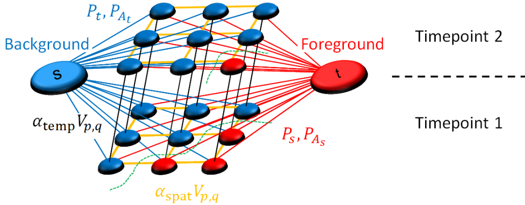
Figure 5.1: 4D graph cut segmentation: images acquired at two timepoints are connected by additional smoothness constraints (black edges) when compared to a 3D graph cut model.
