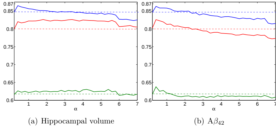
Figure 6.6: Classification accuracy obtained from defining a combined similarity measure incorporating both imaging and non-imaging information before performing manifold learning. AD vs CN: blue; S-MCI vs P-MCI: green; CN vs P-MCI: red. Results with hippocampal volume and A\beta_{42} are presented over an increasing influence of the metadata. The dotted lines indicate the classification accuracy obtained with image similarities only.
