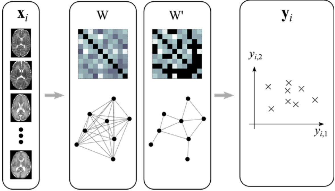
Figure 2.4: In the schematic illustration above, the images \mathbf{x}_i , 1 \leq i \leq N (left) are compared in pairs and measures of similarity or distance between them are obtained. The measures define a N \times N matrix representing the edge weights in a graph representation of the data. The graph/matrix representation may be either full (dense, \mathbf{W} above) or sparse ( \mathbf{W}' ), illustrations of both cases are shown above. Typically, the eigenvalue-eigenvector structure of the matrix (or of a matrix derived from it) is used to derive a coordinate representation for an embedded manifold representation \mathbf{y}_i of the original data. The first two dimensions of \mathbf{y}_i are schematically shown above.
