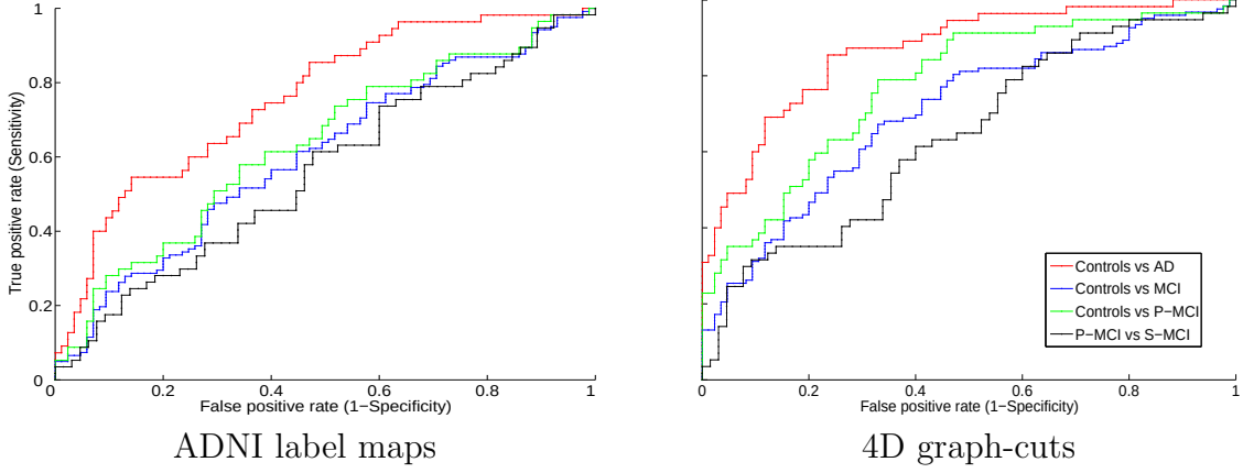
Figure 5.6: ROC curves show the discrimination between subject groups. The area under the curve AUC for (ADNI labels/4D graph-cuts) Controls vs AD, Controls vs MCI, Controls vs P-MCI and P-MCI vs S-MCI are 0.76/0.87, 0.60/0.70, 0.63/0.77, and 0.58/0.66, respectively.
