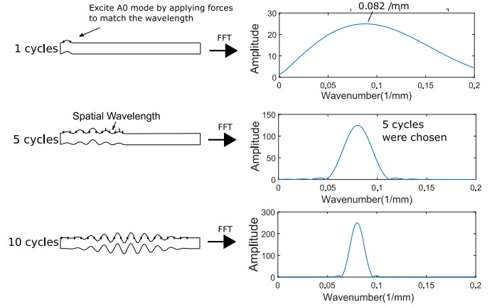
Fig. 5. Spatial variation and FFT for the excitation force for one-, five-, and ten-cycle Hanning windowed tone bursts centered at 0.082 1/mm.
