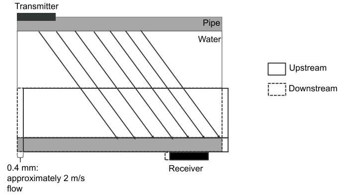
Fig. 13. Movement of the lower part of the model to simulate the flow and shifting the location at which the wave packet arrives on the other side of the pipe.
