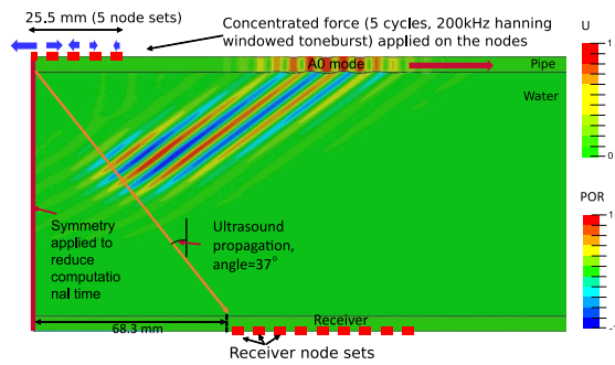
Fig. 7. FE model setup in Abaqus, showing the stress wave in the steel pipe and the pressure wave in the water, 46 \mu s after the transducer emits the signal. The propagation angle in water is calculated using Snell's law. Legend bar shows the arbitrary color scale of both the magnitude of the displacement (U) in the steel pipe and the acoustic pressure (POR) in water.
