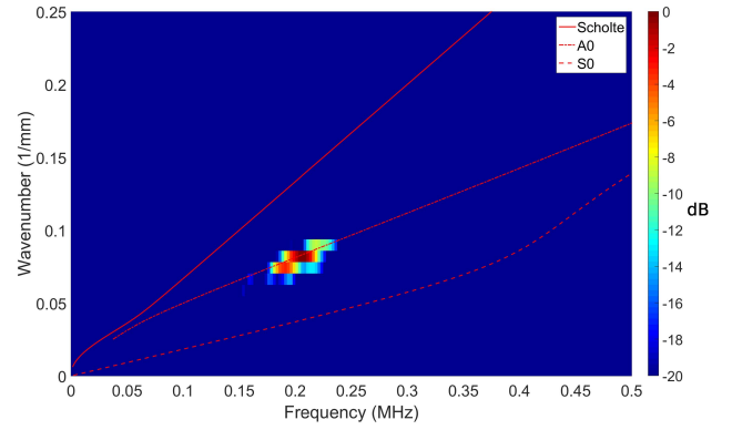
Fig. 21. 2-D FFT results displaying the wavenumber-frequency relationship of the signals. The Dispersion curve for the 5.74-mm thickness plate is also shown.
