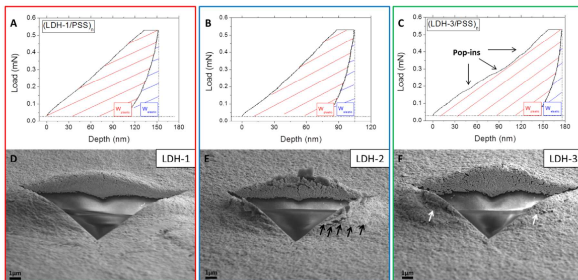
Figure 3. Mechanical properties of (LDH/PSS) n coating via nanoindentation. Load-displacement curves obtained from shallow nanoindentation of ~1.5 \mu\text{m} -thick (LDH/PSS) n coatings containing LDH-1 (A), LDH-2 (B), and LDH-3 (C) platelets. SEM side view micrographs of in-situ indents made on (LDH-1/PSS) n (D), (LDH-2/PSS) n (E) and (LDH-3/PSS) n (F) ~1.5 \mu\text{m} -thick coating at a depth of 10 \mu\text{m} (black arrows indicate multiple and subsequent displacement of materials while white arrows point coating failures within the pileups).
