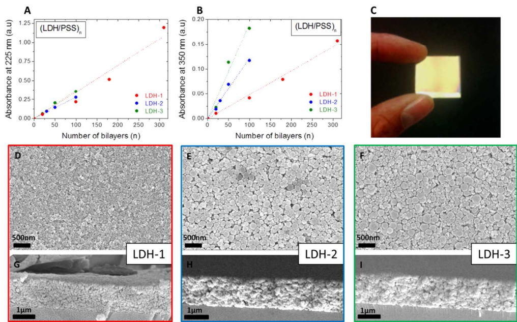
Figure 1. Layer-by-Layer assembly of (LDH/PSS) n multilayer coatings with different inorganic platelets dimensions and size distribution leading to varying organic content. Layer-by-Layer assembly of (LDH/PSS) n coatings monitored by UV-Vis absorbance values at 225 nm (PSS absorption) and 350 nm (scattering) from deconvoluted UV-Vis spectra (A and B, respectively). Photograph of μm-thick (LDH-2/PSS) 50 coating deposited on glass slide with high uniformity (C). SEM top and cross section images of (LDH-1/PSS) 155 (D and G), (LDH-2/PSS) 50 (E and H) and (LDH-3/PSS) 50 (F and I) -LDH terminated coatings.
