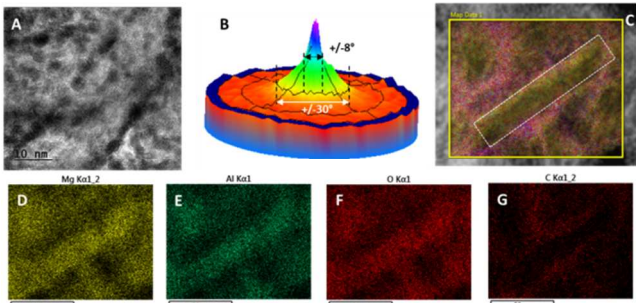
Figure 2. “Brick-and-mortar” (LDH/PSS) n nanostructures. TEM image of (LDH-2/PSS) n cross section (A). Three-dimensional rocking curves of (LDH-2/PSS) n coating (B) acquired for 2\theta=11.7^\circ , \Psi=[0;80^\circ] (graph step: 30^\circ ) and \Phi=[0;360^\circ] (graph step: 90^\circ ). EDX mapping acquired during TEM cross-sectional imaging of (LDH-2/PSS) 50 nanostructure (C), with Mg, Al, O and C atom distributions (D, E, F and G, respectively).
