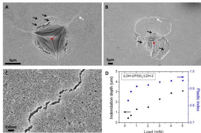
Figure 4. Ductile behaviour of (LDH/PSS) n coatings. Top view SEM images of indents made with a Berkovich tip into 1.5 μm-thick (LDH-2/PSS) n and (LDH-3/PSS) n (A and B, respectively) coatings at a depth of 5 μm (indents center are marked in red - black arrows evidence displacement of material within the pileups, while white arrows show cracks propagating from the indent). Top view SEM image show a crack propagating in (LDH-2/PSS) n coating (C). The plastic index of (LDH-2/PSS) n coating was measured from nanoindentation carried out at varying loads and depth (D).
