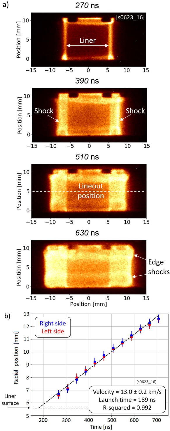
Fig. 4. (a) Optical self-emission images from the shot shown in Fig. 3(a). The liner is seen as the dark region in the center while the shocks expand radially and can be seen as regions of bright emission. (b) Shock front position plotted as a function of time. A linear trend line, shown with a dashed line closely fits the data allowing the velocity to be determined.
