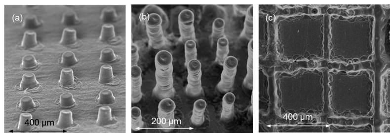
Fig. 18 (a) 50 and (b) 180 layers of YSZ printed to fabricate micro-pillar arrays; (c) a YSZ square lattice printed onto a NiO-YSZ substrate. Reproduced with permission. 31
