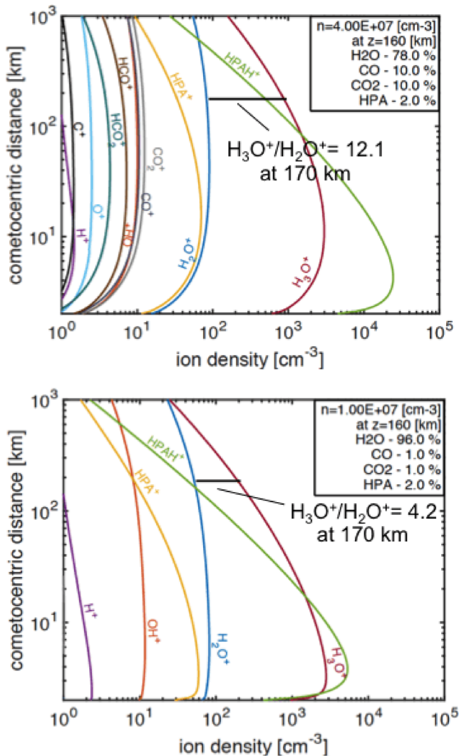
Figure 10. (Top) Same as Fig. 9 bottom, but with a different composition for the coma, 78 per cent ( \text{H}_2\text{O} ), 2 per cent (HPA), 10 per cent ( \text{CO} ), and 10 per cent ( \text{CO}_2 ). (Bottom) Same as Fig. 9 top but with a neutral outflow bulk velocity of 1000 \text{ m s}^{-1} . The composition change had a small effect on the \text{H}_3\text{O}^+/\text{H}_2\text{O}^+ ratio compared to the increase in the outflow bulk velocity.
