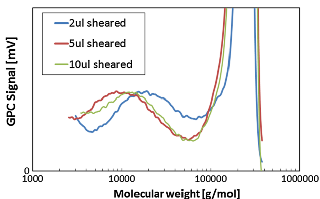
Fig. 13 Magnified scale from GPCs in Fig. 11 showing degraded PS peak
