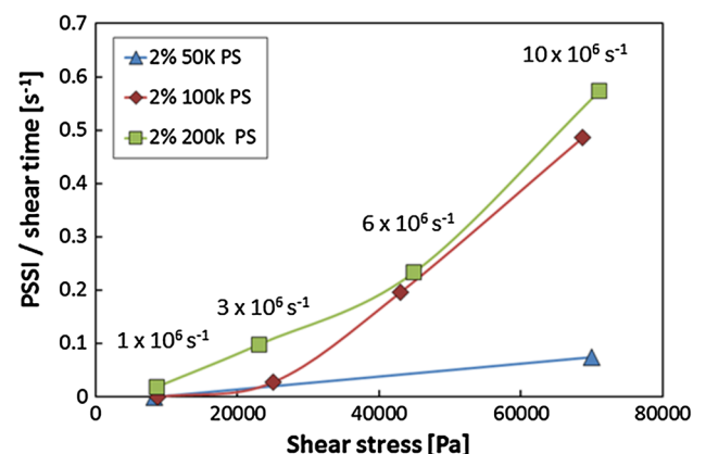
Fig. 10 Dependence of PSSI( 10^6 ) rate of change on shear stress for three different MWt 2 wt% PS solutions in DEHP at 80 °C
