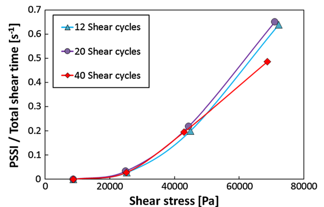
Fig. 9 Dependence of PSSI( 10^6 ) rate of change on shear stress after different shear times for 2 wt% 100 k PS in DEHP at 80 °C
