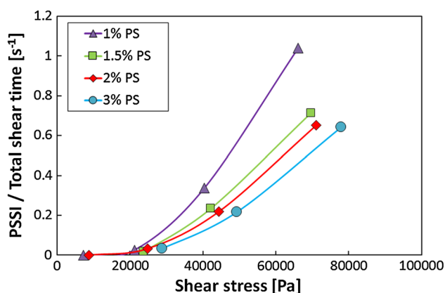
Fig. 11 Dependence of \text{PSSI}(10^6) rate of change on shear stress for four different concentrations of 100 k PS solution in DEHP at 80 °C after 20 cycles
