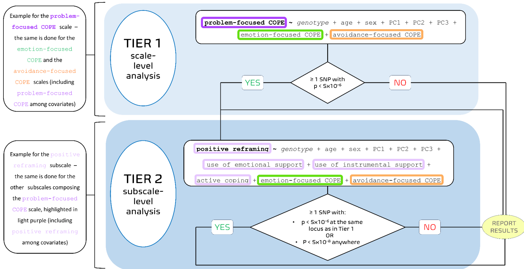
Figure 1 – analysis workflow applied on scores composed by multiple scales and/or subscales (i.e. Brief-COPE and RSA). In Tier-1, genome-wide association analysis is performed on each scale composing the score (e.g. problem-focused COPE, circled in dark purple), with other scales added as covariates (e.g. emotion-focused COPE and avoidance-focused COPE here, circled in green and orange, respectively). If significant genetic associations with a given scale are detected, genome-wide association analysis (Tier-2) is repeated on each subscale composing the scale in question (e.g. positive reframing, circled in light purple). Of note, while the main purpose of Tier-2 analysis is to investigate whether the Tier-1 association is driven by a specific subscale, additional associations not detected in the Tier-1 step may emerge. For this reason, in Tier-2 analysis two significance thresholds are applied: the suggestive significance threshold p < 5 \times 10^{-6} is used for SNPs at the same loci emerged in Tier-1, while the stricter genome-wide significance threshold ( p < 5 \times 10^{-8} ) is applied for associations concerning a specific subscale emerging in other areas of the genome.
