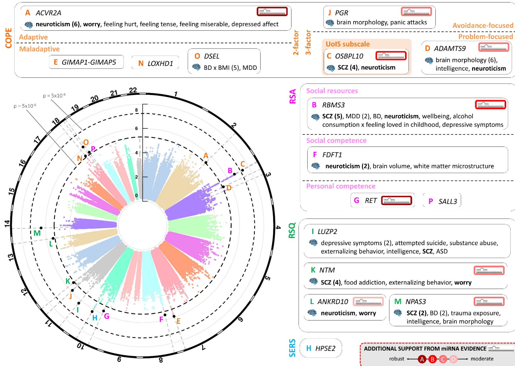
Figure 2 – Genome-wide association results across the 4 analyzed scores. The Manhattan plot shows, for each SNP, the most significant association across COPE, RSA, RSQ and SERS (orange, pink, green and blue association peaks, respectively, labeled with letters A to P starting from chromosome 1). The two black dashed lines represent significance thresholds applied in the analysis (corresponding to p = 5 \times 10^{-6} and 5 \times 10^{-8} ). The brain symbols denote previously published brain- or psychiatric-relevant associations for each gene, as from GWAS Catalog (see the Supplementary Notes for details on trait nomenclature), with the exception of the association between PGR and panic attacks (not listed in the catalog) 73 . In case of multiple associations for a given gene with the same trait/condition, the number of studies in which the association emerged is reported between brackets. Interactions between traits/conditions are indicated with an 'x'. The classification assigned to the additional supporting evidence from the miRNA target analysis, where available, is displayed by the color of the miRNA labels, as shown in the dashed box at the bottom. Traits/conditions tested in the genetic overlap analysis (i.e. those associated with at least 3 genes) are highlighted in bold. ASD=autism spectrum disorder, BD=bipolar disorder, BMI=body mass index, MDD=major depressive disorder, SCZ=schizophrenia.
