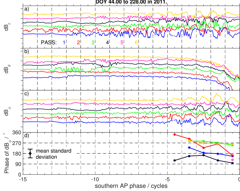
Figure 1. Perturbation magnetic field components as a function of southern AP phase from the 2011 inbound passes (interval C). (a)-(c) Show the r , \theta and \phi components of the perturbation magnetic respectively. (d) shows the phase of the first current sheet crossing (or approach when the current sheet was not crossed) of the normalised dB_\phi component along with the mean standard deviation of the determined phases. Data gaps or encounters of low confidence are omitted from the plot. The arrows highlight the phase-jumps to be discussed. The vertical dashed-lines indicate a unit cycle. The colors indicate the pass number in the selected time period.
