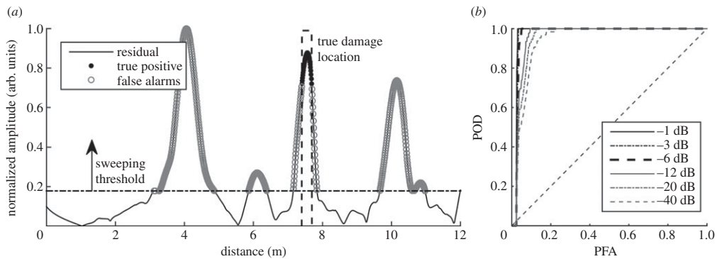
Figure 5. (a) Example residual signal obtained from a set of 100 measurements under temperature variation of 10^{\circ}\text{C} , over which damage grows from zero to 1% of the cross-sectional area. (b) Receiver operating characteristic curves computed from the residual in (a) with different tolerance level.
