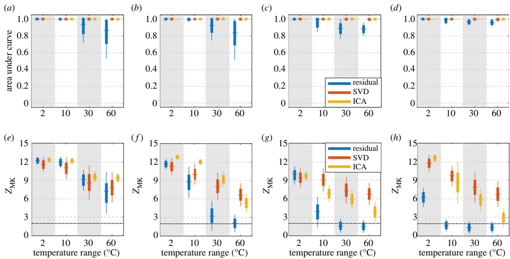
Figure 11. Box plots of AUC and Z_{MK} of detecting 1% damage growth over 100 measurements over different temperature ranges, where damage is added at four different locations in table 1. Plots (a,e) and (b,f) show results when damage is added at, respectively, 2.3 m and 11.3 m, away from structural features. Plots (c,g) and (d,h) show results when damage is added at, respectively, 6.2 m or 10.1 m, close to structural features. The dot-dash line in (e–h) shows the threshold of 1.96. (Online version in colour.)
