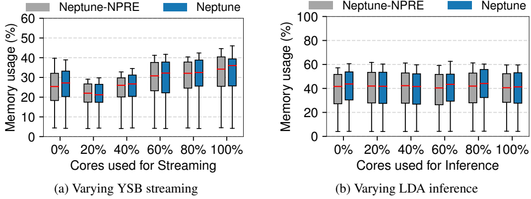
Figure 4.11 Memory impact of varying job demands
