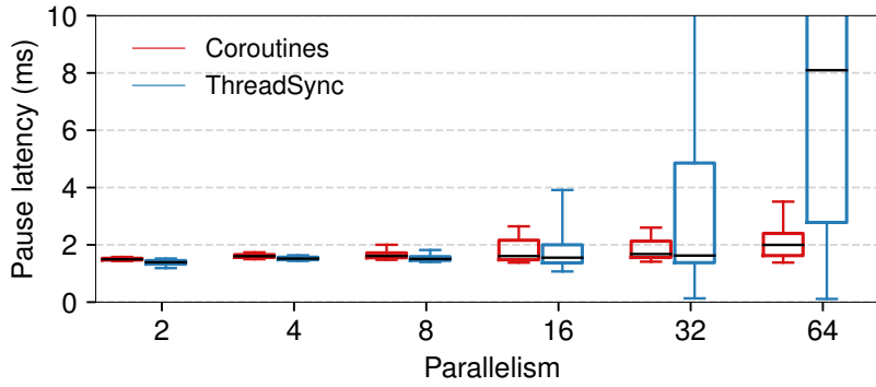
Figure 4.14 Latency of task suspension mechanisms
