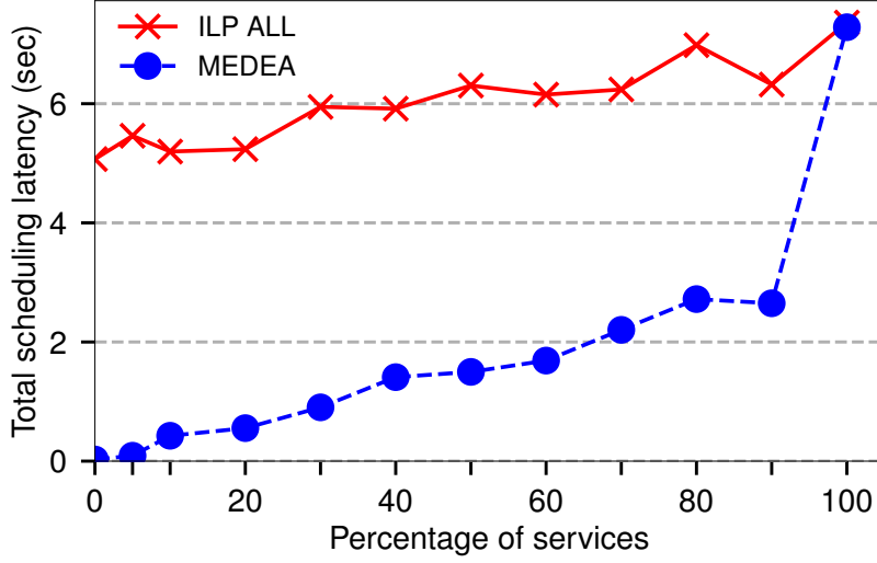
Figure 5.10 Two-scheduler benefit
