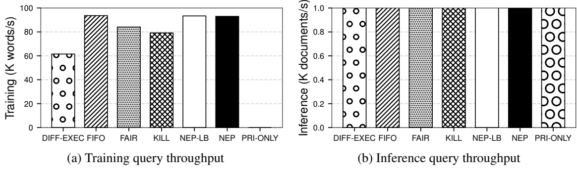
Figure 4.9 LDA NYTimes dataset (training + inference) throughput
