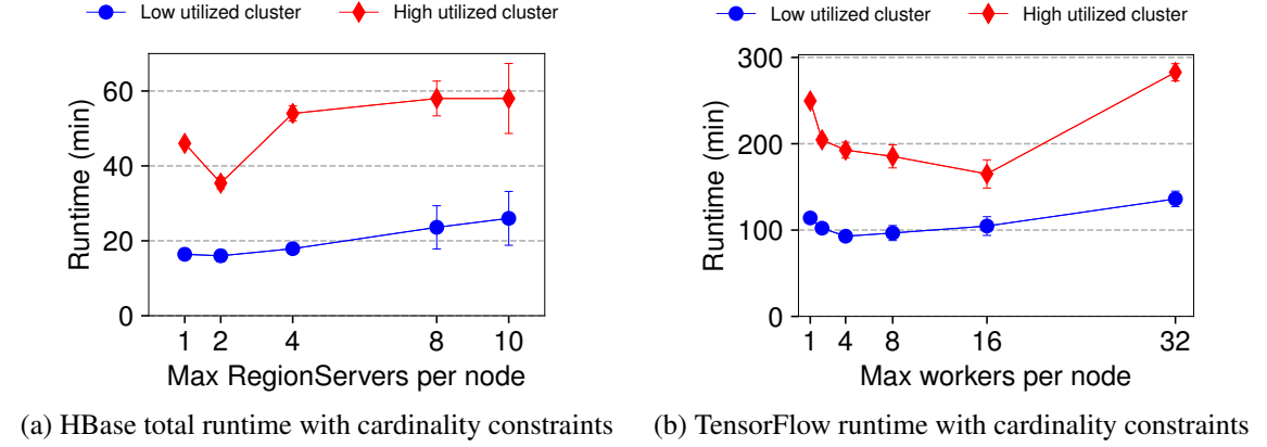
Figure 2.11 Impact of cardinality constraints on application performance
