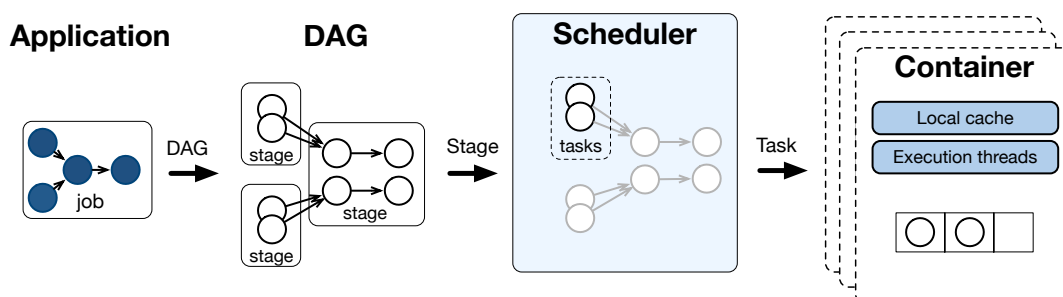
Figure 2.5 Execution overview of a dataflow application (Blue circles represent operators while white ones indicate different tasks.)
