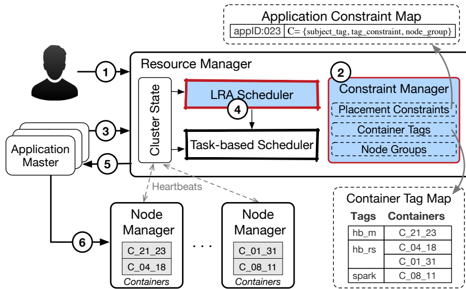
Figure 5.4 MEDEA architecture
