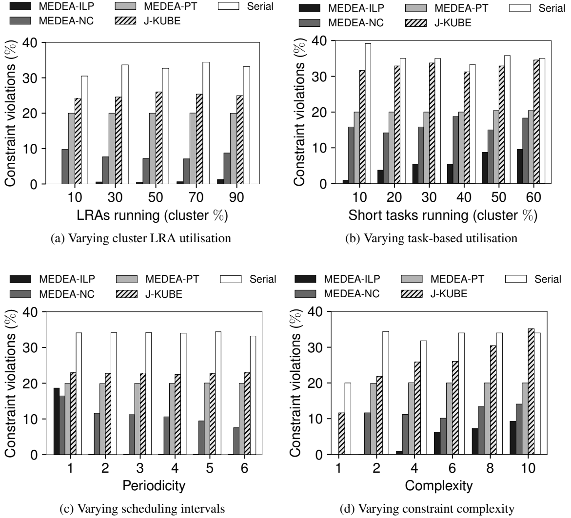
Figure 5.8 Constraint violations
