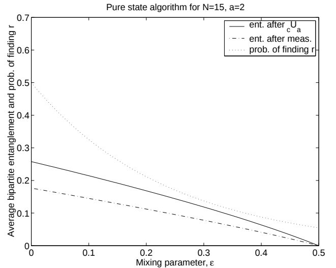
FIG. 11. Here we show, for the pure state algorithm of N = 15 and a = 2 , the entanglement averaged across all bipartite partitionings and all post -U_a and -measurement stages of the algorithm, vs. the mixing parameter, \epsilon , when the state of the control qubit is repeatedly prepared in the mixed state as in section VD. Also shown is the probability that the algorithm correctly finds the period r .
