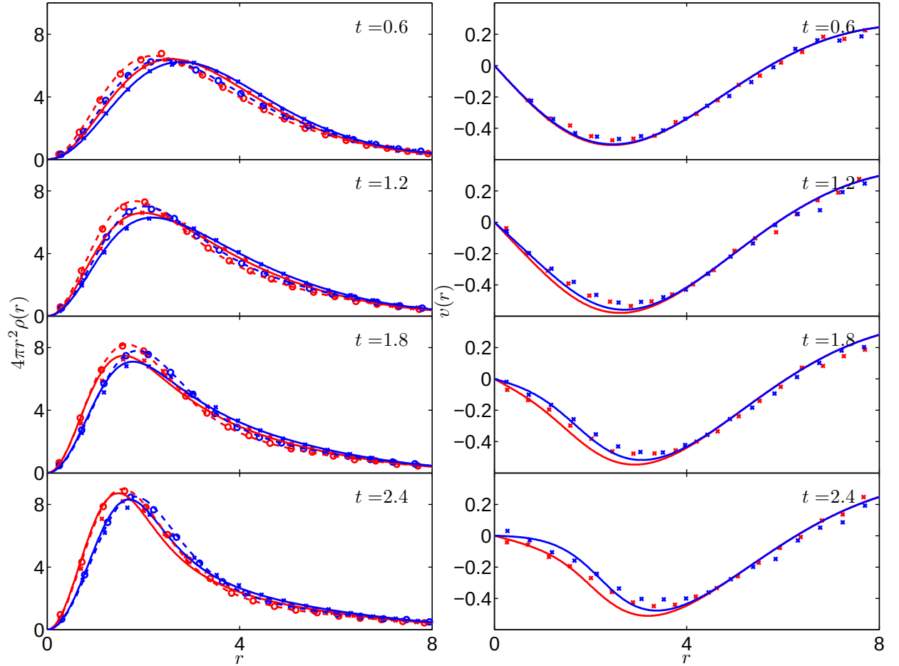
FIG. 10. Snapshots of radial particle distributions and velocities at various times for 25 particles of each species of soft particle. Species 1 in red and species 2 in blue. Lines show DDFT calculations, symbols stochastic dynamics for systems with (solid/crosses) and without (dashed/circles) inertia.
