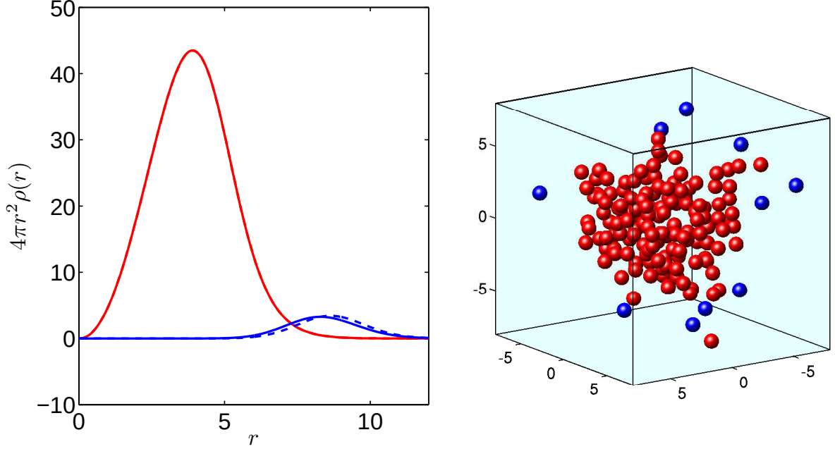
FIG. 7. Left plot shows the equilibrium particle distributions for N_1 = 150 particles of species 1 in red and N_2 = 10 particles of species 2 in blue. Solid lines correspond to r_2 = 7 and dashed to r_2 = 8 . Note that the curves for species 1 are indistinguishable. Right plot shows a typical equilibrium configuration for the same system. We show only the case r_2 = 7 ; the case for r_2 = 8 is similar and differences between particular realizations are uninformative.
