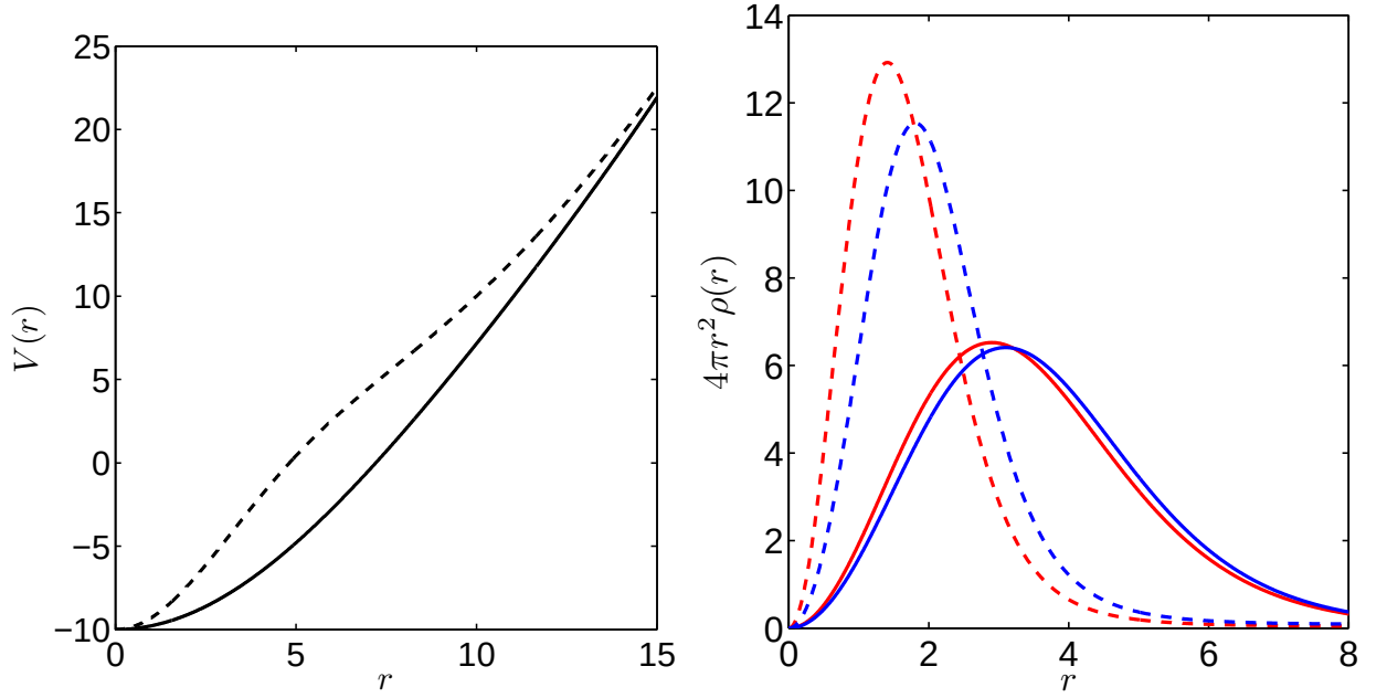
FIG. 9. Left plot shows the external potential for both species of soft particles at t = 0 (solid) and t > 0 (dashed). Right plot shows the initial (solid) and final (dashed) equilibrium particle distributions for the smaller species (red) and larger species (blue).
