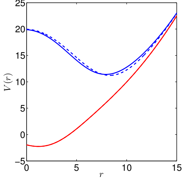
FIG. 6. External potentials (6) for species 1 (red) and (7) for species 2 (blue; solid for r_2(t) = 7 , dashed for r_2(t) = 8 ).
