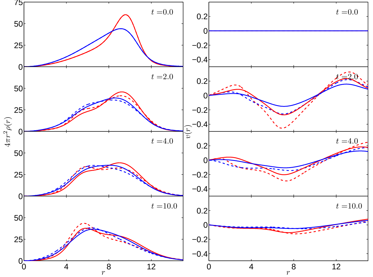
FIG. 5. Snapshots of radial particle distributions and velocities at various times for 250 particles of each species. Lines as in Fig. 3.
