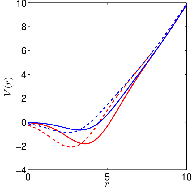
FIG. 2. External potentials for the two species (red, blue respectively) at t = 0 (solid lines) and t > 0 (dashed lines).
