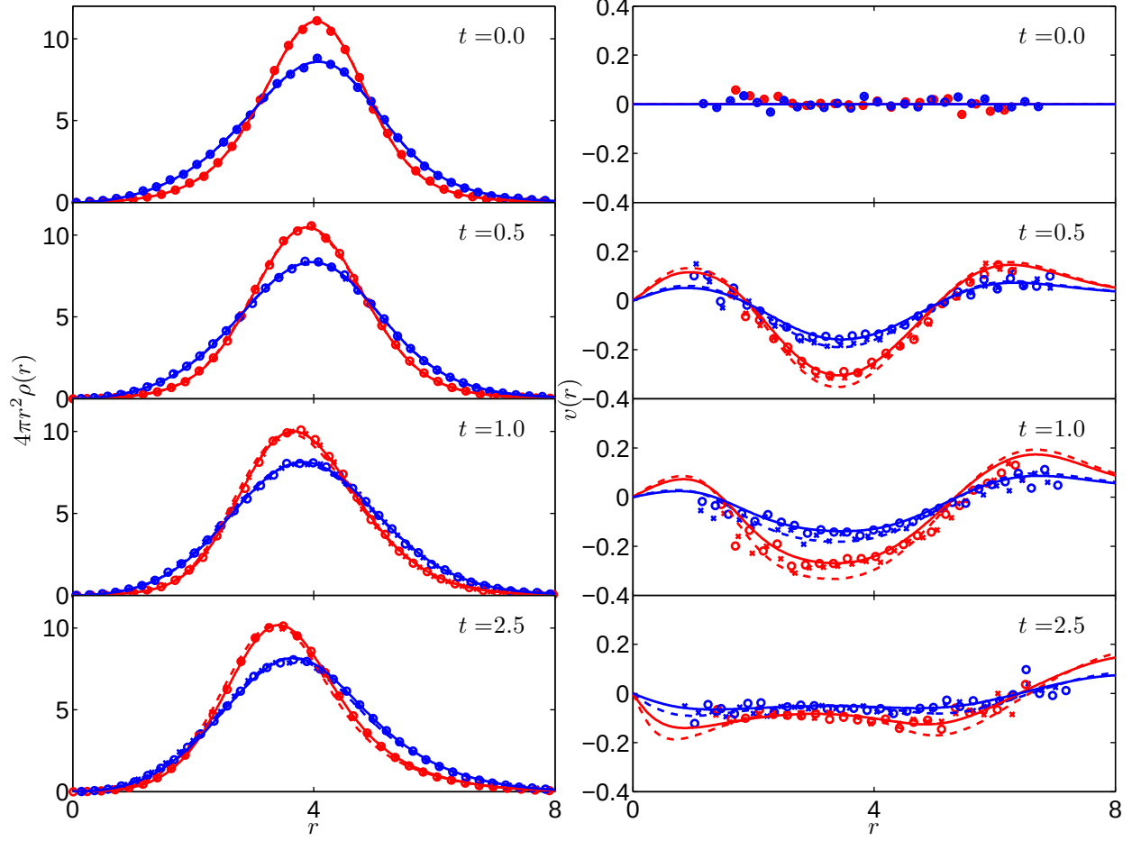
FIG. 3. Snapshots of radial particle distributions and velocities at various times for 25 particles of each species. Species 1 in red, species 2 in blue. Lines show DDFT calculations, symbols Langevin simulations for systems both with (solid/circles) and without (dashed/crosses) HI.
