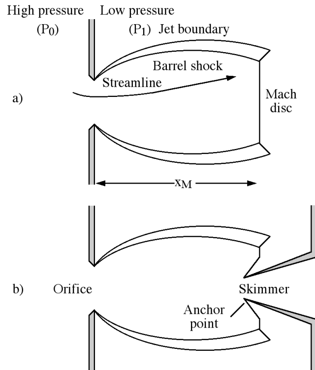
Fig. 1. (a) Structure of a supersonic free jet expansion. (b) Shock attachment to an ideal skimmer.
