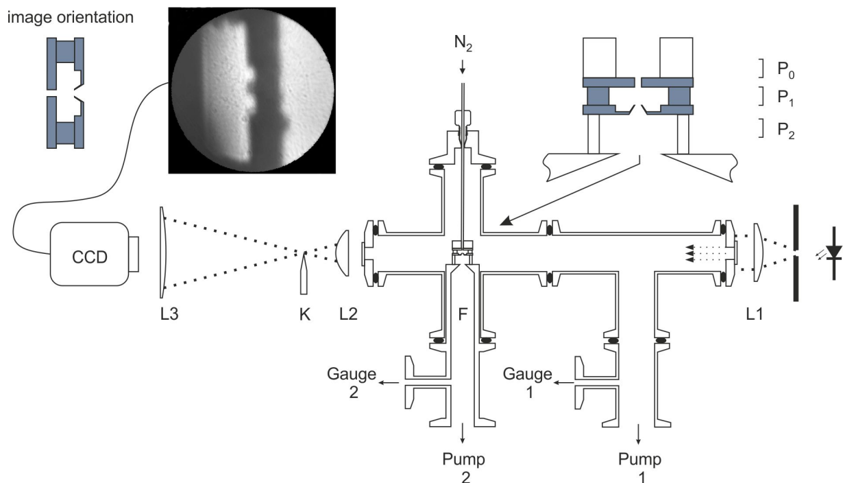
Fig. 5. Vacuum and schlieren imaging systems. Collimated light from a pinhole source passes through a two-stage vacuum bench. The skimmer assembly is mounted on a vacuum finger, F. Regions upstream and downstream of the skimmer are illuminated. The image is magnified by lenses L2 and L3. A knife edge, K, at the common focus of L2 and L3 partially blocks the light beam and generates a schlieren image.
