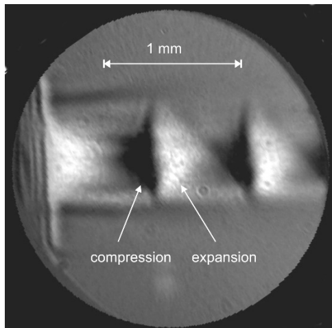
Fig. 12. Schlieren image of a supersonic jet from an 800 \mu\text{m} aperture at P_0/P_1 = 2.75 . Regions of expansion are bright and regions of compression are dark.
