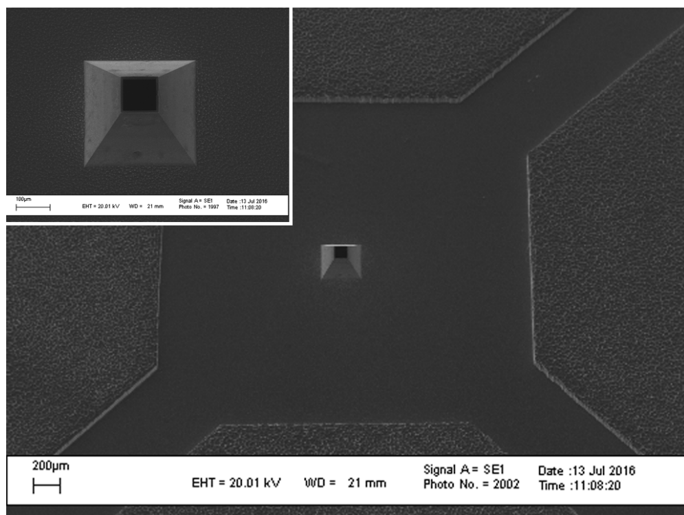
Fig. 4. SEM images of a microfabricated Ni skimmer with a 100 x 100 μm aperture.
