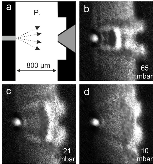
Fig. 7. Schlieren imaging of jets interacting with a skimmer. The inlet and skimmer positions are indicated in (a) and images corresponding P_1 = 65 , 21, and 10 mbar are shown in (b)-(d). P_0 = 3 bar. The skimmer is unable to fully penetrate the shock structure.
