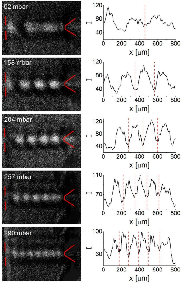
Fig. 11. Schlieren images corresponding to the peak positions in in Fig. 10(a). Plots of intensity (I) against position along the beam centreline (x) are shown on the right.
