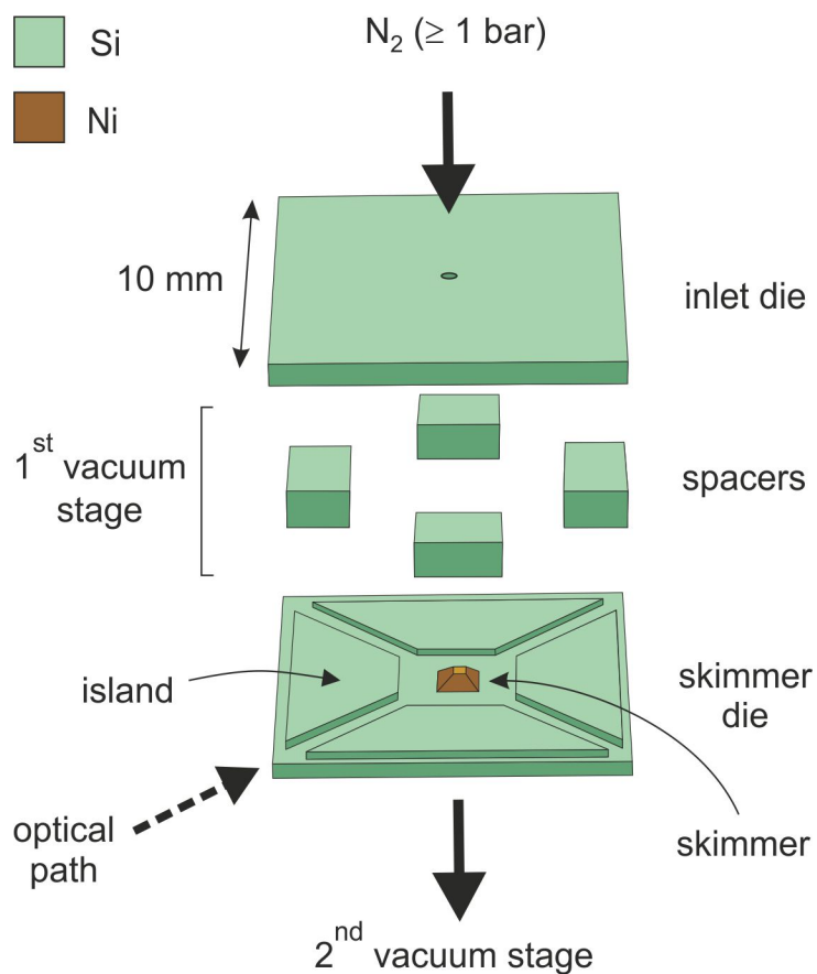
Fig. 2. Exploded view of the skimmer assembly. The spacers are 800 \mu\text{m} deep. For clarity, the skimmer has been drawn on an exaggerated scale. Nitrogen passes through the inlet capillary and expands into the first vacuum stage. The resulting supersonic jet interacts with the skimmer and a portion is transmitted into the second vacuum stage.
