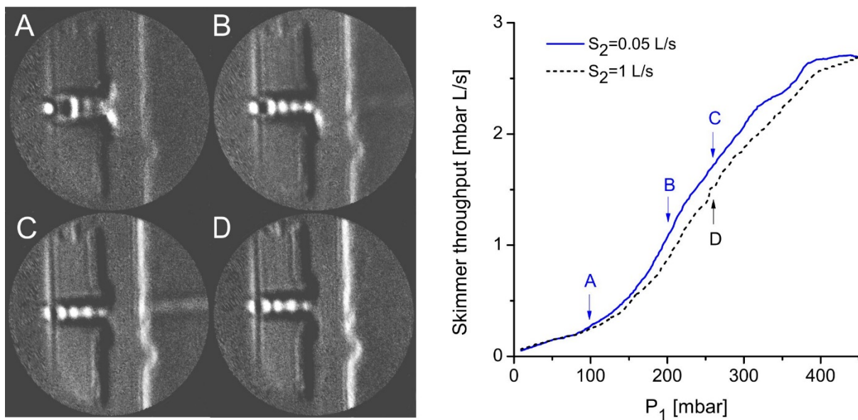
Fig. 9. Plots of skimmer throughput against first stage pressure are shown on the right for two different second stage pumping speeds ( S_2 ). Schlieren images corresponding to the indicated points on the curves are shown on the left. The jet formed in the first stage narrows as P_1 increases (A and B) and eventually passes through the skimmer where a second expansion yields a collimated beam (C). If the background pressure in the second stage is reduced, the same gas flow passes through the skimmer but a beam cannot be seen (D).
