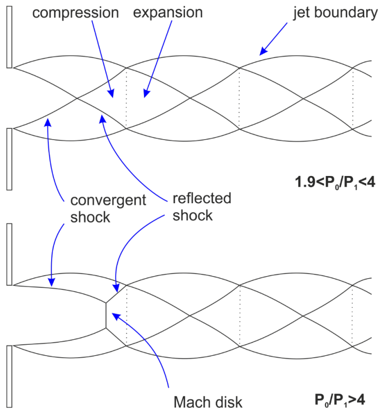
Fig. 8. Schematic representations of extended supersonic jets exhibiting multiple shock cells.
