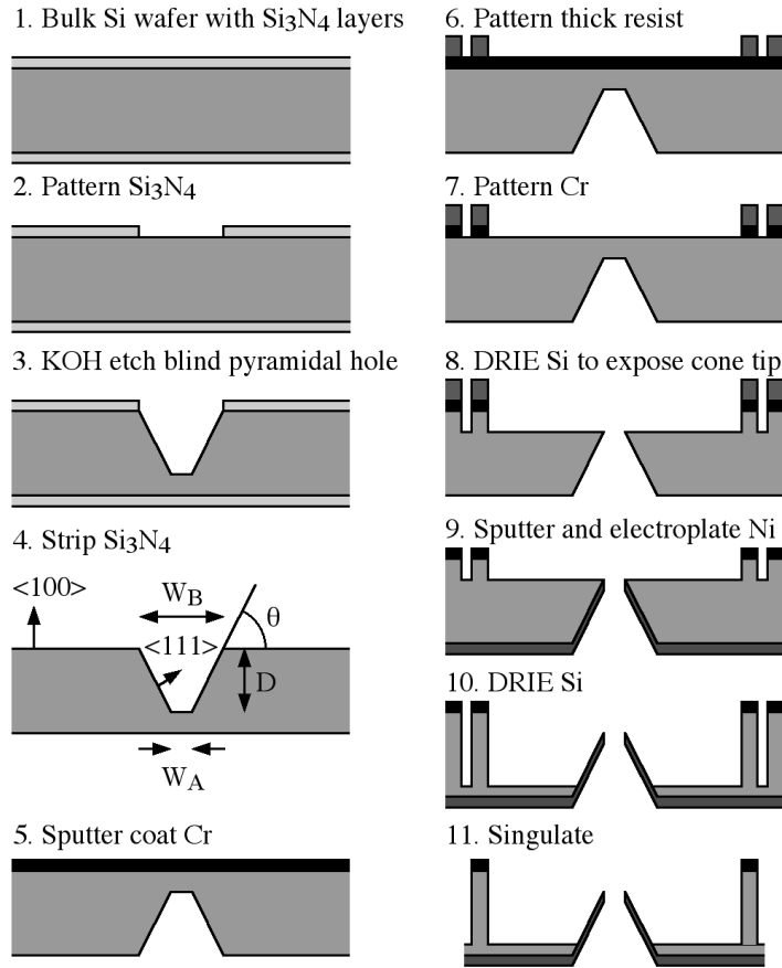
Fig. 3. Skimmer microfabrication process. Pyramidal holes were produced in a (100) silicon wafer by anisotropic crystal etching (steps 1-8). After sputter deposition of nickel on the internal walls (step 9), excess Si was removed from the reverse side of the wafer (step 10), leaving free-standing Ni skimmers supported on a Si substrate.
