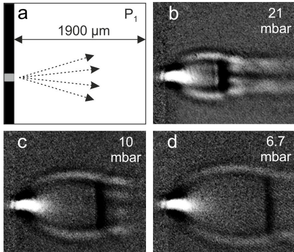
Fig. 6. Schlieren images of free jets. The inlet position and scale are indicated in (a) and images corresponding P_1 = 21 , 10 and 6.7 mbar are shown in (b)-(d). P_0 = 3 bar. The Mach disc (dark vertical band) grows thicker as the jet shrinks.
