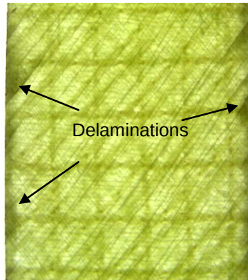
Figure 10. The interlaminar delaminations observed at the free edges of the test specimen during fatigue testing of GFRP composite based upon a neat epoxy matrix. \sigma_{max} = 150 MPa and R = 0.1
