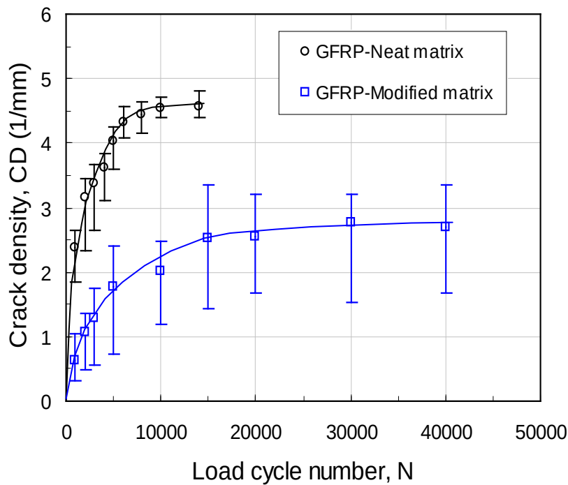
Figure 9. The variation of \pm 45^\circ crack density with fatigue cycles in GFRP composites based upon a neat or a rubber-modified matrix.
