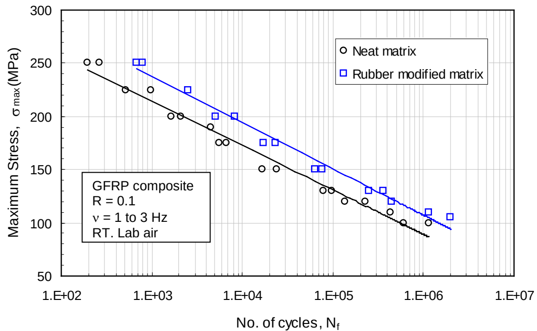
Figure 6. The stress versus life (S-N) curve of GFRP composites with neat and 9 wt.% rubber-modified epoxy matrices.
