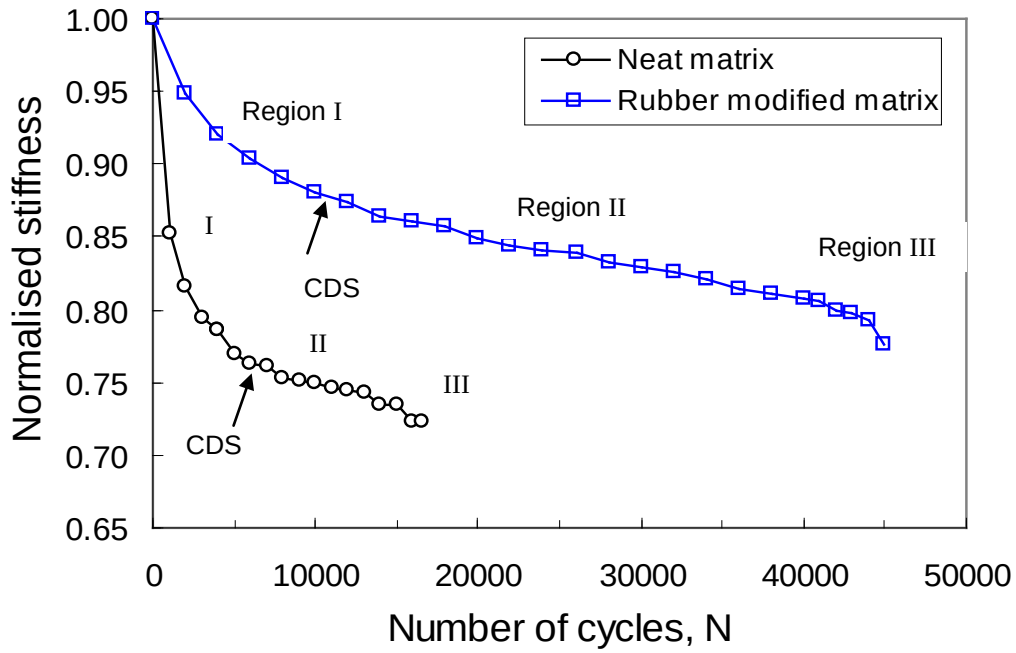
Figure 7. The normalised stiffness variation during fatigue determined in GFRP composite with neat and rubber-modified epoxy matrices. \sigma_{max} = 150 \text{ MPa} , R = 0.1
