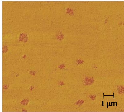
Figure 1. The tapping mode atomic force microscope (AFM) phase image of the 9 wt.% rubber-modified bulk epoxy polymer.
