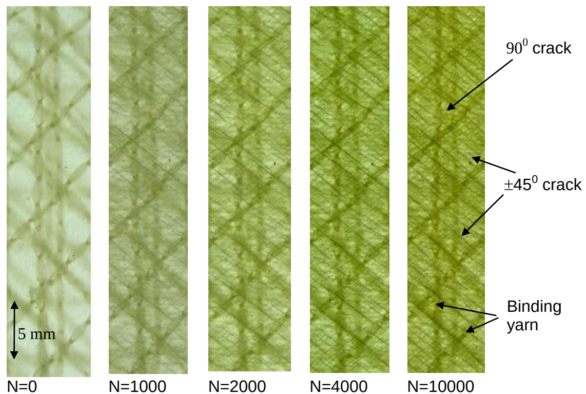
Figure 3. The transmitted light photographic images of the GFRP composite with a neat matrix showing the sequence of matrix crack development with increasing number of cycles (N) under fatigue loading.
