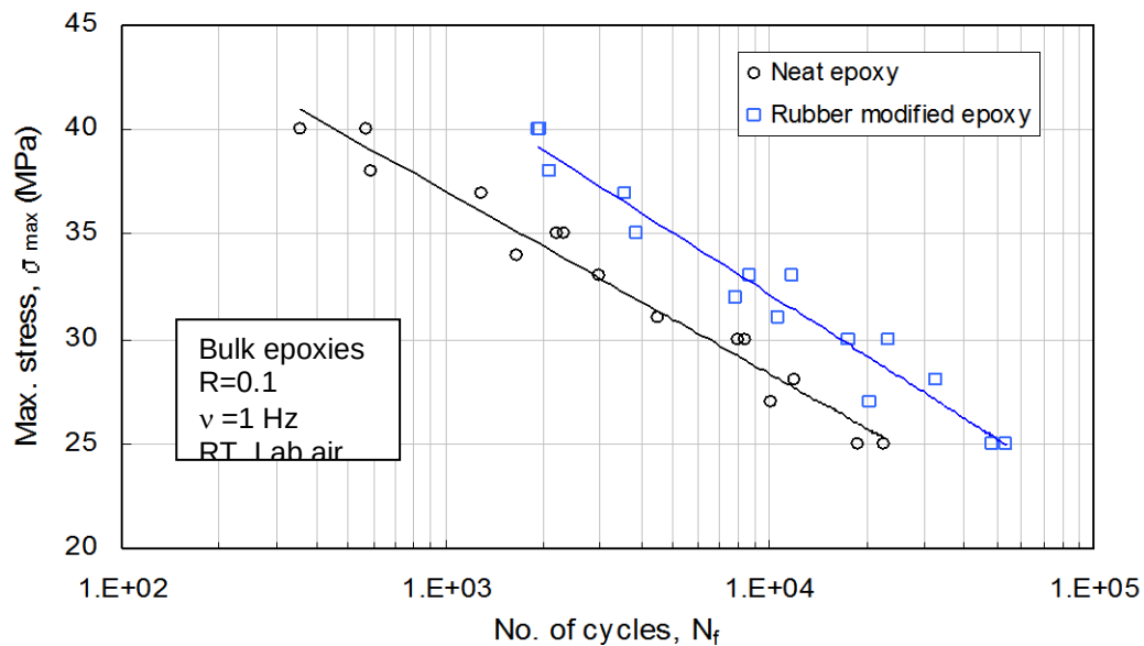
Figure 4. The stress versus lifetime (S-N) curves of the neat and 9 wt.% rubber-modified bulk epoxy polymers.
