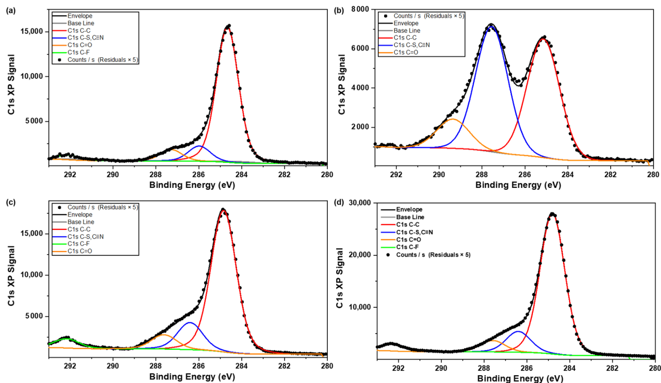
Figure 7. C1s spectra of (a) facet 1, (b) facet 2, and (c) facet 3 of Odanacatib crystal, and (d) C1s spectra of a tablet of Sample A1.
