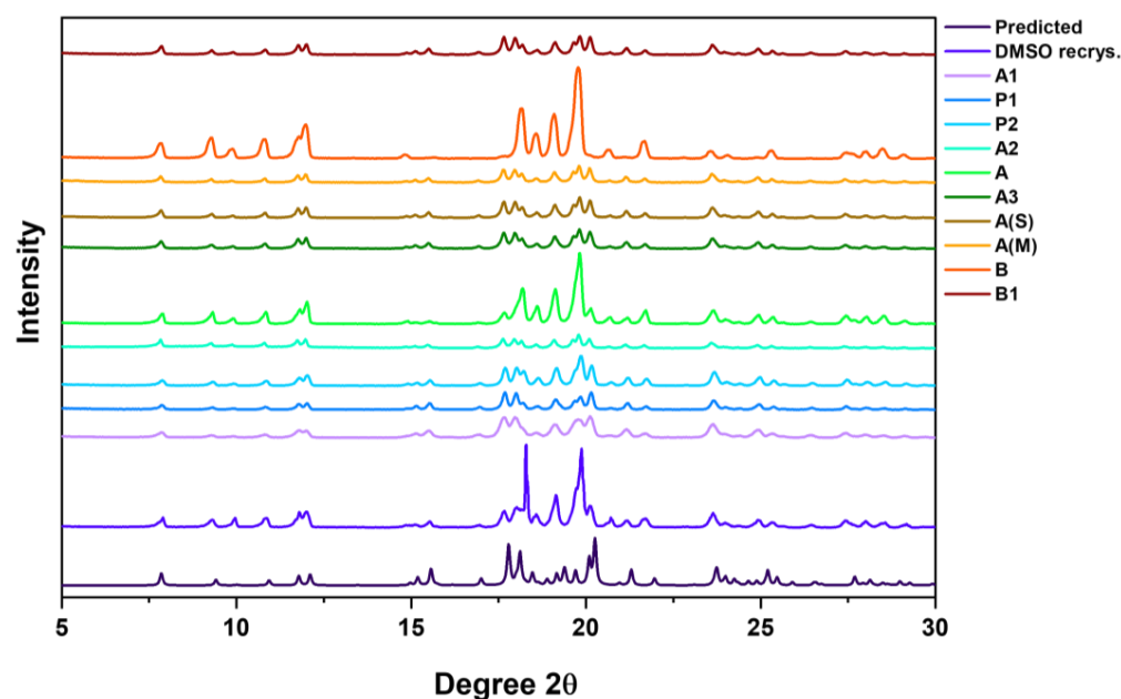
Figure 5. X-ray diffraction patterns of all the as-received samples and the crystals grown using DMSO, compared against the predicted powder pattern.
