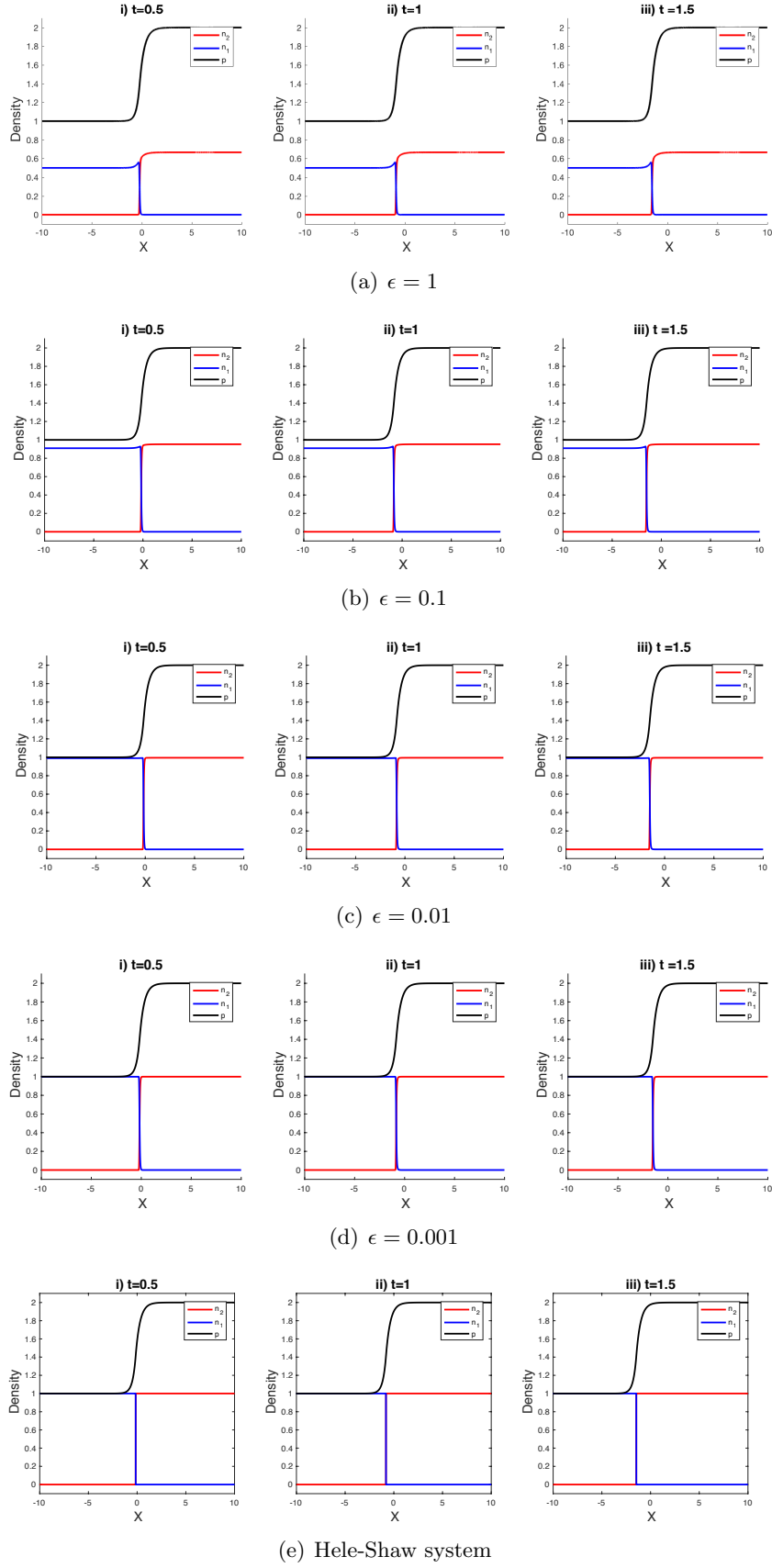
Figure 2: Densities n_1 (blue), n_2 (red) and pressure p as functions of position x at different times: (i) t = 0.5 , (ii) t = 1 , (iii) t = 1.5 ; and for different values of \epsilon : (a) \epsilon = 1 , (b) \epsilon = 0.1 , (c) \epsilon = 0.01 , (d) \epsilon = 0.001 , (e) Hele-Shaw system.
