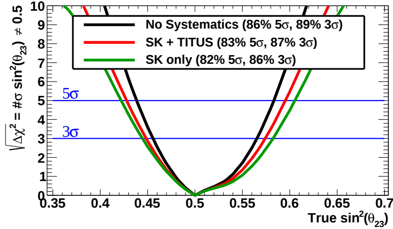
Figure 37: Significance to exclude \sin^2(\theta_{23}) = 0.5 as a function of \sin^2(\theta_{23}) with the combinations of samples and constraints given in the legend and the fraction of \sin^2(\theta_{23}) Super-K will be able to exclude \sin^2(\theta_{23}) = 0.5 (at 5\sigma and 3\sigma ). For the studies, the true values of oscillation parameters to generate the data sets were taken from Table 19. Sensitivity is for the case of normal hierarchy and assuming it is known. Due to a non zero \sin^2(\theta_{13}) , the disappearance spectra have a symmetry around \sin^2(\theta_{23}) = 0.511 , which is the cause of the flat feature in the sensitivity between 0.5 and 0.511.
