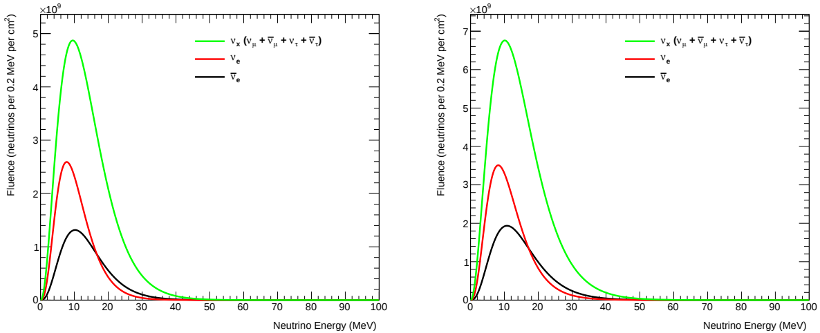
Figure 40: Total predicted neutrino flux for 11.2M_{\odot} (left) and 27.0M_{\odot} (right) progenitor mass stars at a distance of 10 kpc.
