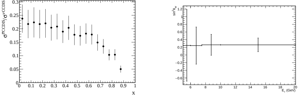
Figure 39: Left: Ratio of the \bar{\nu}_\mu CCDIS to \nu_\mu CCDIS cross sections as a function of x with statistical and systematic errors given in the text. Right: Measurement of \sin^2 \theta_W as a function of neutrino energy starting from 5 GeV.
