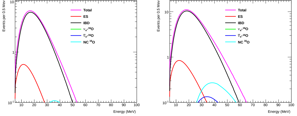
Figure 41: Predicted neutrino interaction spectrum, broken down by interaction type, for 11.2M_{\odot} (left) and 27.0M_{\odot} (right) progenitor mass stars at a distance of 10 kpc in the TITUS detector. Legend defined in Table 27.
