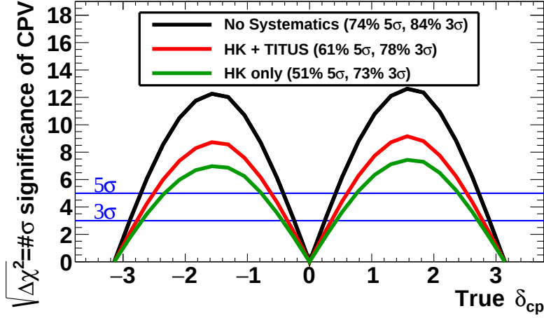
Figure 31: Significance to measure CP violation as a function of \delta_{CP} with Hyper-K only, TITUS (Gd-doped) and Hyper-K (not Gd-doped), and Hyper-K without considering sources of systematic uncertainty. For the studies, the true values of oscillation parameters to generate the data sets were taken from Table 19 but with \sin^2(\theta_{23}) = 0.5 . The fraction of \delta_{CP} for which CP violation will be measured at 5\sigma and 3\sigma is given in the legend. The sensitivity is for the case of normal hierarchy and assuming it is known.
