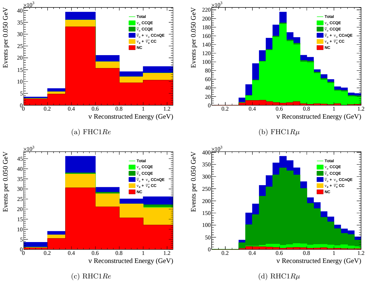
Figure 28: Predicted neutron tagged TITUS spectra.
