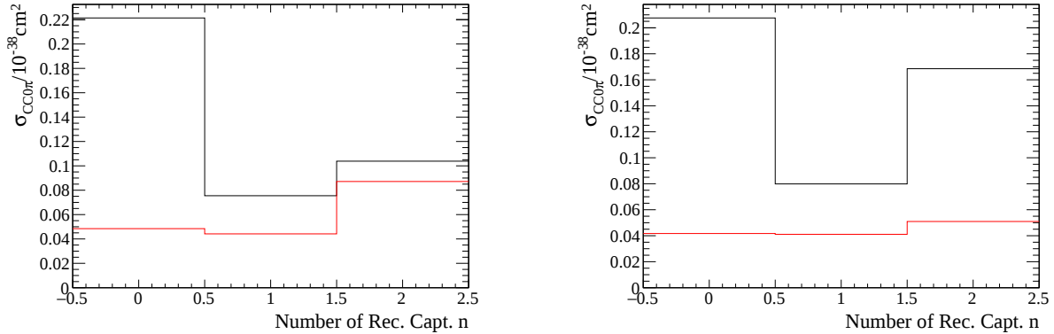
Figure 38: True flux-integrated cross section as a function of neutron multiplicity for \nu_\mu (black) and \bar{\nu}_\mu (red) \text{CC}0\pi using the NEUT generator. The \nu -mode ( \bar{\nu} -mode) measurement is on the left(right). Statistical and systematic uncertainties have not been considered. The last bin is integrated for all events with neutron captures greater than 1.
