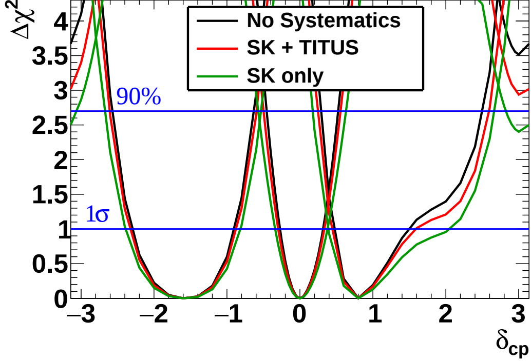
Figure 36: Significance to measure CP violation as a function of \delta_{cp} with T2K phase-2 only, TITUS and T2K phase-2, and T2K phase-2 without considering sources of systematic uncertainty for 3 Asimov fits to \delta_{cp} assuming T2K phase-2 statistics. The sensitivity is for the case of normal hierarchy and assuming it is known. The uncertainty on \delta_{cp} is given in Table 25 and the other oscillation parameters are given in Table 19.
