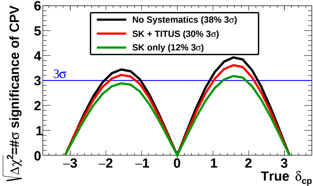
Figure 35: Significance to measure CP violation as a function of \delta_{cp} with T2K phase-2 only, TITUS and T2K phase-2, and T2K phase-2 without considering sources of systematic uncertainty assuming T2K phase-2 statistics. For the studies, the true values of oscillation parameters to generate the data sets were taken from Table 19 but with \sin^2(\theta_{23}) = 0.5 . The fraction of \delta_{cp} for which CP violation will be measured at 5\sigma and 3\sigma is given in the legend. The sensitivity is for the case of normal hierarchy and assuming it is known.
