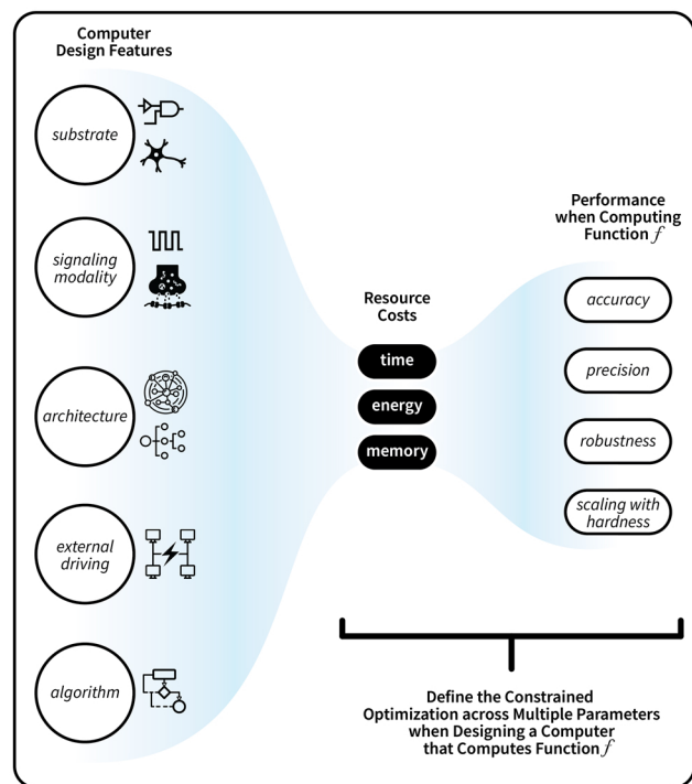
Fig. 1. The mapping between the design features of a computer and its performance when computing a function is mediated by its resource costs.
