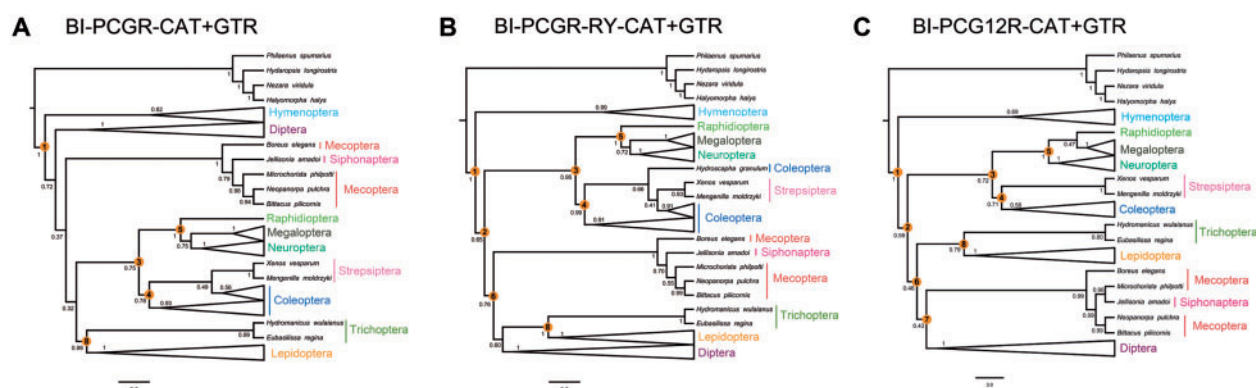
Fig. 5. —Holometabolan phylogenies inferred from the combined protein-coding genes and rRNA genes using PhyloBayes with the CAT + GTR model. (A) Bayesian tree from the data set PCGR under the CAT + GTR model. (B) Bayesian tree from the data set PCGR-RY under the CAT + GTR model. (C) Bayesian tree from the data set PCG12R under the CAT + GTR model. We show a schematic version of the Bayesian trees with some lineages collapsed for clarity. Supports at nodes are Bayesian posterior probabilities. Orange circles with number indicate recovered uncontroversial relationships in figure 1.
